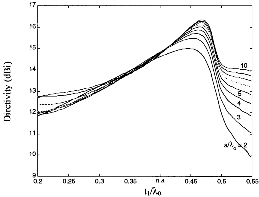
Fig. 23: Variation in directivity as a function of t_1/\lambda_0 for various values of a/\lambda_0 from 2 to 10, while t_1/\lambda_2 = 0.25 .
