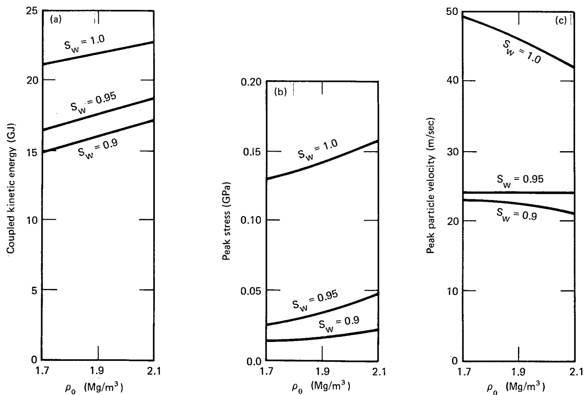
Fig. 54. Total effect of \rho_0 on kinetic energy coupling and ground motion.
