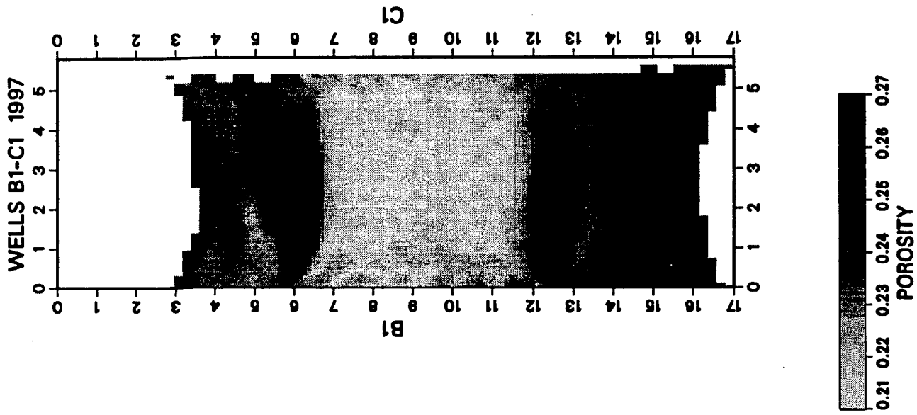
Figure 5. Porosity tomogram using 100 MHz radar antennas.
