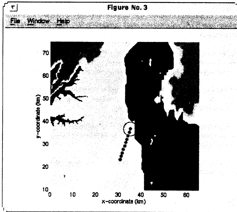
Figure 19: Tracking Window
