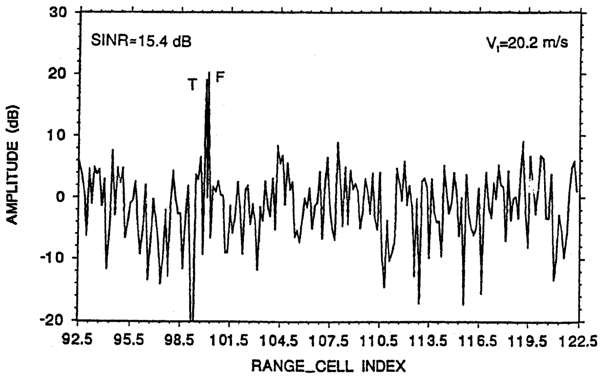
Figure 3-18: Large Degree of Freedom STAP; Jamming and Highway Traffic
