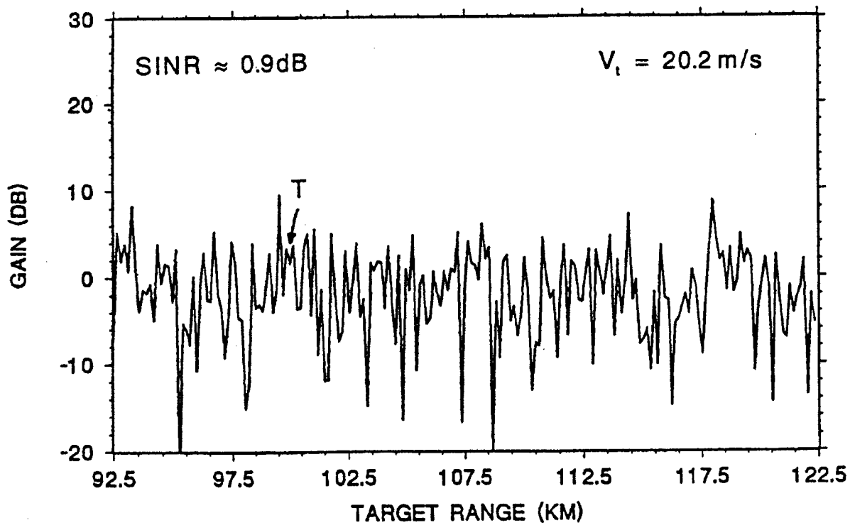
Figure 3-14: STAP and Notching; Highway Traffic and Jamming at 5.2 degrees
