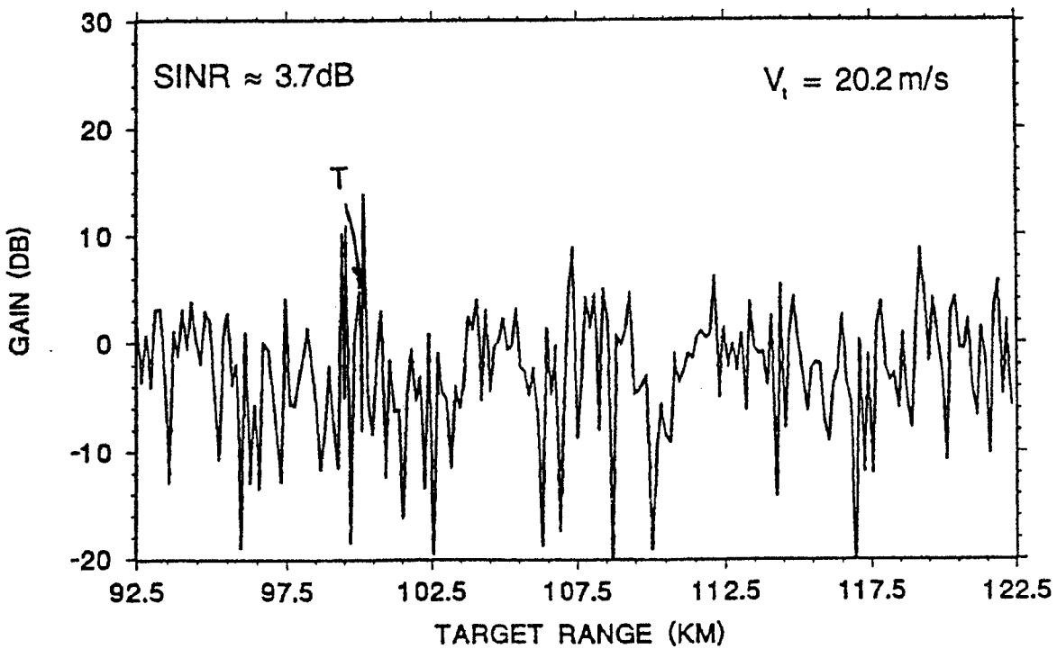
Figure 3-11: STAP Only; Highway Traffic but no Jamming
