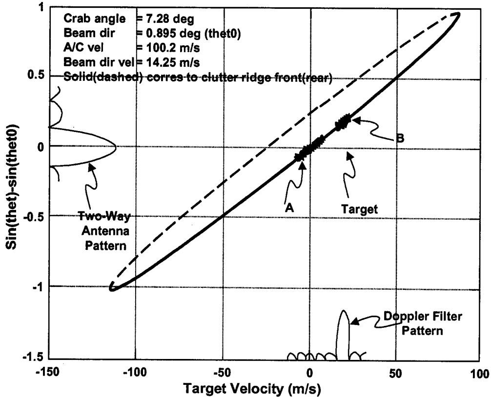
Figure 1-11: Angle/Doppler Diagram
