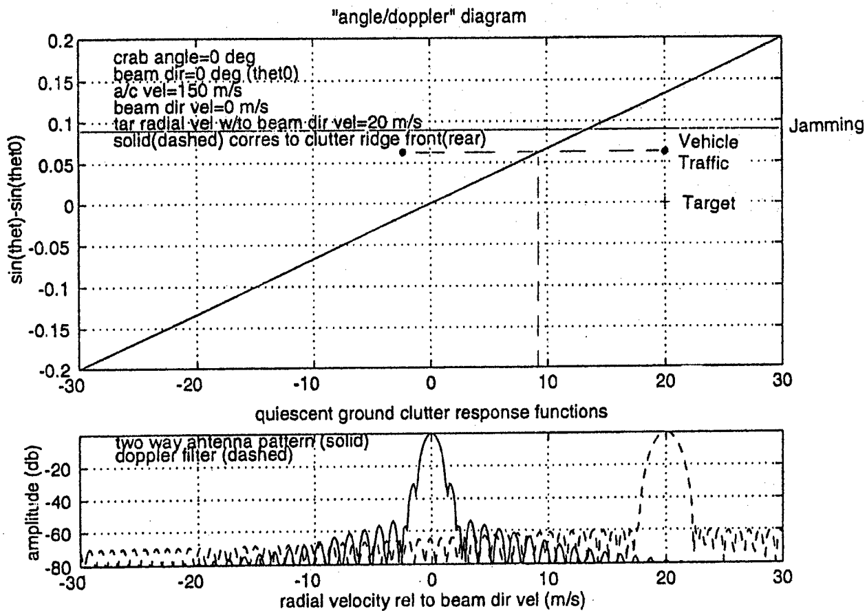
Figure 3-7: Angle/Doppler Diagram
