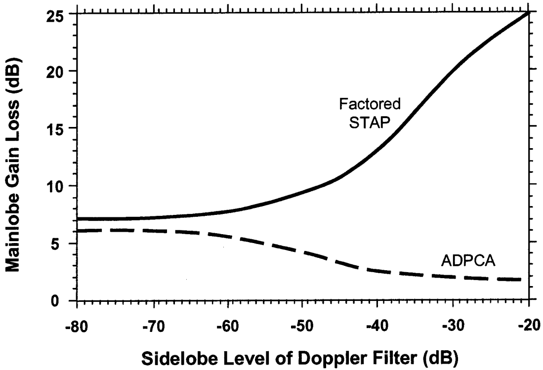
Figure 1-12: STAP Method Comparison
