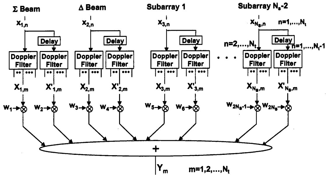
Figure 1-7: SLC Post-Doppler STAP
