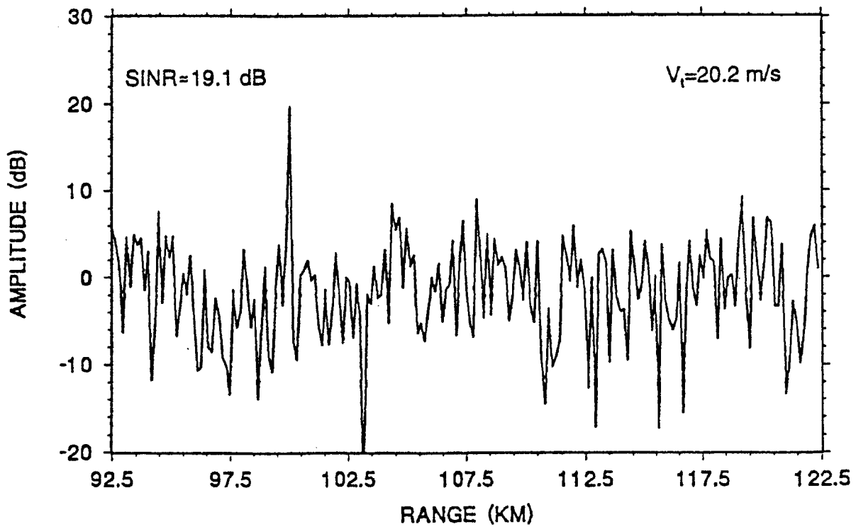
Figure 3-17: Large Degree of Freedom STAP; Jamming but no Highway Traffic
