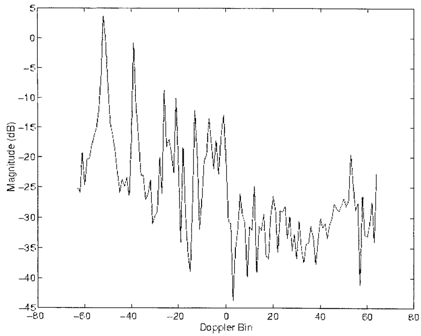
Figure 22: Location of the MTS tones using a non-adaptive beamformer
