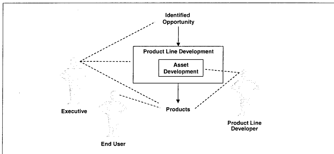
Figure 2: Stakeholder Views
