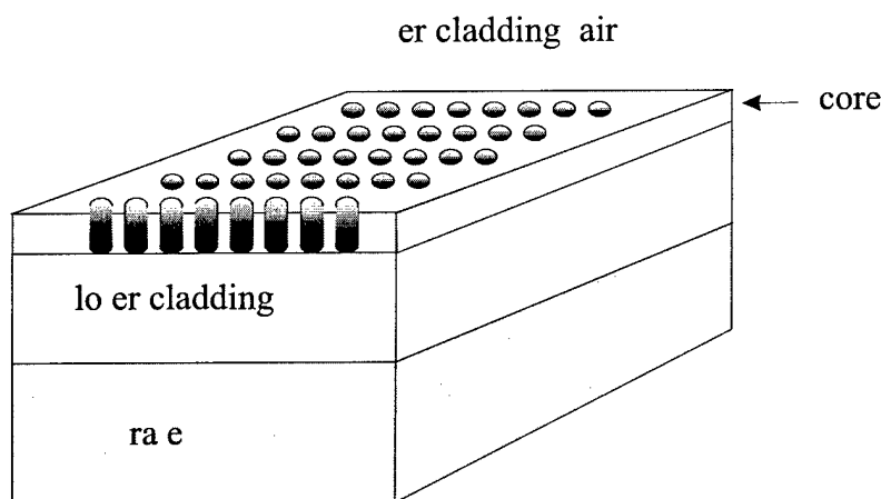
Figure 2.9: Schematic diagram of a textured planar waveguide.
