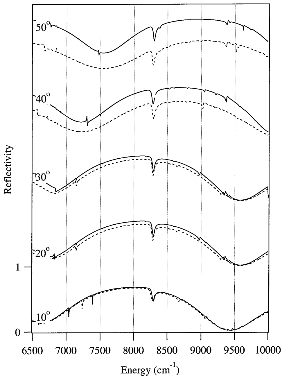
Figure 5.47: Simulated specular reflectivity for a textured planar waveguide with a triangular lattice, exhibiting a dispersion-free defect band in the first order pseudo-gap, shown for angles of incidence of 10^\circ , 20^\circ , 30^\circ , 40^\circ and 50^\circ along the M direction. The solid lines represent s-polarized and the dashed lines represent p-polarized reflectivity spectra.
