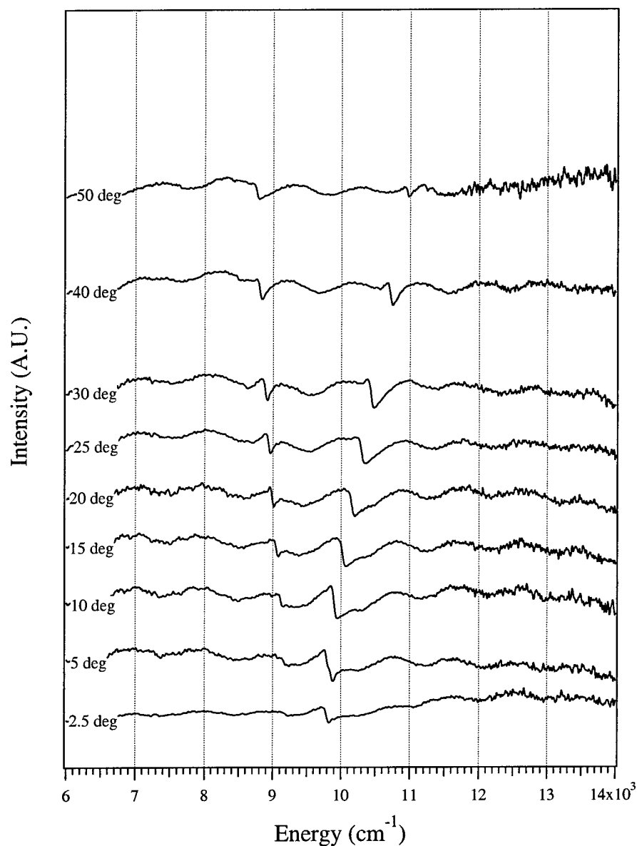
Figure 5.44: P-polarized specular reflectivity data for T-7 taken in the M direction.
