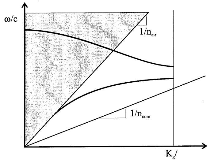
Figure 2.2: Schematic of 1D zone-folding.
