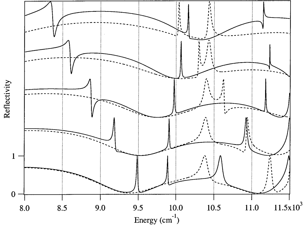
Figure 5.23: Simulation of specular reflectivity for the 150 nm thick textured planar waveguide with the square lattice discussed in the text. The spectra correspond to angles of incidence of 10^\circ , 20^\circ , 30^\circ , 40^\circ and 50^\circ from the bottom up. The solid lines represent s-polarized simulations. The dashed lines represent p-polarized simulations.
