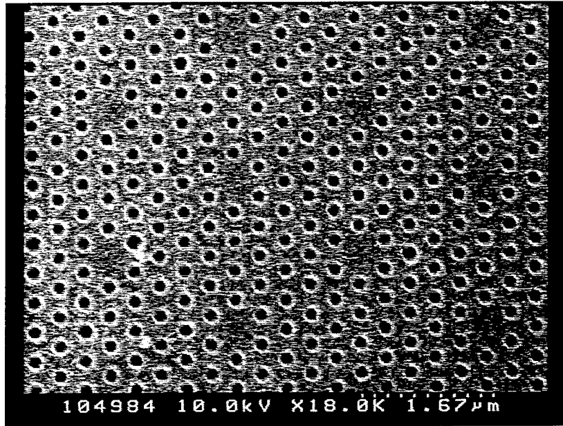
Figure 5.31: Scanning electron micrograph of T-5 sample: a planar waveguide textured with a triangular base lattice, with a defect superlattice 5x the period of the base lattice. This waveguide was fabricated using ASU721, and the pitch of the lattice is 600 nm.
