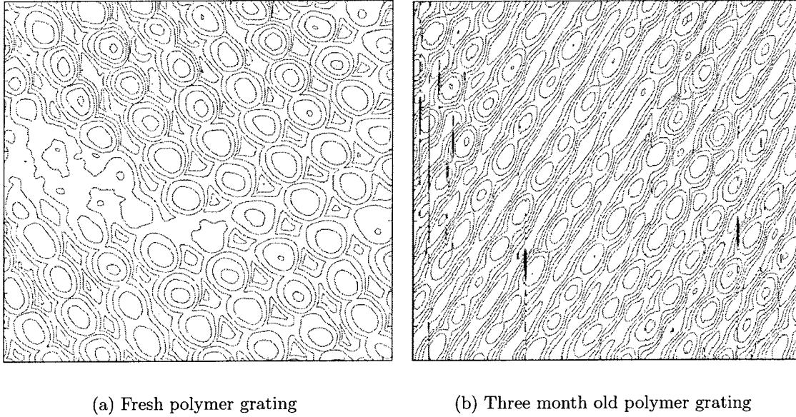
Figure 5.21: Atomic force micrographs of two polymer square lattice gratings. The sample shown in Figure (a) was recently manufactured, while the one shown in Figure (b) was exposed to ambient light for approximately 3 months. Each contour line is 50 nm.
