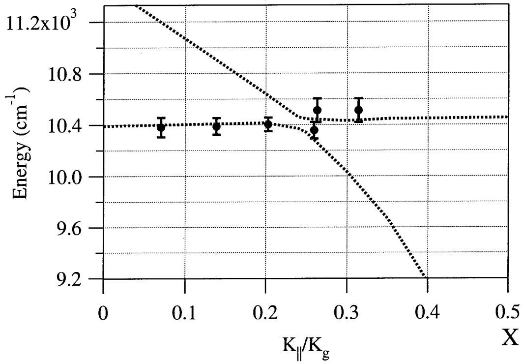
Figure 5.28: Dispersion diagram of the flat p-polarized bands showing simulation and data. Dotted line represents the simulation for the base lattice. Large dots represent central location of the mode derived experimentally via the -K_g^D diffracted order. Error bars on data points represent the width of gaussian fits to mode profile from diffraction data.
