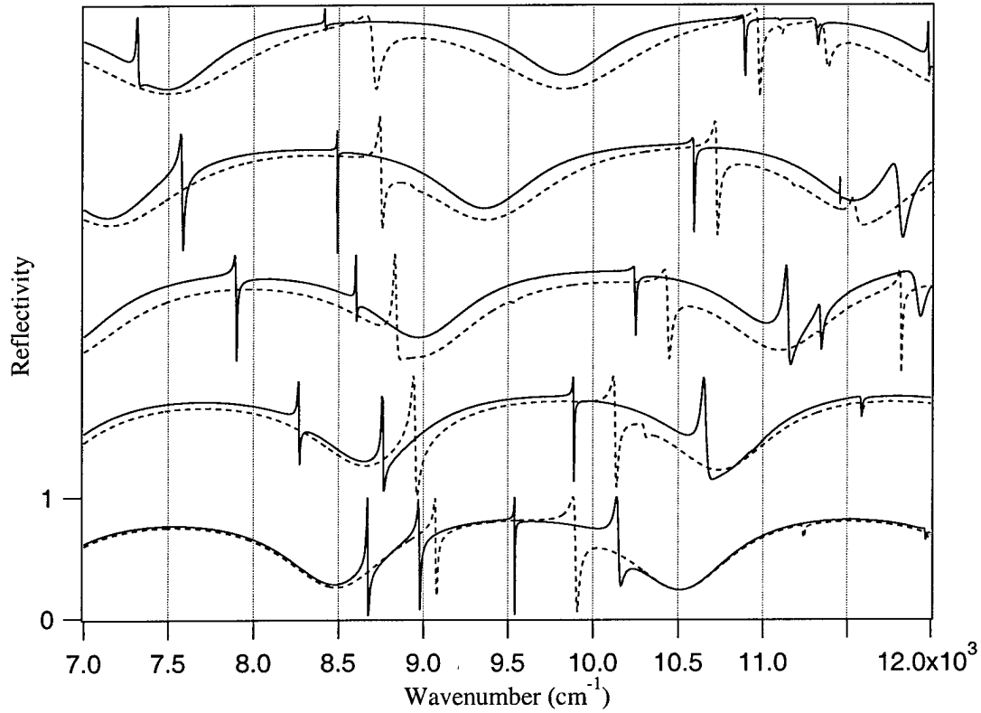
Figure 5.11: Simulated spectra for the M direction of a triangular lattice sample with 1600 nm of oxide, i.e. thick oxide layer. The spectra are for angles of incidence of 10°, 20°, 30°, 40°, and 50° from the bottom up. Solid lines represent s-polarization; dashed lines represent p-polarization.
