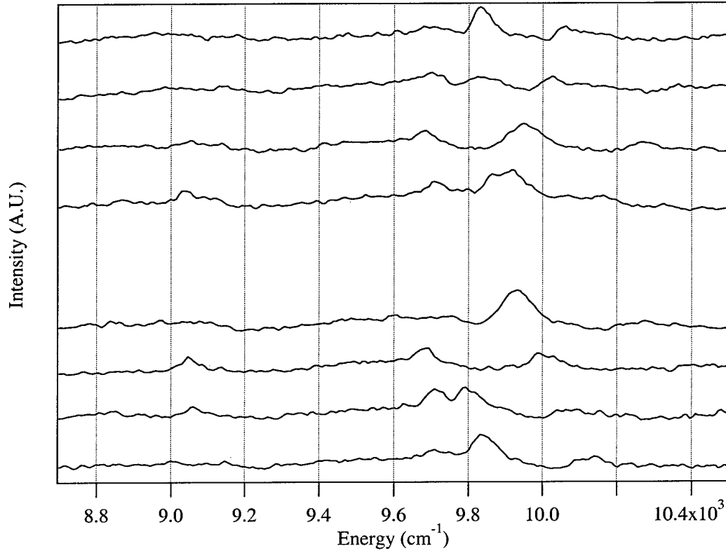
Figure 5.32: Unpolarized -K_g^D diffraction data for T-5. Spectra from the bottom up are for incident angles of 2^\circ , 4^\circ , 6^\circ , 8^\circ , 14^\circ , 16^\circ , 18^\circ , and 20^\circ .
