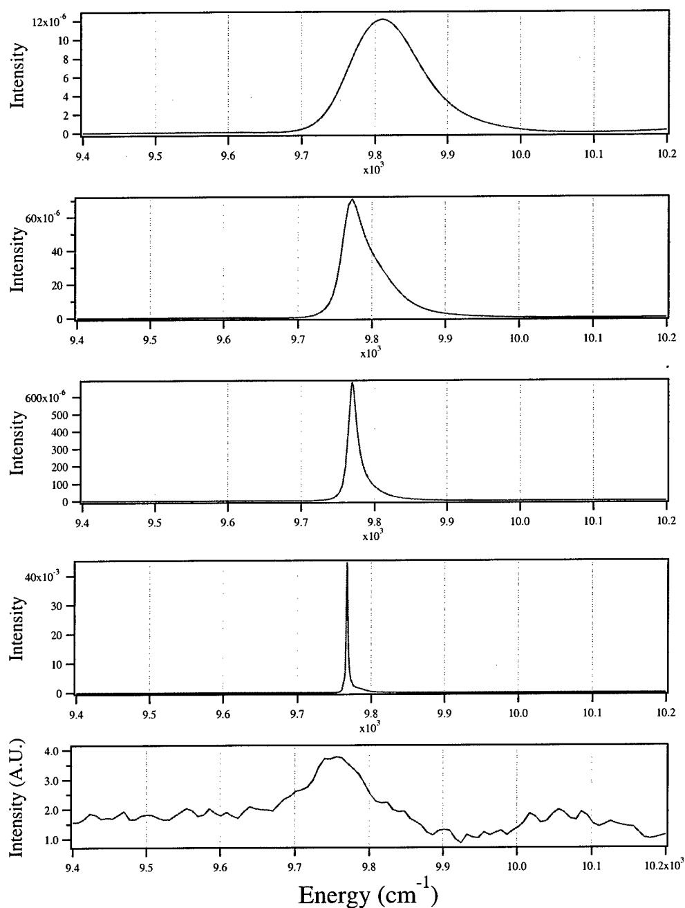
Figure 5.45: Triangular superlattice diffraction data compared with simulations for various oxide thicknesses. Simulations and data are for -K_g^D diffraction with incident light at 2^\circ in the M direction. The oxide thickness for the simulations are, from the bottom up, 1600 nm, 900 nm, 300 nm, and 200 nm.
