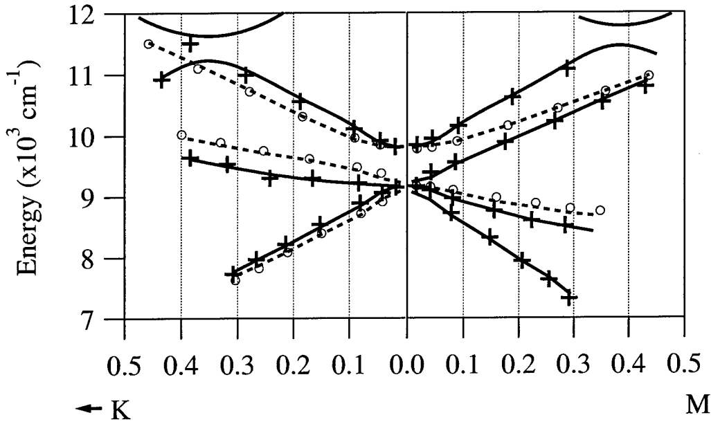
Figure 5.6: Dispersion diagram for the planar waveguide with the triangular lattice discussed in the text. The crosses represent s-polarized data. The circles represent p-polarized data. The solid lines represent s-polarized simulations. The dashed lines represent p-polarized simulations.
