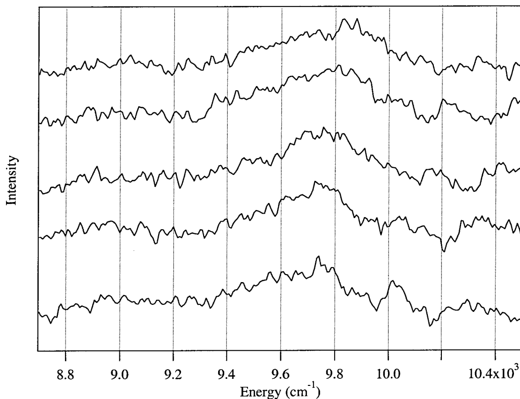
Figure 5.33: Unpolarized +K_g^D diffraction data for T-5. Spectra from the bottom up are for incident angles of 2^\circ , 4^\circ , 6^\circ , 8^\circ , and 10^\circ .
