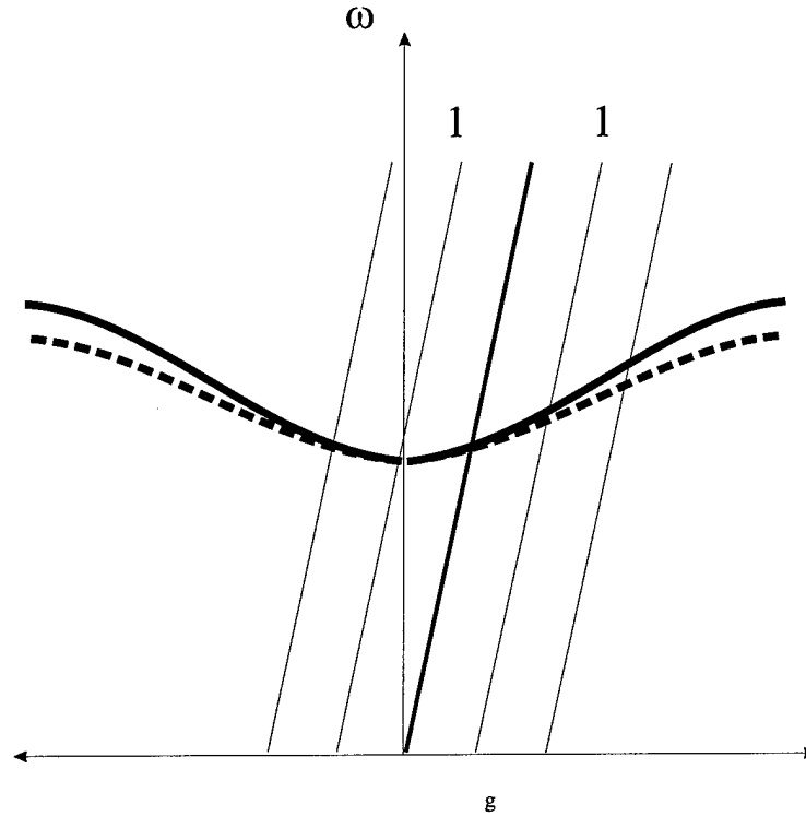
Figure 5.30: Schematic diagram illustrating the diffraction probe technique. The bold, straight line at 0 represents the parameter space directly stimulated by the incident light. The dashed line represents the upper most p-polarized band, and the solid represents the upper most s-polarized band of the triangular lattice structure (see Figure 5.6).
