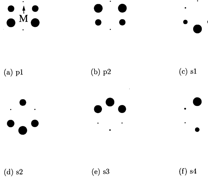
Figure 5.8: Momentum space diagrams for each Bloch mode of the triangular lattice at K_{||}=0.01K_g in the M direction. The M direction is toward the top of the page. The strength of each Fourier component is indicated by the size of the dot. The labels for each diagram correspond to the labels on the modes shown in Figure 5.5
