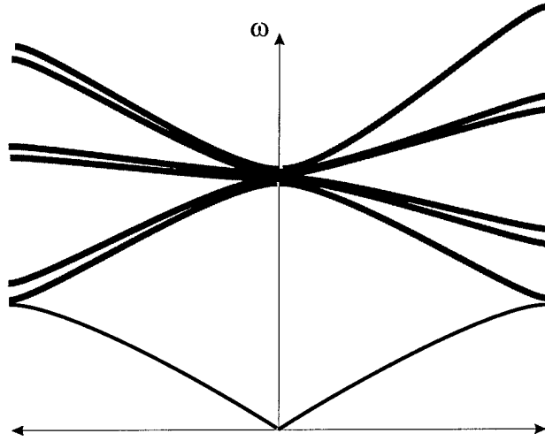
Figure 2.6: Schematic dispersion diagram for a thin planar waveguide textured with a 2D triangular lattice.
