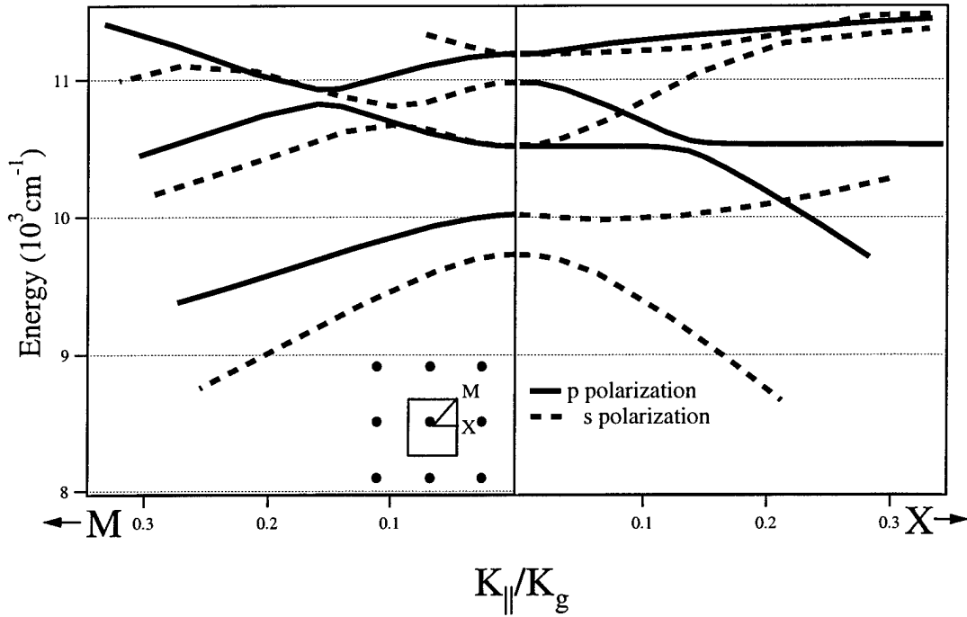
Figure 5.22: Theoretical dispersion diagram for the 150 nm thick textured planar waveguide with the square lattice discussed in the text. Note the p-polarized, low-dispersion bands near 10,000 \text{cm}^{-1} . [17]
