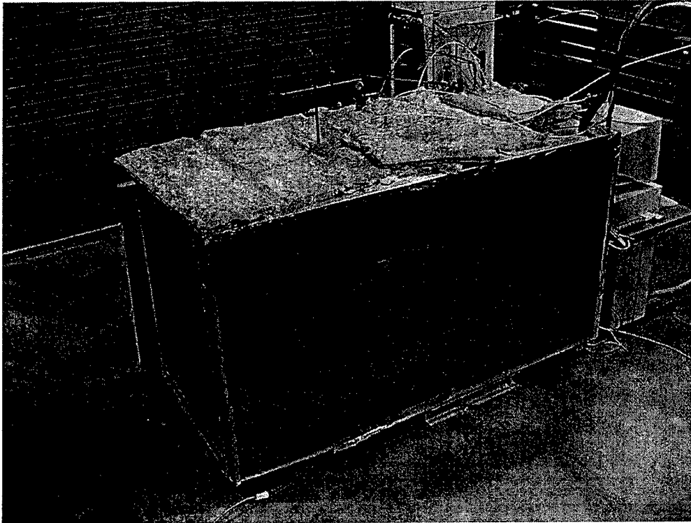
FIGURE 3. PHOTO OF FUEL TANK SPECIMEN IN THE AIRCRAFT COMPONENTS FIRE TEST FACILITY
