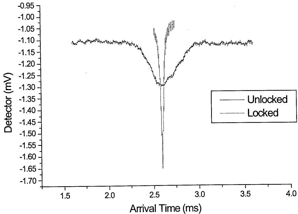
Figure 8: Comparison of measured hole when laser is locked to the spectral hole, and when only stabilized by its internal cavity.
