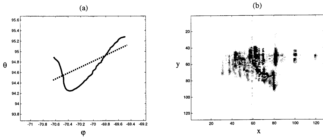
Fig. 11 3D motion and resulting ISAR image (frame 18).
