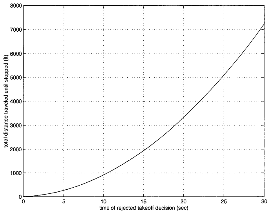
Figure 57. Total runway used versus t_{\text{evade}} , time evasive action began for the nominal takeoff profile.
