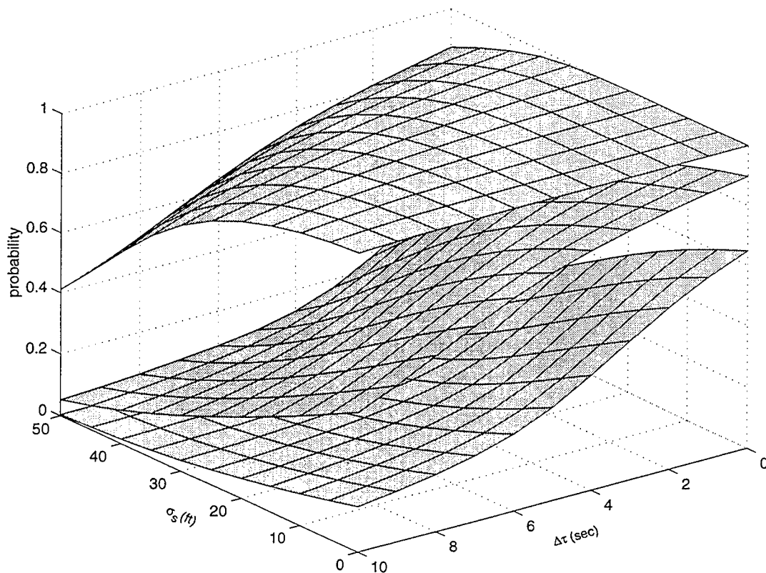
Figure 25. Safe probability surface for taxi, 5, 10, and 15 kts, direct cockpit alert with B-747 on runway.
