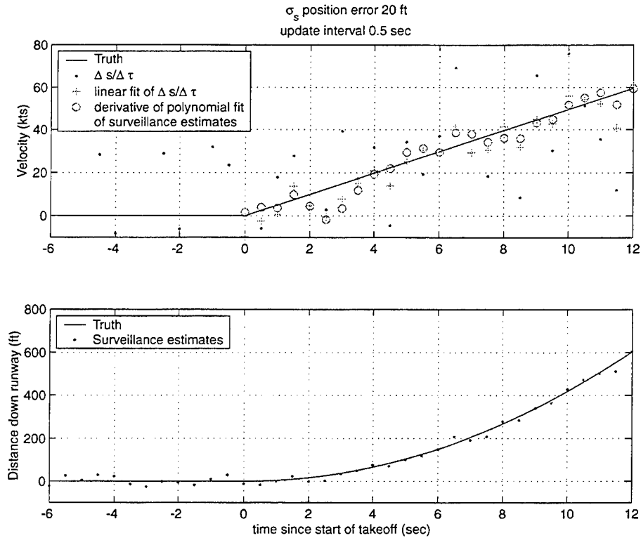
Figure 42. Monte Carlo trial of velocity estimates with \sigma_s = 20 feet and \Delta\tau = 0.5 seconds.
