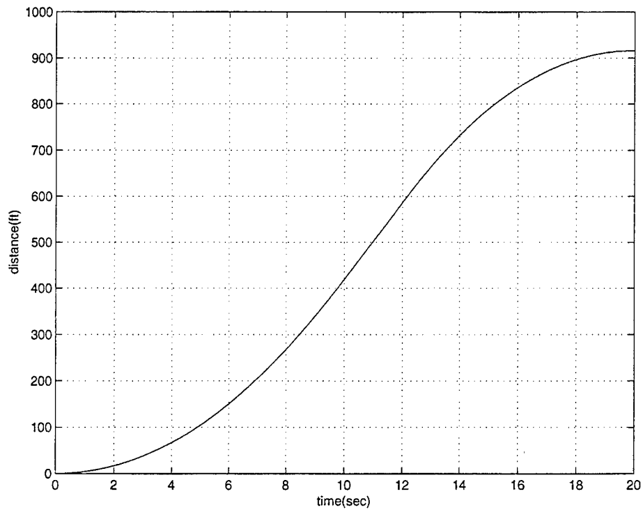
Figure 56. Distance vs. time for nominal takeoff rejected at t_{\text{evade}} = 10 seconds.
