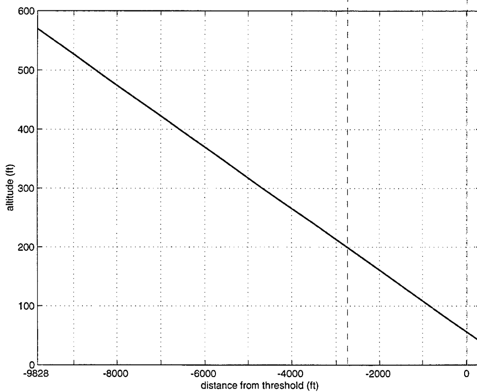
Figure 66. Timing analysis for a 150 knot arrival and a 0.26g acceleration to 150 knot departure.
