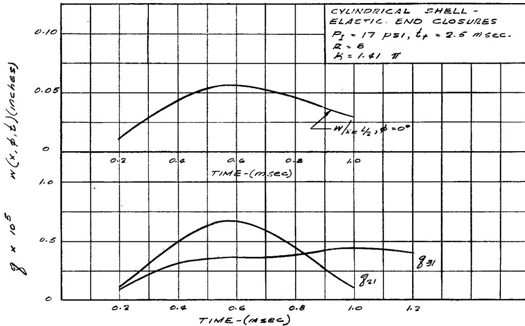
FIGURE 3.21. VARIATION OF q_{mn}(t) AND RADIAL DISPLACEMENT w(t) AT x = L/2, \phi = 0^\circ FOR CYLINDRICAL SHELL
