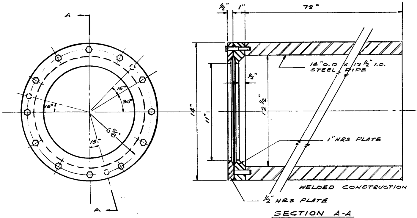
FIGURE II. 4. FIXTURE FOR CIRCULAR, FLAT PLATE MODELS
