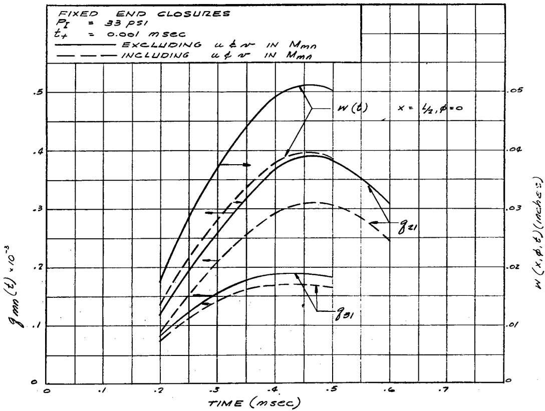
FIGURE 3. 16. VARIATION OF g_{mn}(t) AND RADIAL DISPLACEMENT w(t) AT x = L/2, \phi = 0^\circ FOR CYLINDRICAL SHELL
