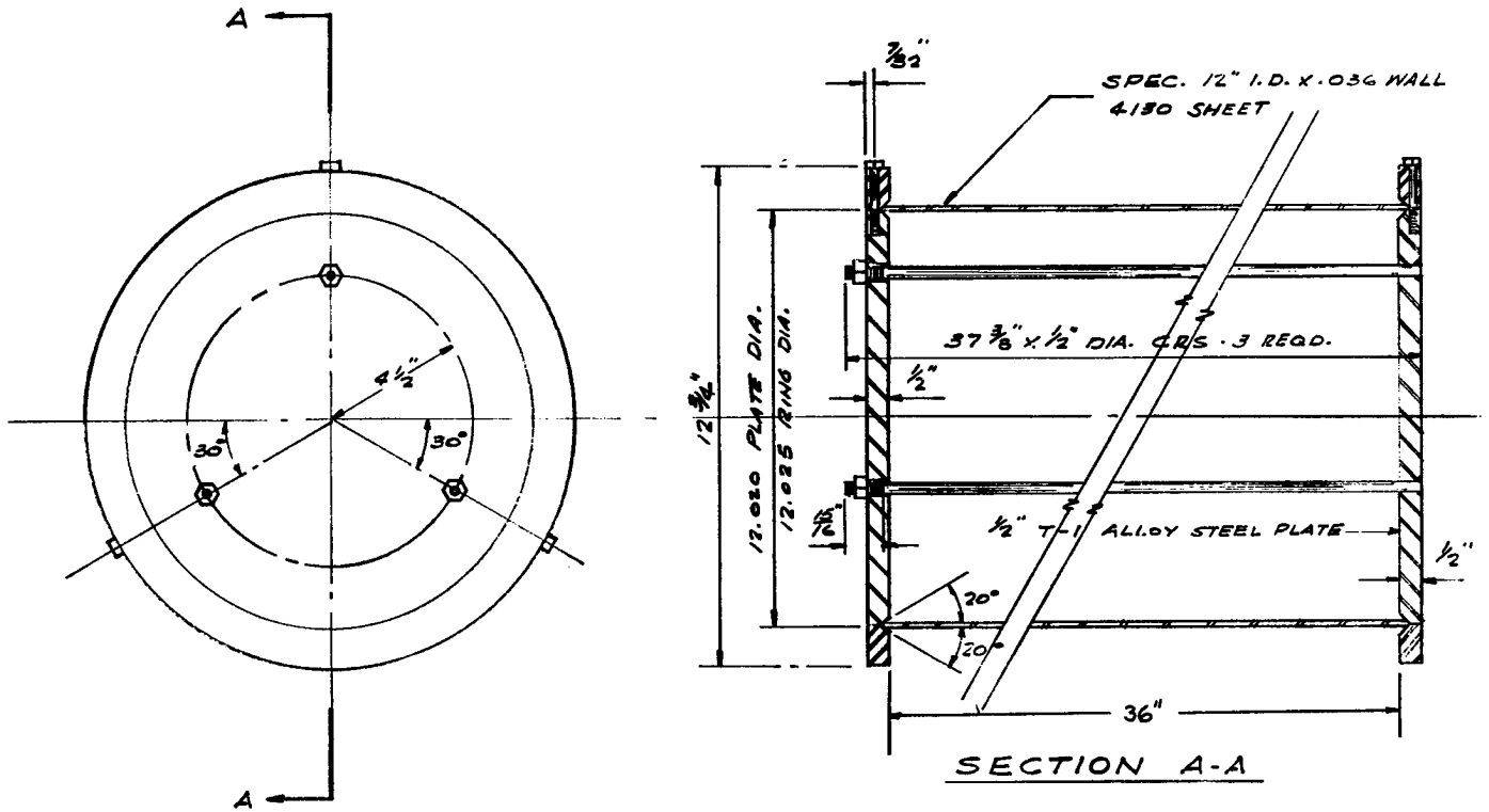
FIGURE II. 3. TYPE CB CYLINDRICAL SHELL MODELS
