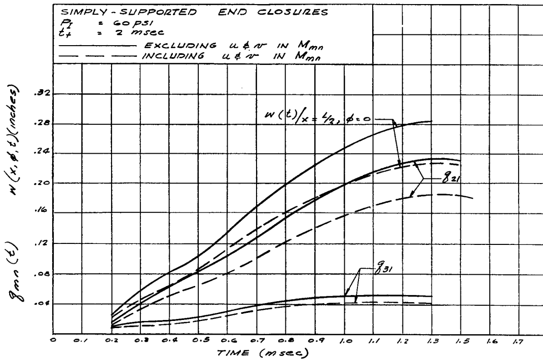
FIGURE 3.12. VARIATION OF g_{mn}(t) AND RADIAL DISPLACEMENT w(t) AT x = L/2, \phi = 0^\circ FOR CYLINDRICAL SHELL
