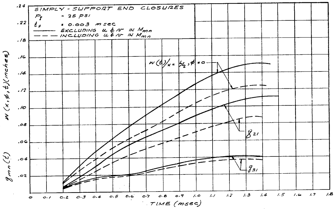
FIGURE 3.6. VARIATION OF q_{mn}(t) AND RADIAL DISPLACEMENT w(t) AT x = L/2, \phi = 0^\circ FOR CYLINDRICAL SHELL.
