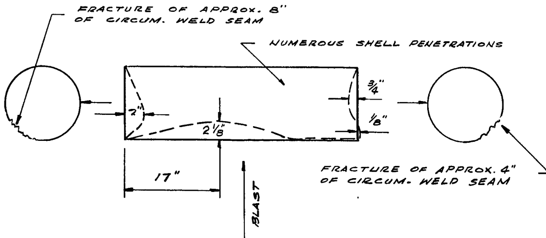
FIGURE II. 10. END PLATE AND SHELL FAILURE IN MODEL CC1 AFTER SHOT B3
