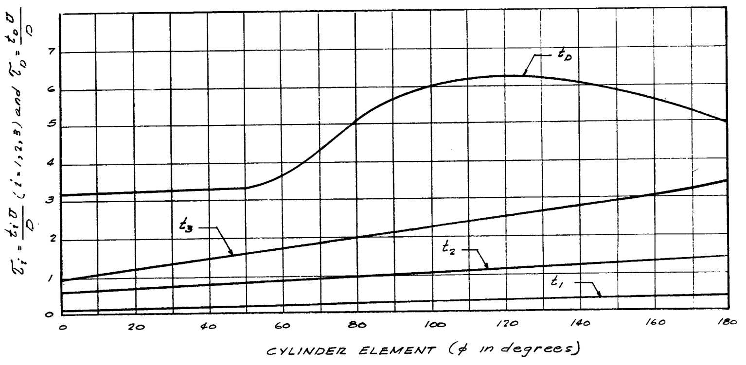
FIGURE I. 8. VARIATION OF CRITICAL TIMES ( t_i ) AND DIFFRACTION PHASE DURATION ( t_D ) WITH CYLINDER ELEMENT
