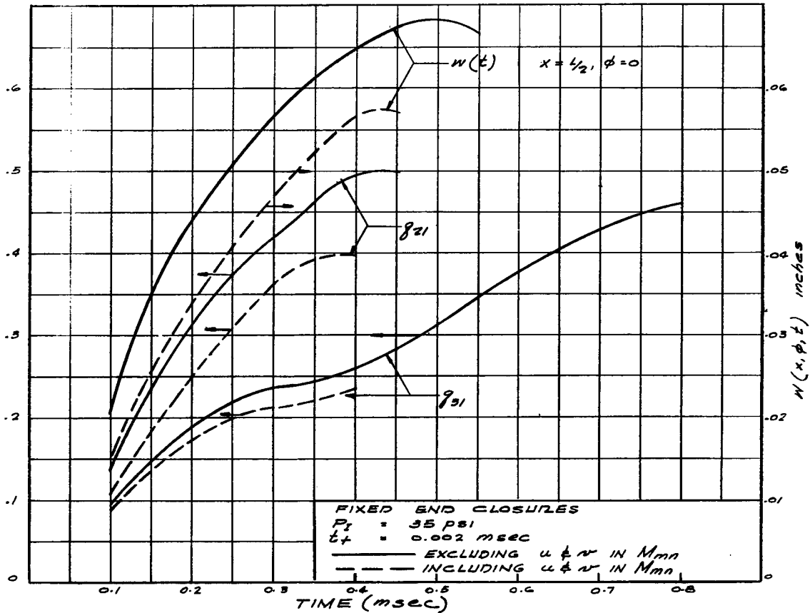
FIGURE 3. 17. VARIATION OF g_{mn}(t) AND RADIAL DISPLACEMENT w(t) AT x = L/2, \phi = 0^\circ FOR CYLINDRICAL SHELL
