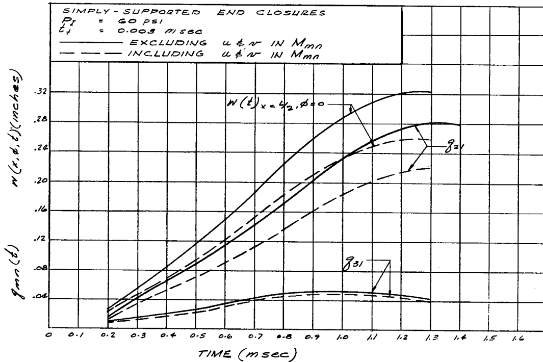
FIGURE 3.13. VARIATION OF g_{mn}(t) AND RADIAL DISPLACEMENT w(t) AT x = L/2, \phi = 0^\circ FOR CYLINDRICAL SHELL
