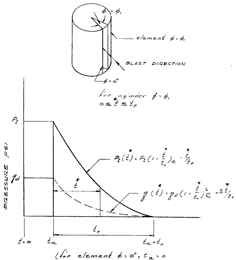
FIGURE I. 5. INCIDENT OVERPRESSURE AND DYNAMIC PRESSURE VERSUS TIME
