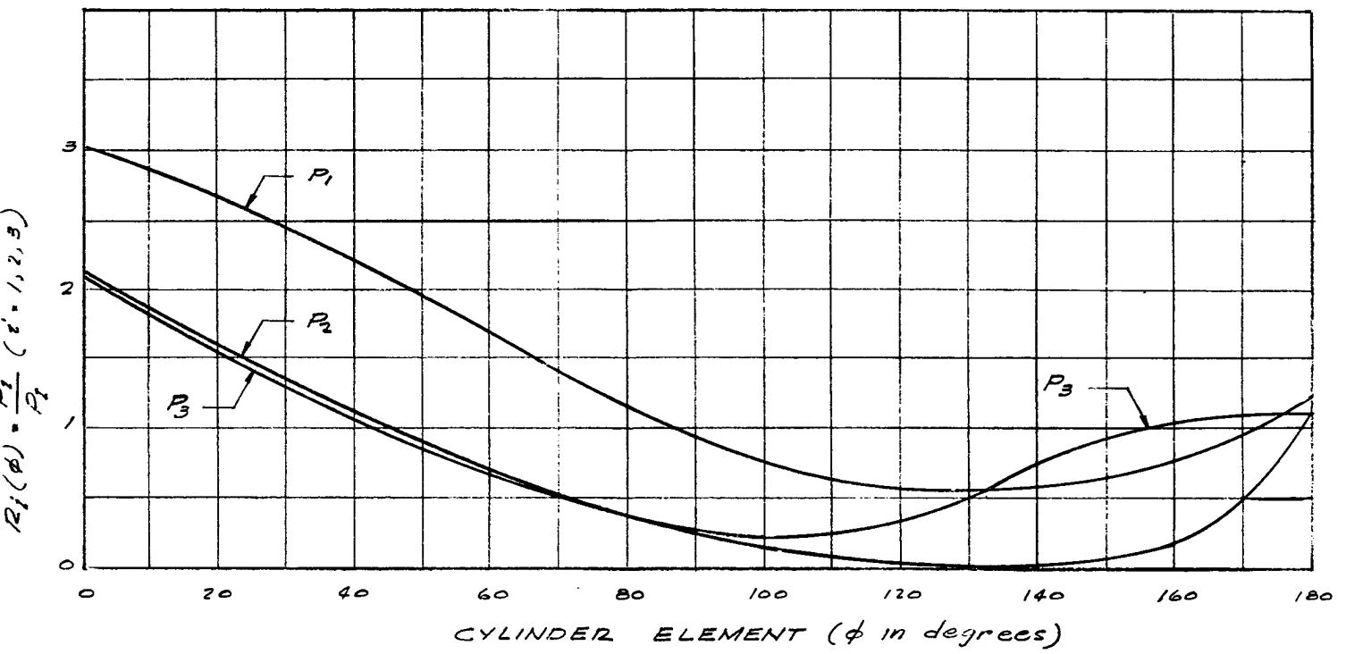
FIGURE I. 9. VARIATION OF CRITICAL PRESSURE ( P_j ) TO PEAK INCIDENT OVERPRESSURE ( P_1 ) RATIOS WITH CYLINDER ELEMENT
