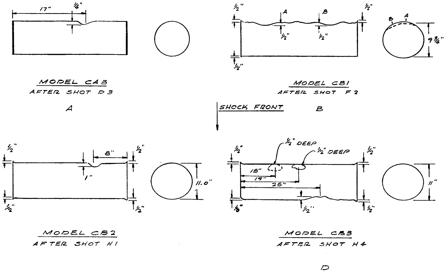
FIGURE II. 17. FAILURE STATE OF MODELS USED IN SHOTS D, F, AND H
