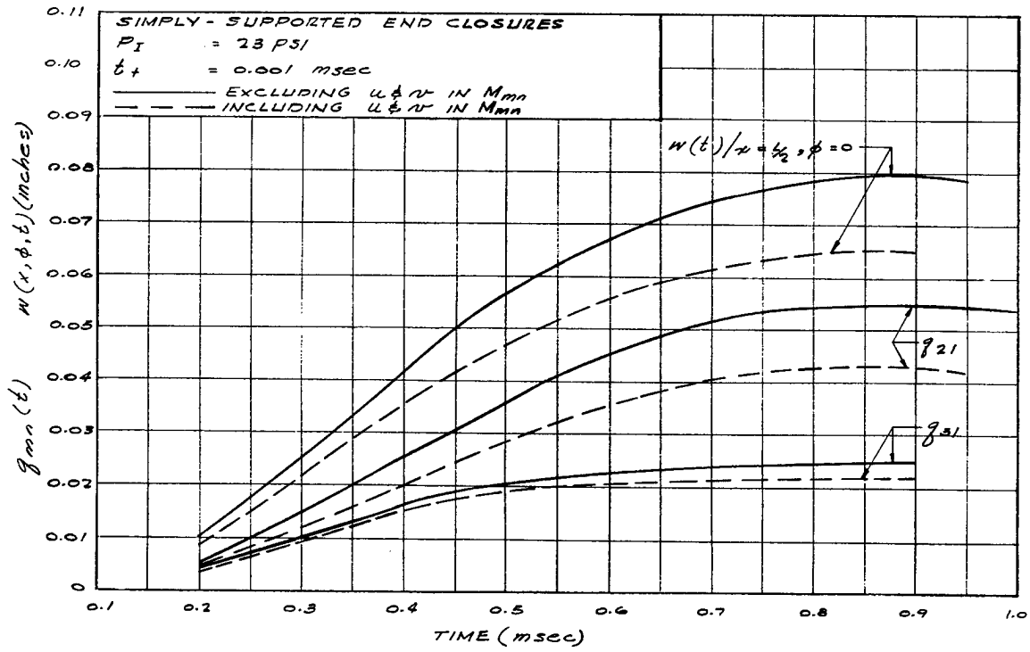
FIGURE 3.4. VARIATION OF g_{mn}(t) AND RADIAL DISPLACEMENT w(t) AT x = L/2, \phi = 0^\circ FOR CYLINDRICAL SHELL
