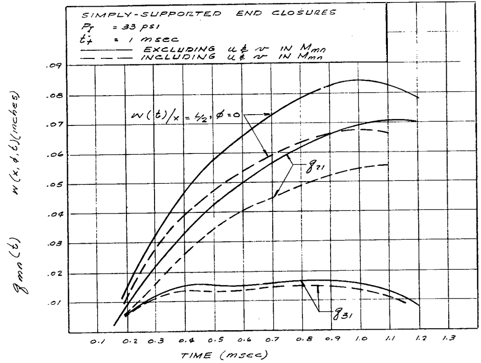
FIGURE 3.7. VARIATION OF q_{mn}(t) AND RADIAL DISPLACEMENT w(t) AT x = L/2, \phi = 0^\circ FOR CYLINDRICAL SHELL.
