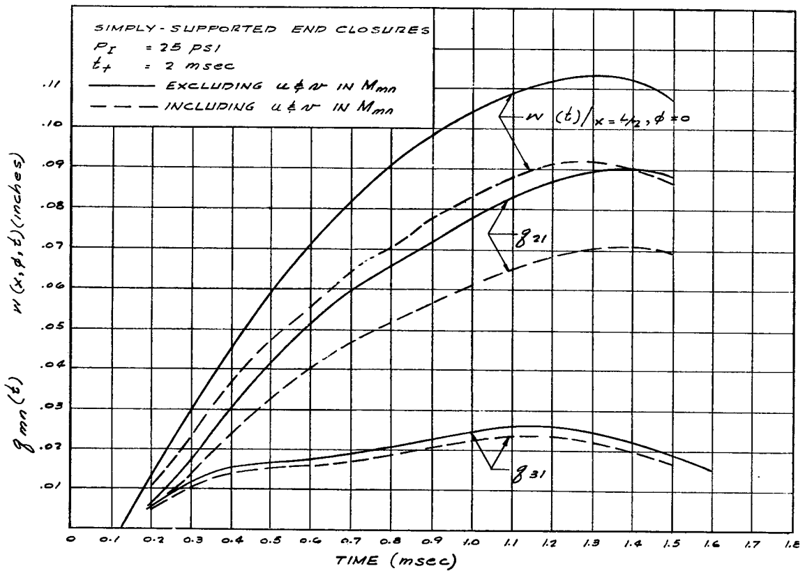
FIGURE 3.5. VARIATION OF g_{mn}(t) AND RADIAL DISPLACEMENT w(t) AT x = L/2, \phi = 0^\circ FOR CYLINDRICAL SHELL
