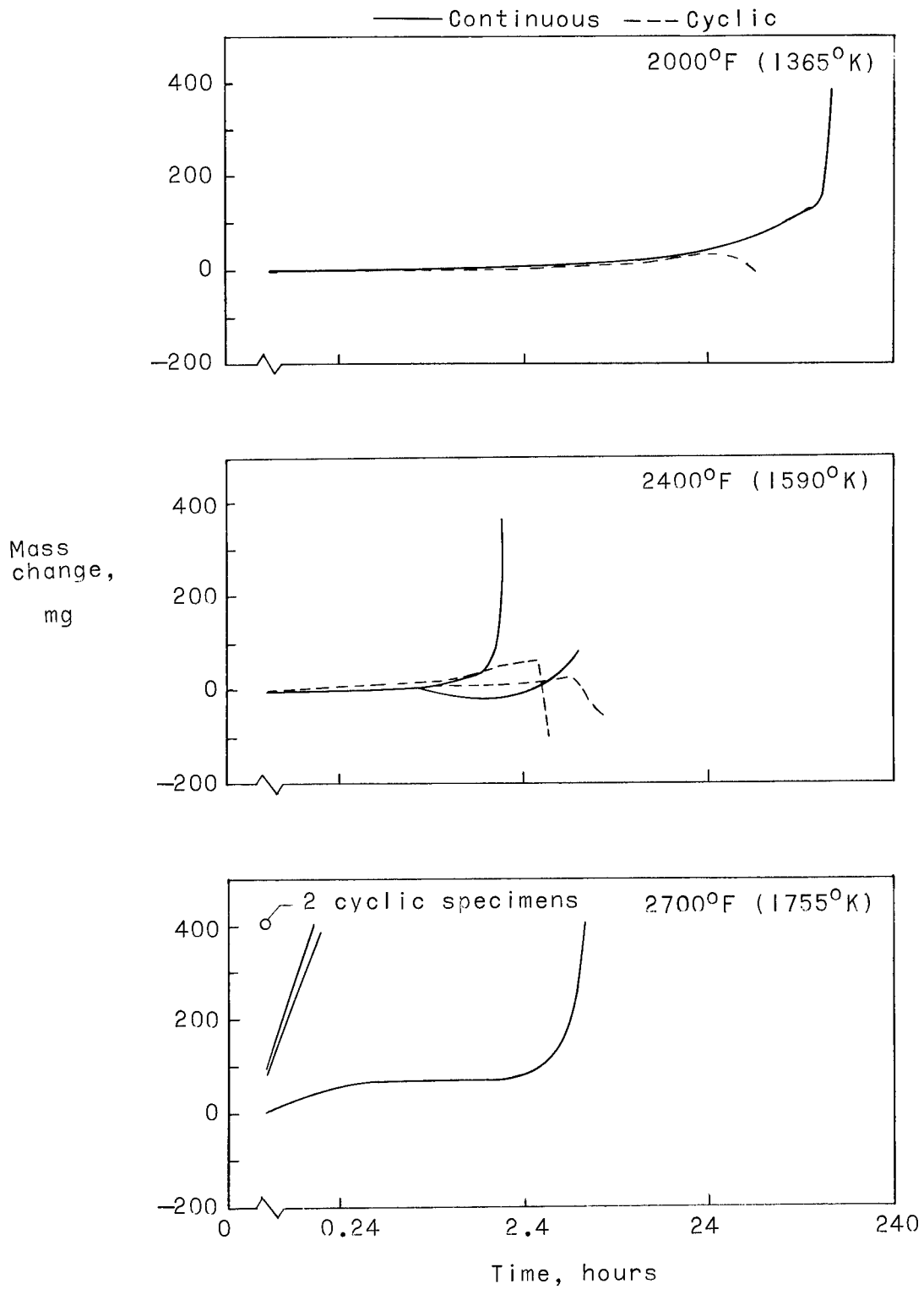
Figure 23.- Mass change histories for specimens of coating 7 on Cb-10Ti-5Zr alloy sheet tested in air at atmospheric pressure.
