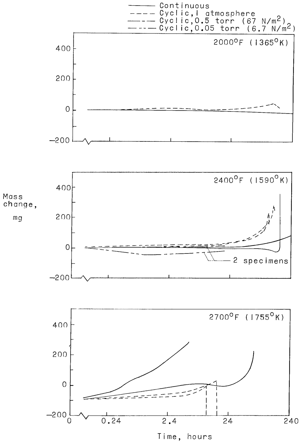
Figure 26.- Mass change histories for specimens of coating 8 on Cb-10Ti-5Zr alloy sheet tested in air.
