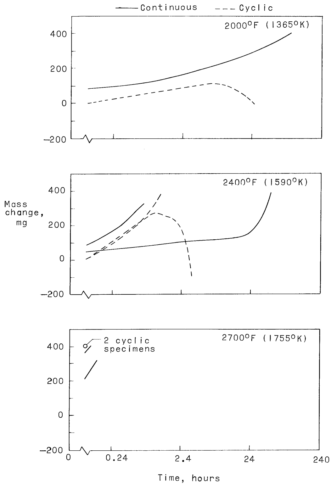
Figure 4.- Mass change histories for specimens of coating 1 on Cb-10Ti-5Zr alloy sheet tested in air at atmospheric pressure.
