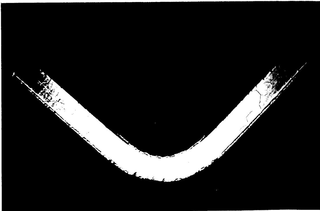
Figure 45.- Cross-sectional view of a specimen of coating 12 exhibiting a ductile bend after 240 hours of continuous exposure at 2000° F (1365° K). X 25.
