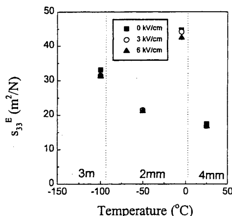
FIG. 4. s_{33}^E as a function of temperature for the \langle 001 \rangle -poled \text{BaTiO}_3 crystals under various dc bias.
