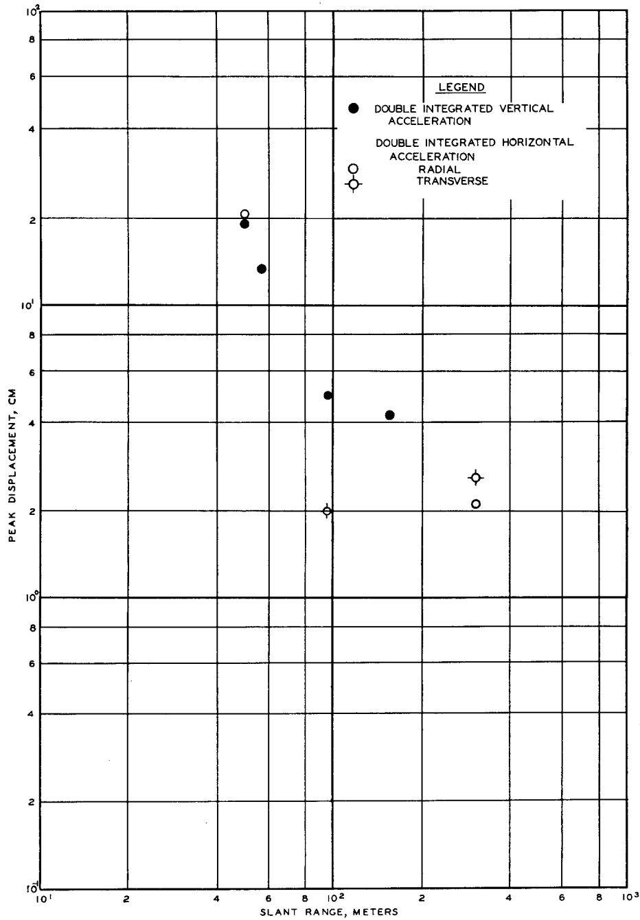
Figure 3.8 Peak displacement versus distance.
