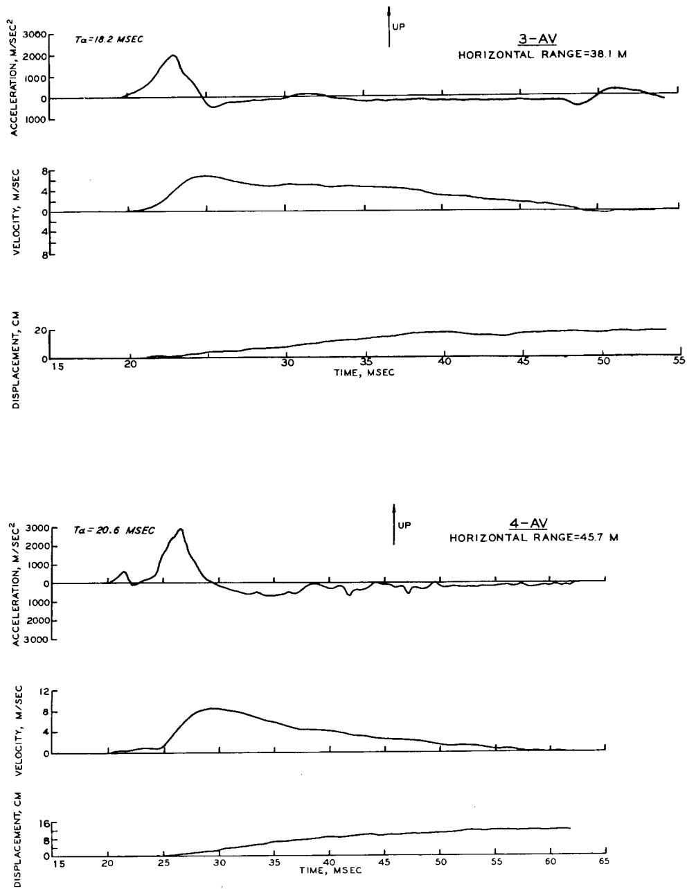
Figure 3.5 Corrected acceleration histories with twofold integrations (1 of 4 pages).
