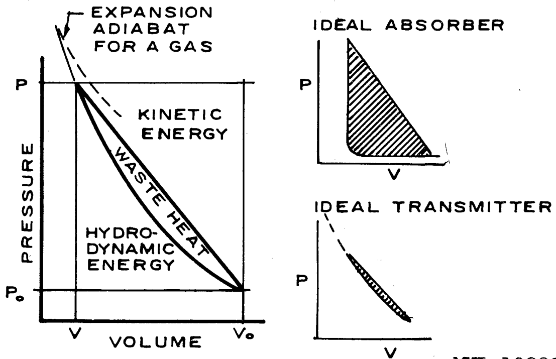
Fig. 3. 3. Waste heat concept.
