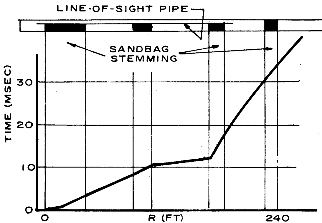
Fig. 3.2. Logan - time of arrival. MUL-10219
