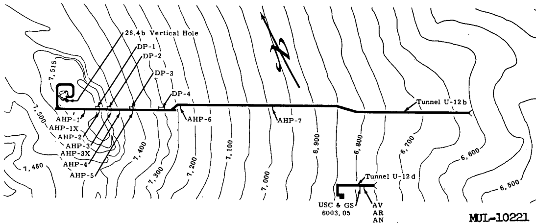
Fig. 4.1. Plan and elevation, Rainier tunnel.
