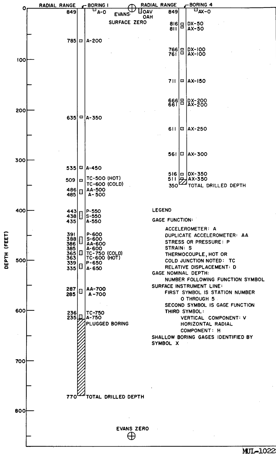
Fig. 4. 2. Distribution of vertical instrumentation for Evans.
