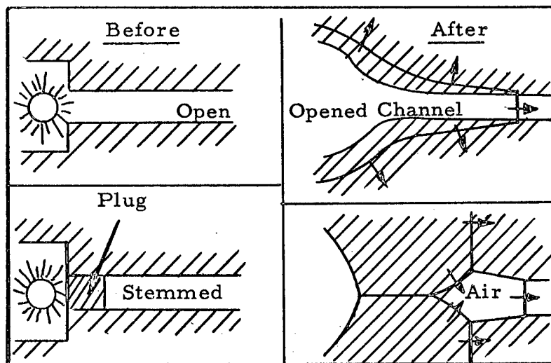
Fig. 3.6a. Open channel (upper figures).
