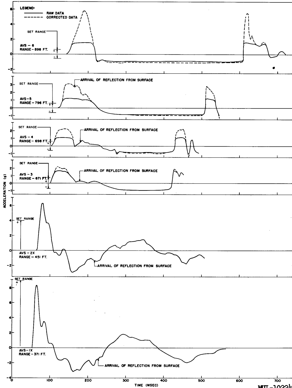
Fig. 4.4. Acceleration - time records, vertical radius.
