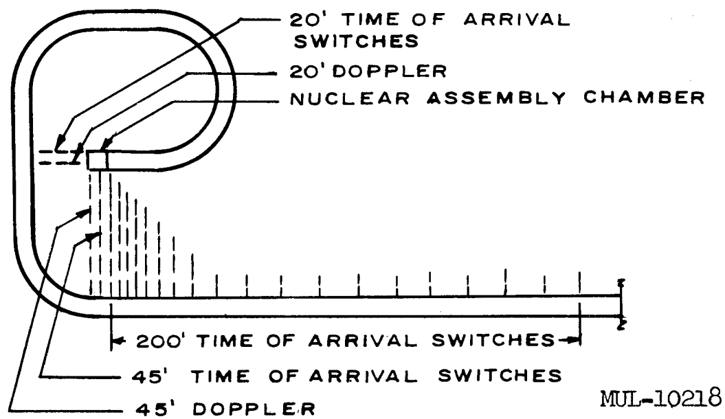
Fig. 3.1. Rainier equipment layout.
