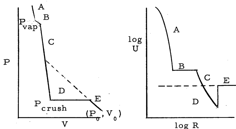
Fig. 3.4a. Pressure-velocity diagram for soil.
