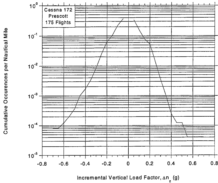
FIGURE C-37. CUMULATIVE OCCURRENCES OF INCREMENTAL MANEUVER LOAD FACTOR PER NAUTICAL MILE
