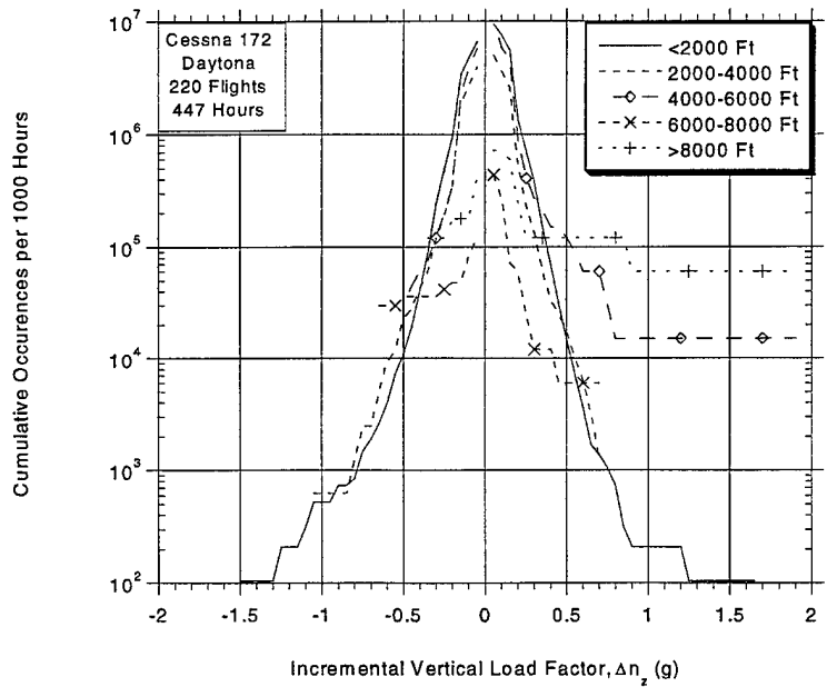
FIGURE B-18. CUMULATIVE OCCURRENCES OF INCREMENTAL GUST LOAD FACTOR PER 1000 HOURS BY ALTITUDE ABOVE AIRPORT FOR DEPARTURE PHASE
