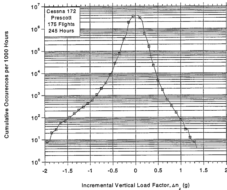
FIGURE C-22. CUMULATIVE OCCURRENCES OF INCREMENTAL GUST LOAD FACTOR PER 1000 HOURS, COMBINED FLIGHT PHASES
