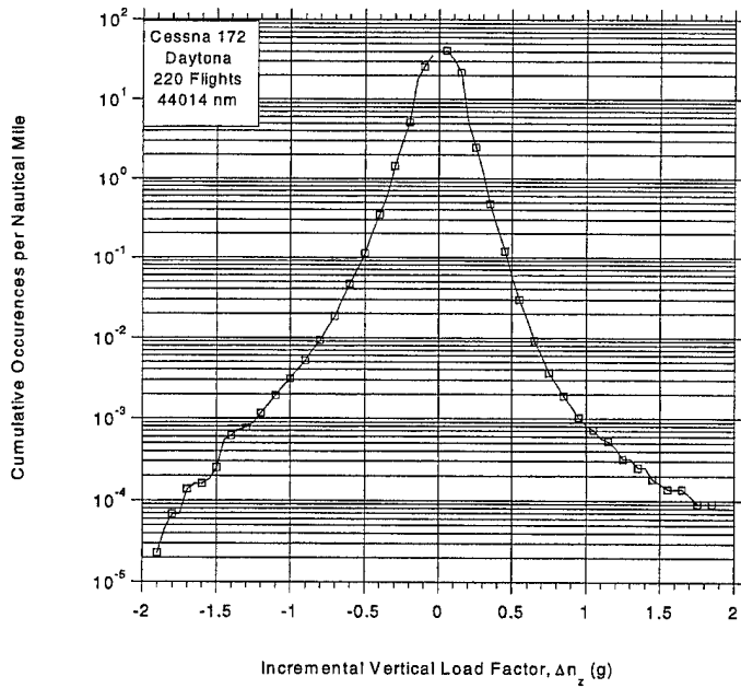
FIGURE B-23. CUMULATIVE OCCURRENCES OF INCREMENTAL GUST LOAD FACTOR PER NAUTICAL MILE
