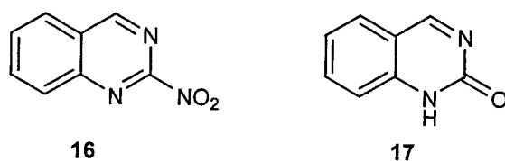
Figure 3.2. Potential products from the quinazoline nitration.
