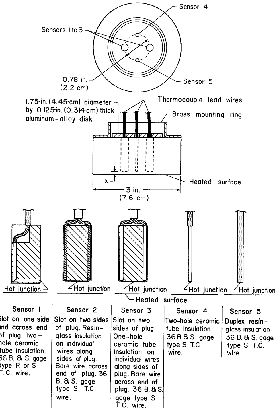
Figure 1.- Details of thermocouple sensors used in charring ablator specimens. Plugs 1 to 3 are made of the same ablation material as that used in the test specimens. All plugs are 0.25-in. (0.635-cm) diameter.
