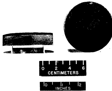
L-64-5211 Figure 4.- Charring ablator specimen after testing.
