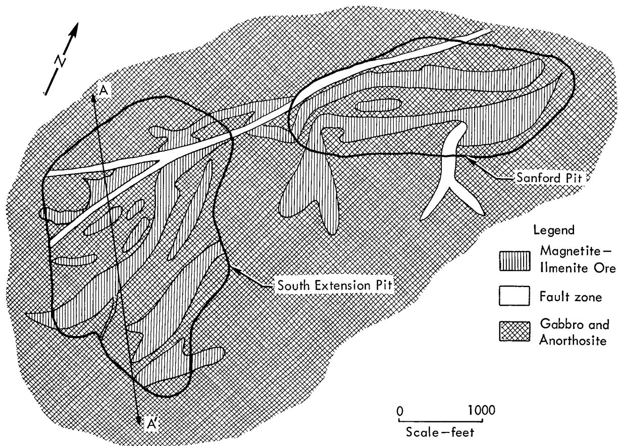
Figure A.58 Sanford and South Extension Pits; generalized geological map. (Adapted from data contributed by National Lead Company)
