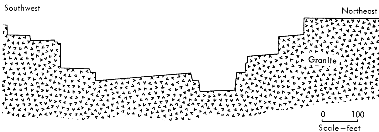
Figure A.32 Fletcher Quarry; representative profile. (Adapted from data contributed by H. E. Fletcher Company)
