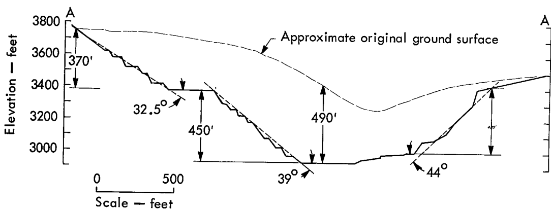
Figure A.3 Bagdad Pit; plan and representative profile. (Adapted from Reference 51, Hardwick and Jones, 1959)
