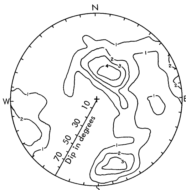
A. Attitude of joints west of Dome Fault; percentage of 745 joints
