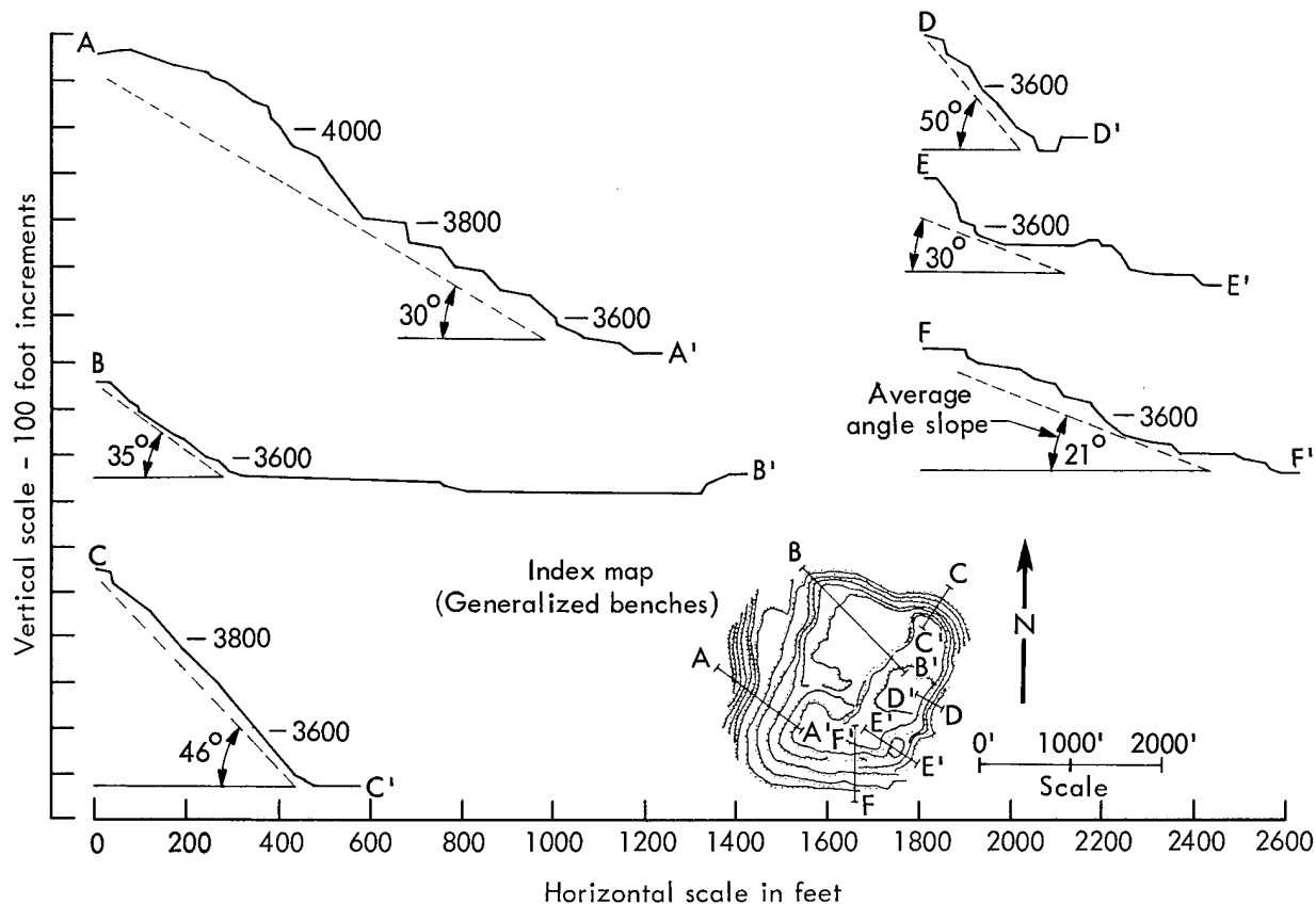
Figure A.45 Thornton Pit; generalized plan and representative profiles. (Adapted from Reference 49, Hardwick, 1963)
