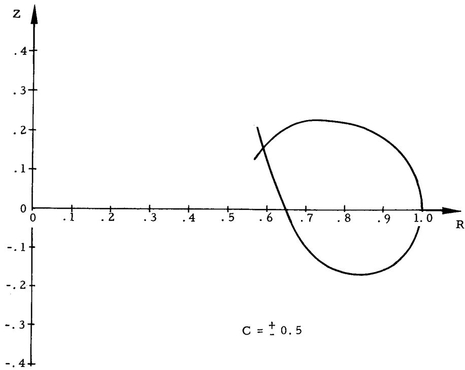
Figure 19.- Isotensoid Shape for Linear Pressure Gradient.
