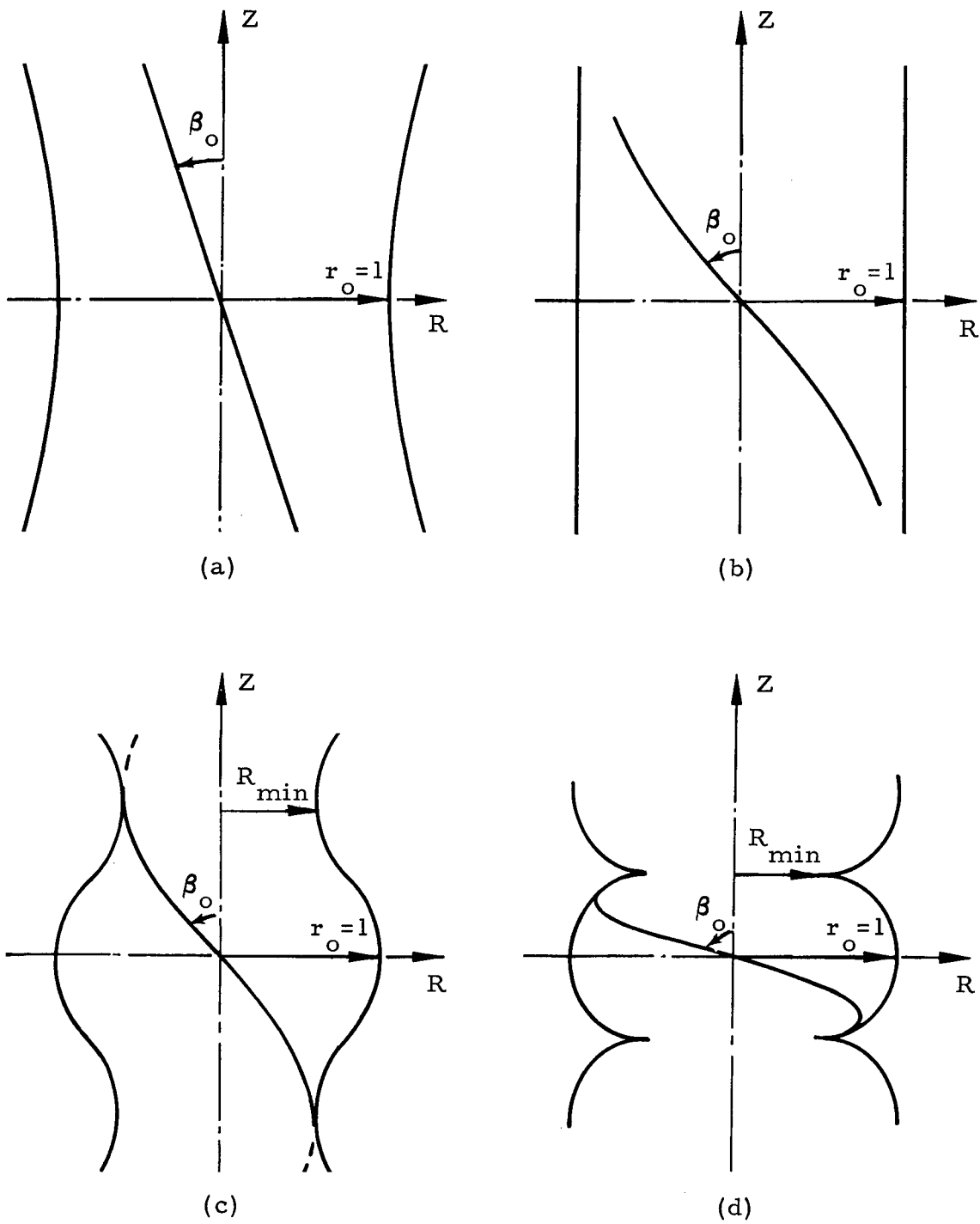
Figure 8. - Isotensoid Meridional Shapes.
