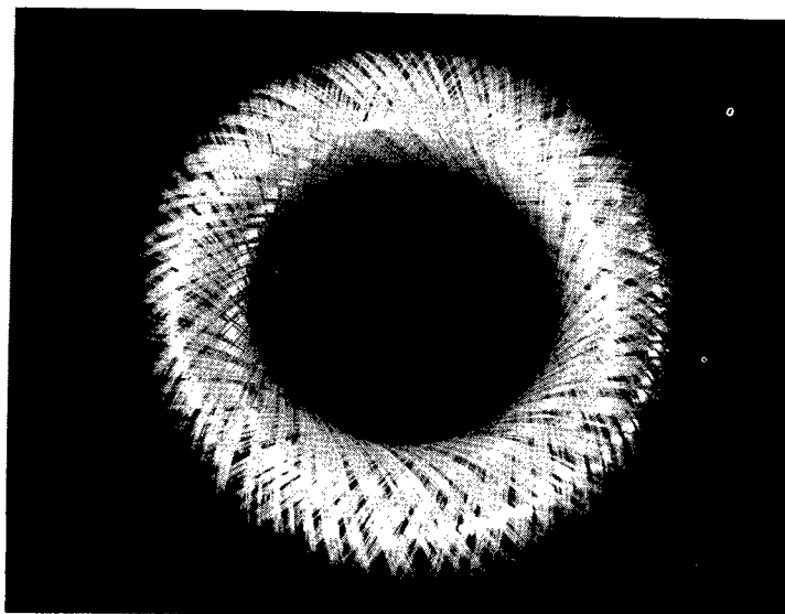
Figure 20.- Isotensoid Shape and Filament Geometry for Closed Torus C = \pm .35 K = 4.4 .
