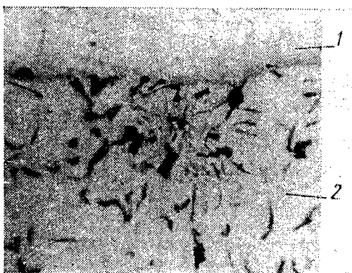
Figure 22. Structure of brazed sample at the border of alloying of brass with cast iron (X 200). 1 - brass LKN 56-03-6; 2 - cast iron
