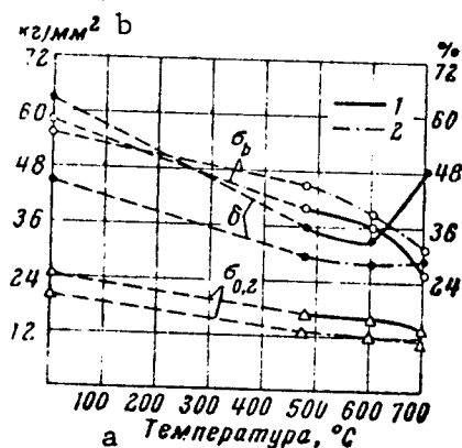
Fig. 1. Properties of steel EI-846 with 0.1 o/o of boron. Melting: Line 1 -- in vacuum; line 2 -- in air. a) Temperature, degrees C; b) kg/mm 2 .
