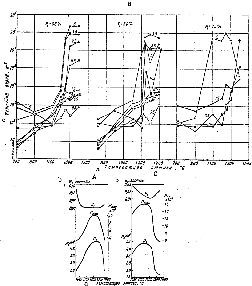
Fig. 5. Influence of temperature of deep-vacuum annealing on magnetic properties and grain size of iron-nickel alloys of brands 50N (A, B) and 79NM (C). Annealing in furnace MPV-2M, vacuum 10^{-4} mm mercury column. a) Temperature of annealing; b) oersteds; c) grain size.
