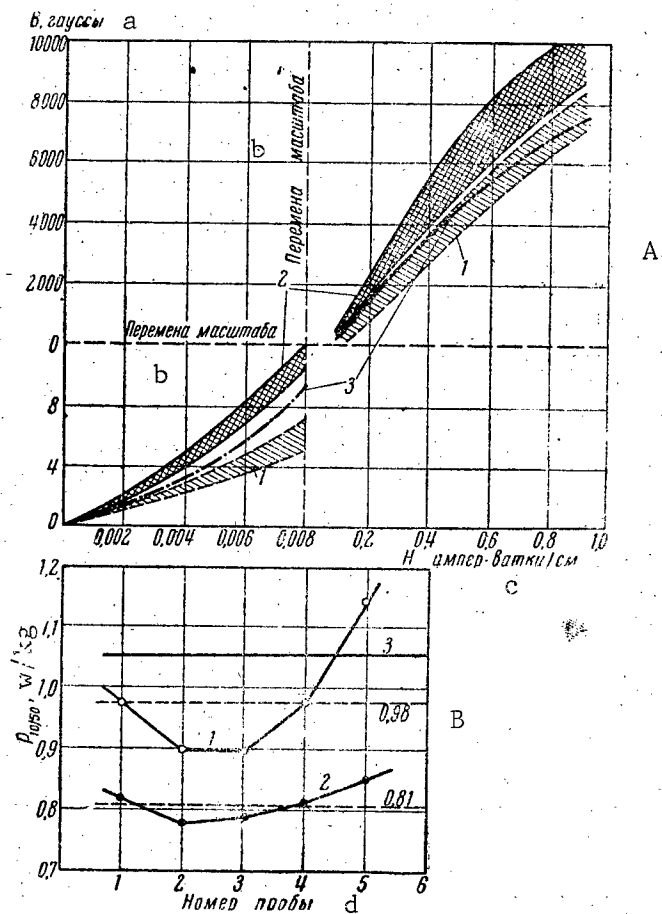
Fig. 4. Influence of depth of vacuum on magnetic induction (A) and specific losses (B) of transformer steels; 1 -- annealing in cupola furnace UKP-03B, vacuum 50 mm mercury column; 2 -- annealing in retort, vacuum 0.1 mm mercury column; 3 -- requirement of All-Union Government Standard 802-58 (brands E46 and E43). a) B , Gauss; b) change of scale; c) H ampere-vatki/cm; d) number of test.
