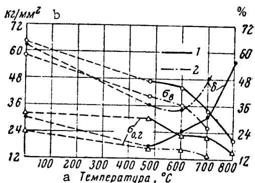
Fig. 2. Properties of steel EI-846, melted in vacuum: line 1 -- with 0.1 o/o tungsten; line 2 -- with 0.8 o/o tungsten. a) Temperature, degrees C; b) kg/mm 2 .
