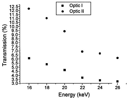
Figure 15. Transmission as a function of energy for taper I and II.
