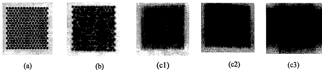
Figure 2. X-ray images of the field at the locations marked (a)–(c) in figure 1. The fiber structure of the optic is clearly visible in (a). Location of (b) is 17 cm after the optic. The divergence has blurred the fiber structure. Post crystal images are measured using a Fuji image plate for silicon (400) (c1), for mica (0010) (c2) and for graphite (002) (c3).
