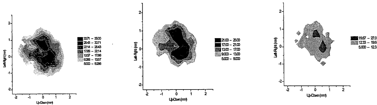
Figure 18. Transmission uniformity at 14 keV, 18 keV, and 22 keV, respectively.
