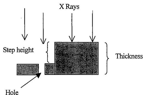
Figure 11. Shape of the polypropylene step phantom used for figure 12 and table 4.
