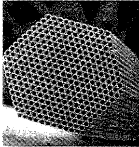
Figure 1. Cross sectional electron picture of polycapillary fiber 500 μm in diameter. This fiber has approximately 100 channels, each 50 μm in diameter.
