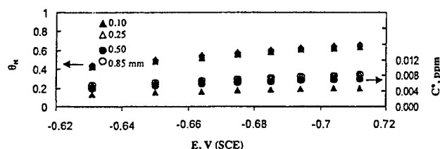
Figure 5. The relation between the hydrogen surface coverage, \theta_{\text{H}} , and the electrode potential, E , obtained on iron membranes of different thicknesses in 0.1 N \text{H}_2\text{SO}_4 + 0.9 N \text{Na}_2\text{SO}_4 , and the corresponding hydrogen concentration, C^0 , in the iron membrane at the input surface.
