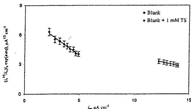
Figure 6. The relation between (\sqrt{i_e/i_0}) i_e \exp(\alpha\eta) and the steady-state permeation current density, i_e . Blank = 1 M \text{Na}_2\text{SO}_4 , pH 2, TS = \text{S}_2\text{O}_3^{2-} .
