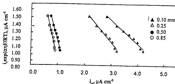
Figure 3. The relation between the charging function, i_c \exp(\alpha\eta F/RT) , and the steady-state hydrogen permeation current density, i_\infty , for iron membranes of different thickness in 0.1 N \text{H}_2\text{SO}_4 + 0.9 N \text{Na}_2\text{SO}_4 .
