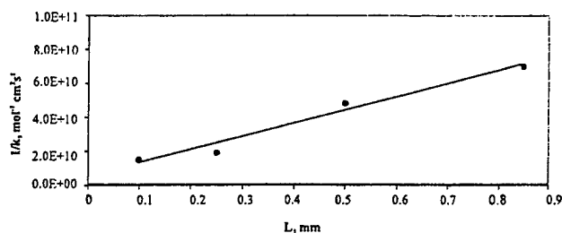
Figure 4. The relation between the reciprocal of the kinetic-diffusion constant, k , and the membrane thicknesses, L , for iron in 0.1 N \text{H}_2\text{SO}_4 + 0.9 N \text{Na}_2\text{SO}_4 .
