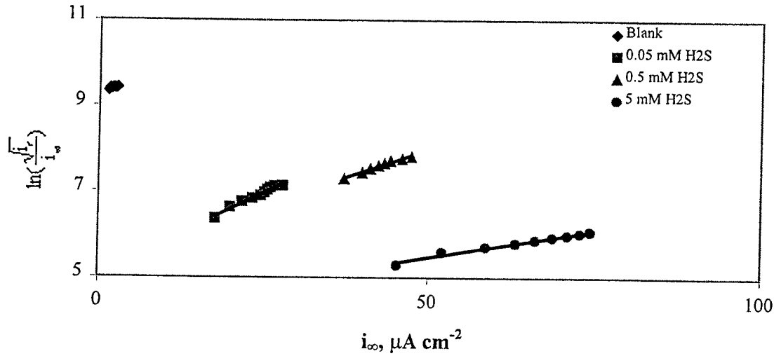
Figure 5 The relation between \ln\left(\frac{\sqrt{i_r}}{i_\infty}\right) and i_\infty obtained at different hydrogen sulfide concentrations at pH 2
