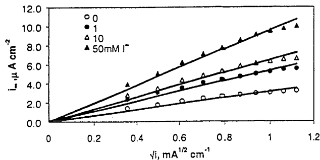
Figure 4. Relationship between the steady-state hydrogen permeation current, i_\infty , and the square root of the hydrogen recombination current, \sqrt{i_r} , obtained on an iron membrane in 0.1 N H 2 SO 4 + 0.9 N Na 2 SO 4 , at different iodide ion concentrations.
