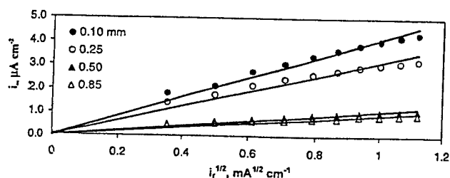
Figure 2. The relation between the steady-state hydrogen permeation current density, i_\infty , and square root of the recombination current density, \sqrt{i_r} , obtained on iron membranes of different thicknesses in 0.1 N \text{H}_2\text{SO}_4 + 0.9 N \text{Na}_2\text{SO}_4 (pH 1.8).
