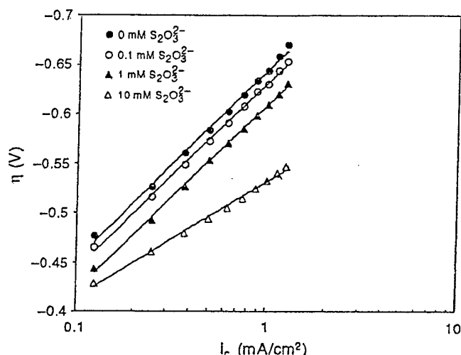
FIGURE 5. Effect of \text{S}_2\text{O}_3^{2-} concentration on the Tafel plots of the HER obtained on a steel membrane of thickness 0.25 mm in 0.5 M \text{Na}_2\text{SO}_4 .
