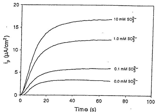
FIGURE 6. Effect of \text{SO}_3^{2-} concentration on the hydrogen permeation transients obtained on a steel membrane of thickness 0.25 mm in 0.05 M \text{H}_2\text{SO}_4 + 0.45 M \text{Na}_2\text{SO}_4 (pH 1.8) at a charging current density of 1.25 mA/cm 2 .
