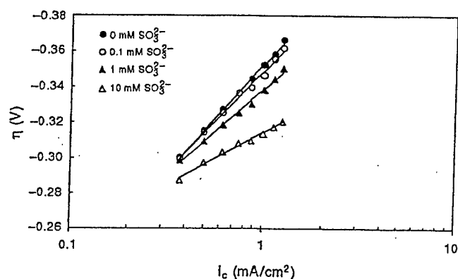
FIGURE 7. Effect of \text{SO}_3^{2-} concentration on the Tafel plots of the HER obtained on a steel membrane of thickness 0.25 mm in 0.05 M \text{H}_2\text{SO}_4 + 0.45 M \text{Na}_2\text{SO}_4 at a charging current density of 1.25 mA/cm 2 .
