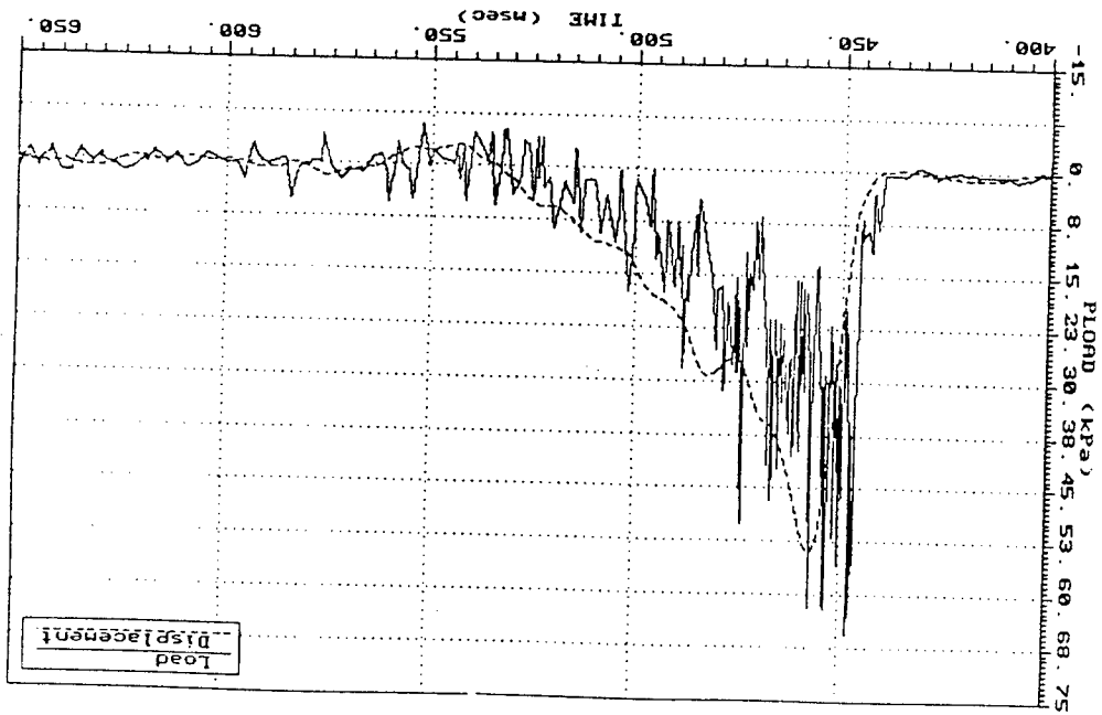
Figure 4: A representative sample of the measured load and resultant calculated chest wall displacement time histories.
