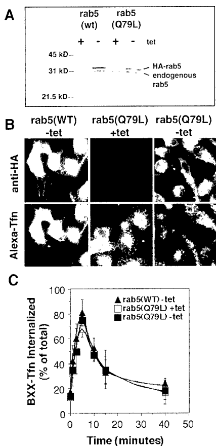
FIG. 1. HA-Rab5(Q79L) expression in stably transformed tTA-HeLa cells causes enlarged endosomes but does not effect Tfn endocytosis or recycling. tTA-HeLa cells stably expressing either HA-Rab5(WT) or HA-Rab5(Q79L) under control of a tetracycline ( tet )-regulatable promoter were clonally selected as described under "Materials and Methods." Cells were incubated in the absence (induced) or presence (uninduced) of 1 \mu g/ml tetracycline for 48 h. A , immunoblots of cell lysates probed with antibodies against Rab5 showing expression of endogenous and HA-tagged Rab5. B , transformed tTA-HeLa cells uninduced or induced to express either HA-Rab5(WT) or HA-Rab5(Q79L) as indicated were incubated with Alexa-Tfn ( lower panels ) for 20 min at 37 °C before fixation, permeabilized in 0.1% saponin, and processed for indirect immunofluorescence using the 12CA5 anti-HA antibody ( upper panels ), as described under "Materials and Methods." C , single-round kinetics of uptake and recycling of prebound biotinylated Tfn in tTA-HeLa cells uninduced ( \square ) or induced to express either HA-Rab5(WT) ( \blacktriangle ) or HA-Rab5(Q79L) ( \blacksquare ) for 48 h as described under "Materials and Methods." Results are average \pm S.D. of three independent experiments.
