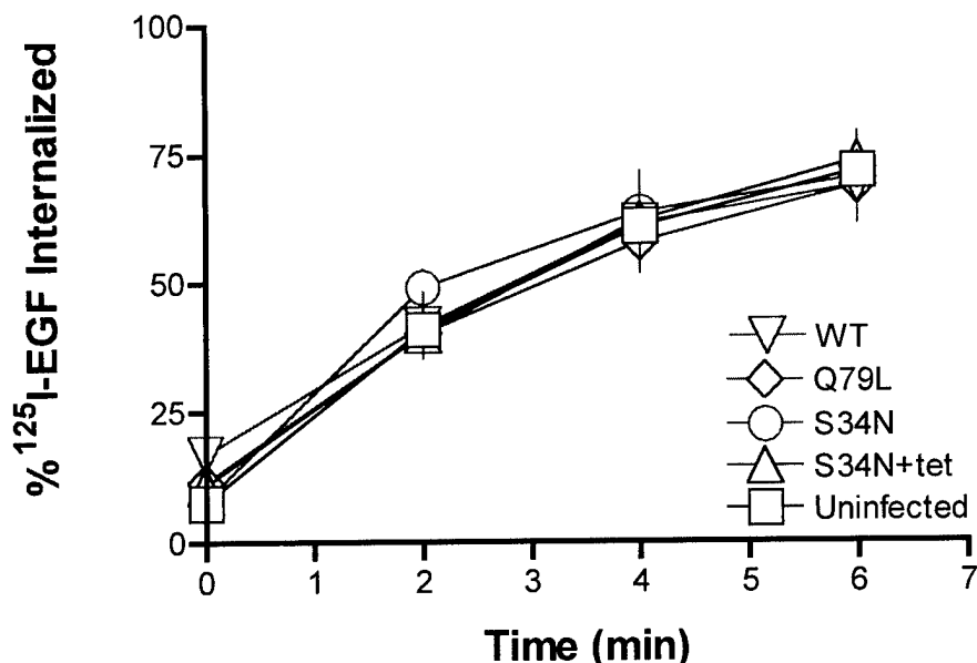
Figure 1. Overexpression of rab5(WT), rab5(Q79L), or rab5(S34N) has no effect on the rate of ^{125}\text{I} -EGF internalization. Subconfluent 35 mm dishes of tTA-HeLa cells were infected for 2 hours with adenoviruses encoding for the indicated rab5 mutants. Cells were returned to growth media for 18 hours and then assayed for ^{125}\text{I} -EGF internalization. Briefly, the infected cells were incubated on ice for 2 hours with XX nM ^{125}\text{I} -EGF ( ci/mol) to achieve steady-state binding of cell surface EGFR. Free radioligand was removed with a series of washes using ice cold PBS. The cells were incubated with pre-warmed 37^\circ\text{C} media for the indicated amounts of time, allowing for internalization of the radioligand/receptor complex. Dissociated ligand was removed with a series of ice cold PBS washes. Cell surface ^{125}\text{I} -EGF was measured as the amount of acid dissociatable radioligand (determined as the amount of radioactivity dissociated in two 8 min washes in 0.2M NaCl/0.2 M acetic acid) and internalized ^{125}\text{I} -EGF was assessed from the remaining cell associated radioactivity (assayed by solubilizing the remain cells in 1.0 M NaOH). Data are plotted as the percent internalized (cpm internalized/(cpm cell surface + cpm internalized)) at each time point. Data are plotted as the average \pm S.E.M. from 3-4 experiments from each condition.
