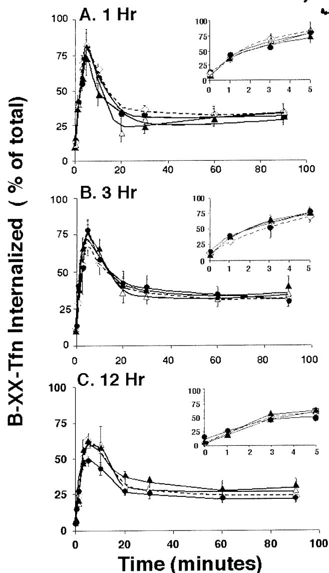
FIG. 4. Endocytic trafficking of transferrin is unaffected even by rapid induction of high levels of Rab5(Q79L) expression. Kinetics of uptake and recycling of prebound biotinylated Tfn were measured in uninfected tTA-HeLa cells ( \diamond ), tTA-HeLa cells infected with recombinant adenovirus that encode HA-Rab5(Q79L) but maintained in the presence of 1 \mu g/ml tetracycline ( \triangle ), or tTA-HeLa cells infected with adenovirus in the presence of cycloheximide and induced to express either HA-Rab5(WT) ( \blacktriangle ) or HA-Rab5(Q79L) ( \bullet ) after release from cycloheximide for 1, 3, and 12 h as described under "Materials and Methods." Transferrin endocytosis and recycling were examined using an enzyme-linked immunosorbent assay-based assay, which monitors the total level of internalized, prebound, and biotinylated transferrin as described under "Materials and Methods." Data are plotted as a percentage of the total biotinylated transferrin initially bound to the cells. The same data are shown over a shorter time course ( inset ).
