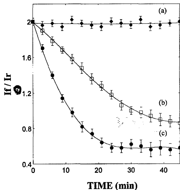
Figure 5. Temporal dependence of the ratio between the fluorescence intensities of fluorescein ( I_f ) and tetramethylrhodamine ( I_r ) in individual lipobeads monitoring the pH decrease during the enzymatic oxidation of glucose catalyzed by glucose oxidase. Curve a describes a control experiment where the lipobeads are suspended in a 10 mM oxygenated glucose solution in the absence of glucose oxidase. Curves b and c describe the fluorescence intensity of individual lipobeads in (b) air-saturated and (c) oxygen-saturated 10 mM glucose solutions containing 0.1 aunit/mL glucose oxidase. The fluorescence decrease is due to the accumulation of gluconic acid near the lipobead.
