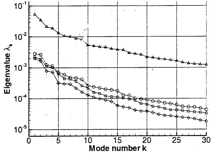
Figure 5.2: Eigenvalues from POD of run L2: u (o), v (□), h (◇), and \omega (△).
