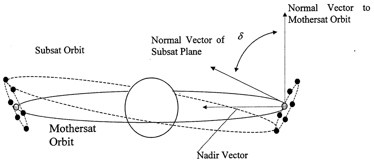
Figure 3.8 Cyclic motion of Subsat Orbit
