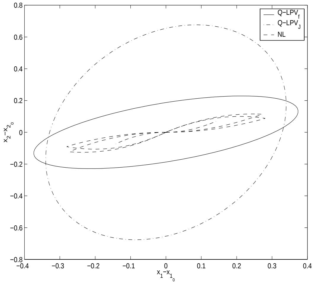
FIG. 5.3. The ellipsoids to contain a reachable set of the nonlinear dynamics.
