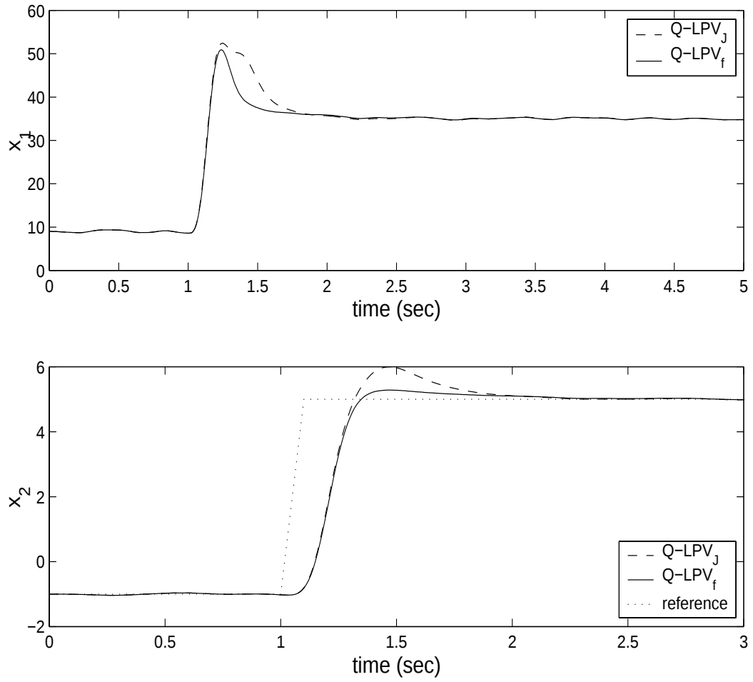
FIG. 5.8. The step responses based on different quasi-LPV models.
