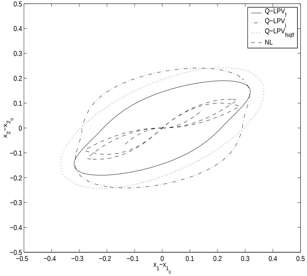
FIG. 5.6. The set to contain the reachable set \mathcal{R}_{bu} .
