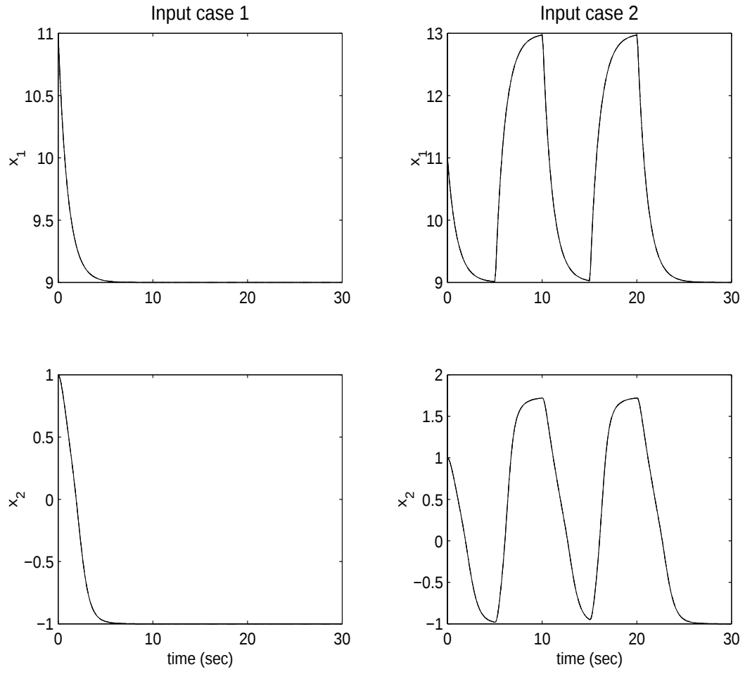
FIG. 5.2. Quasi-LPV model simulations at two input cases.
