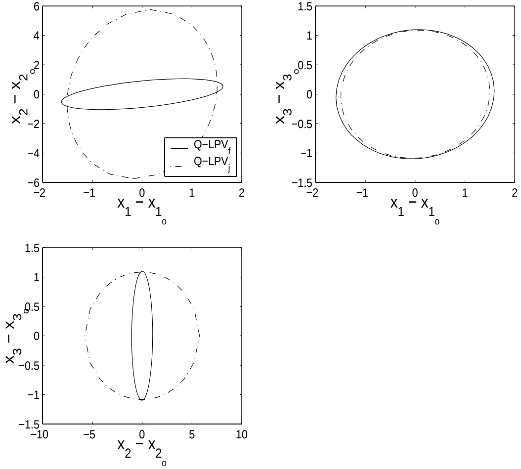
FIG. 5.5. The ellipsoids based on each quasi-LPV model with unmodeled dynamics.
