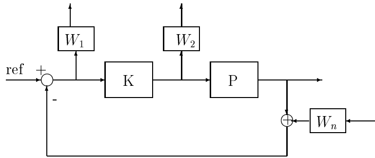
FIG. 5.7. Interconnection of LPV control synthesis
