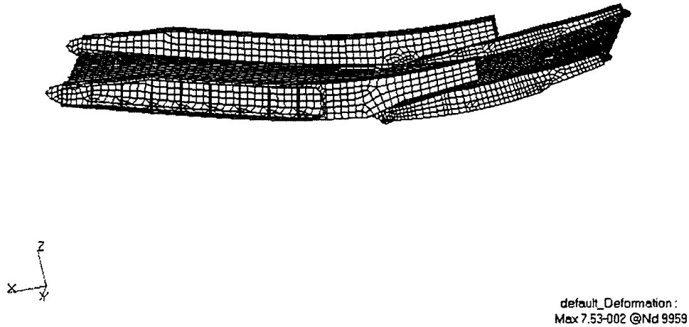
Figure 24. LMSR, Boundary Condition Case 3, Mode 3, Bending
