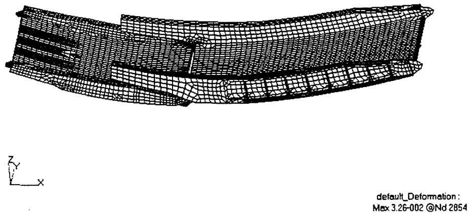
Figure 25. LMSR, Boundary Condition Case 4, Mode 1, Bending
