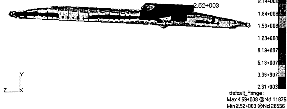
Figure 139. Cape T (right view) von Mises Stress Contour Plot, Max. Stress: 66.6 ksi (Inertia Loading, 3 Degree Twist, Two Tanks)
