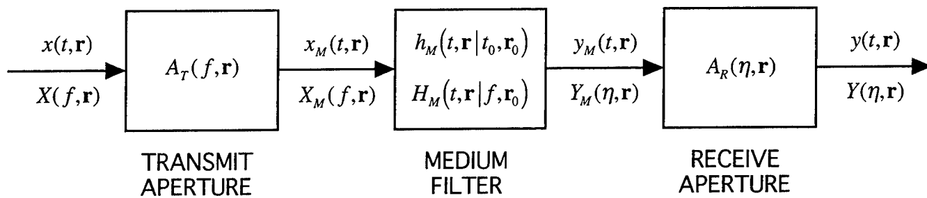
Figure 2.2-1. Block diagram model of small-amplitude pulse propagation.
