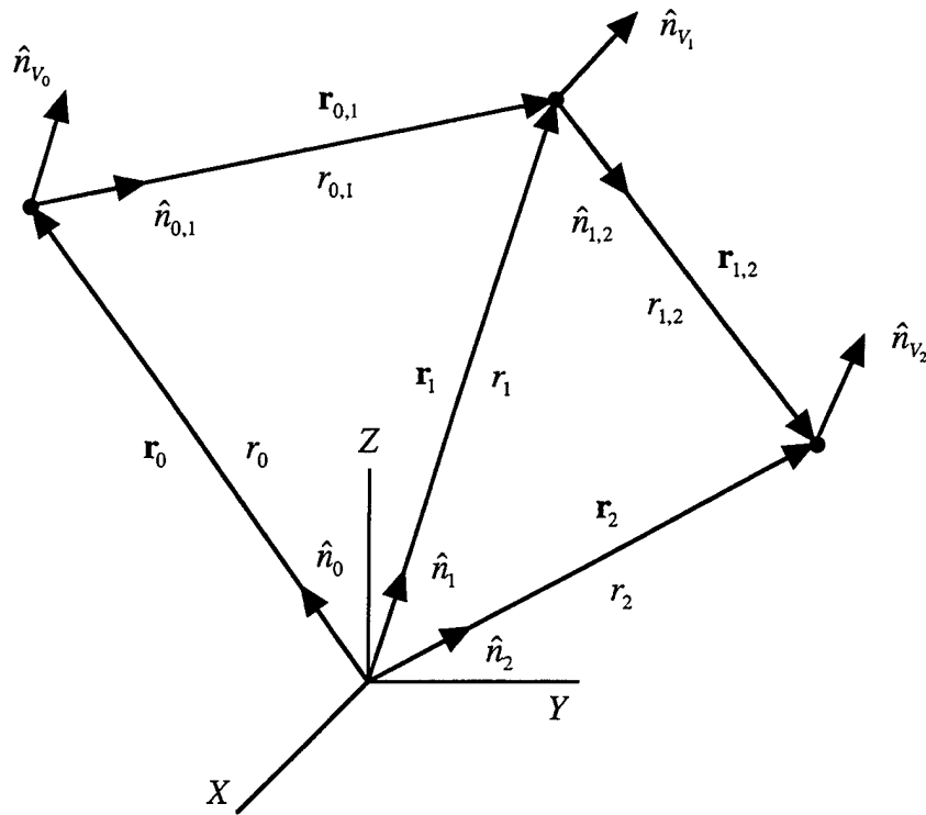
Figure 3.3-1. Bistatic scattering geometry when motion begins at time t = t_0 = 0 seconds. Point 0, P_0(\mathbf{r}_0) , is the transmitter; point 1, P_1(\mathbf{r}_1) , is the discrete point scatterer; and point 2, P_2(\mathbf{r}_2) , is the receiver. All three platforms are in motion.
