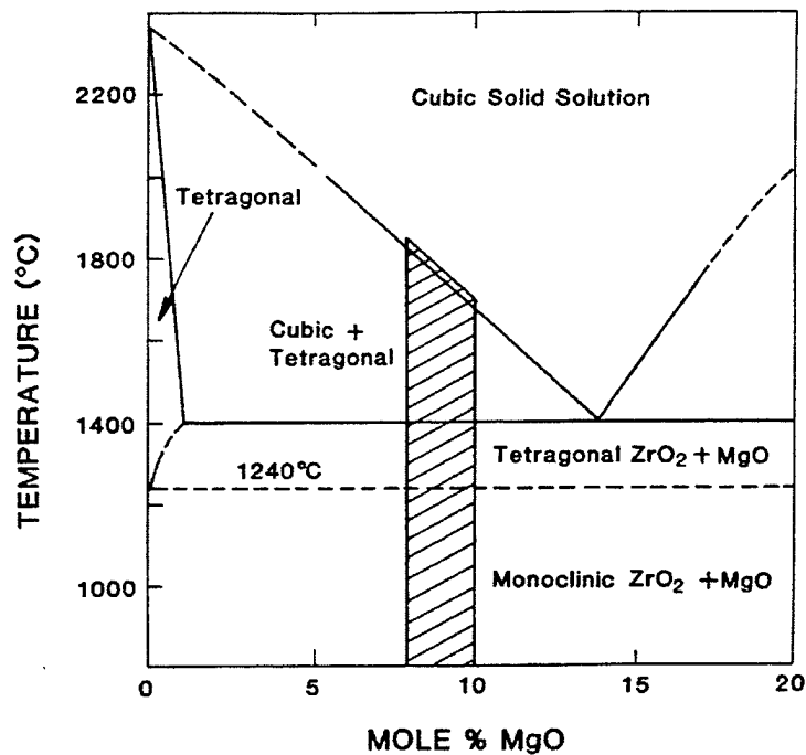
Figure 1. ZrO 2 -Rich End of the MgO-ZrO 2 Phase Diagram [6].
