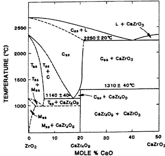
Figure 2. ZrO_2 -CaO Phase Diagram [22].
