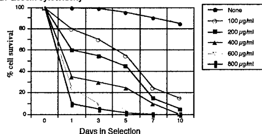
Figure 3. MCF-10A cell survival curves in the presence of selective agents.
