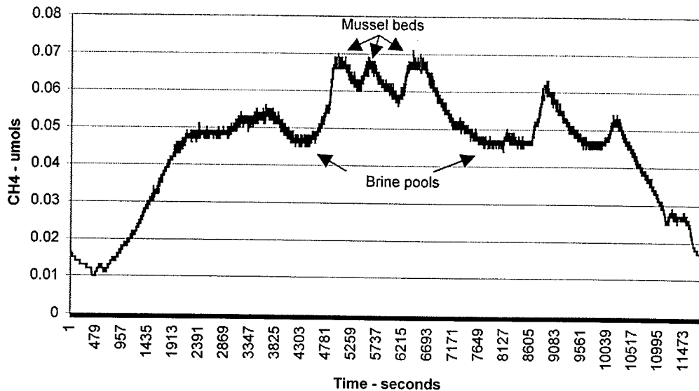
Figure 10. An example of low methane concentrations with strong local variability.
