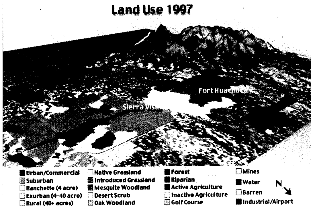
Figure 11. Sierra Vista land use classification 1997, looking southwest.
