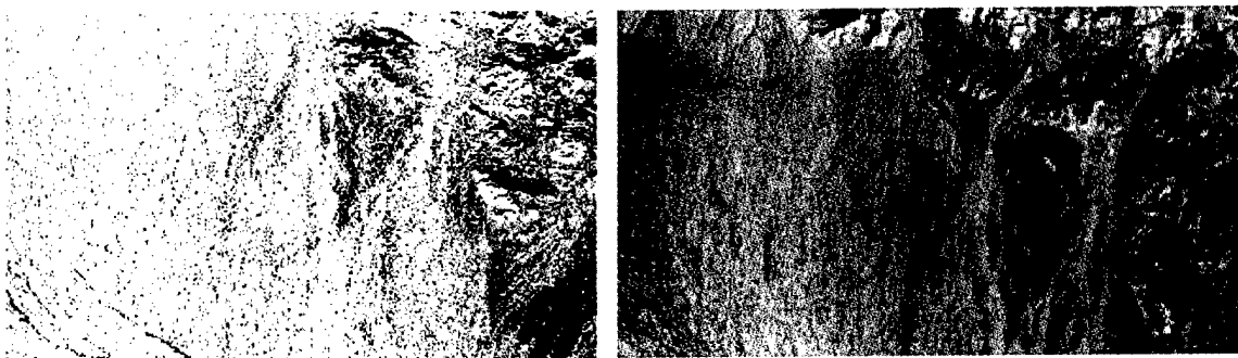
Figure 48. Corona image (left) dark areas with spotting and Landsat TM (right, Bands 4,3,2).
