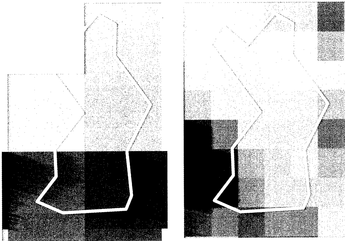
Figure 28. TM (left) and Corona (right): pixel samples (small area – 246.5 meters).
