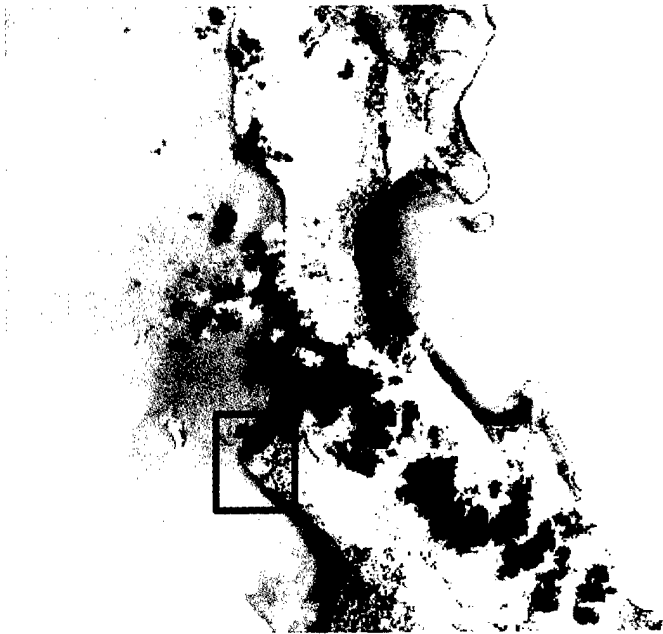
Figure 89. Ko Yao Yai Island, Thailand and the location used in the stereo pair application to show 3-D effects.
