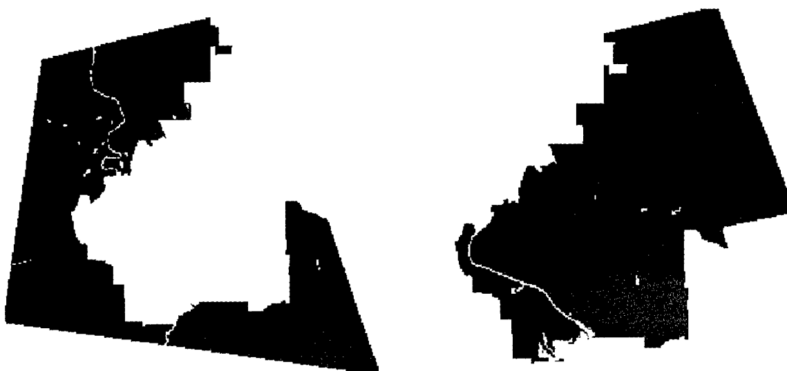
Figure 63. Outside (left) vs inside (right) the Fort Benning boundary based on the Landsat TM image and coordinated with the Corona image.
