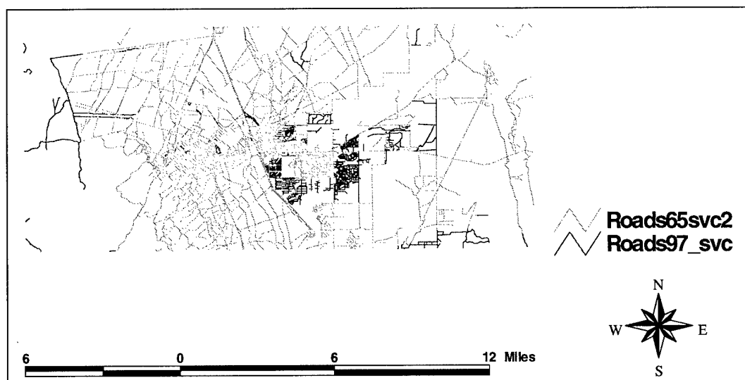
Figure 7. Increase in roads between 1965 and 1991.
