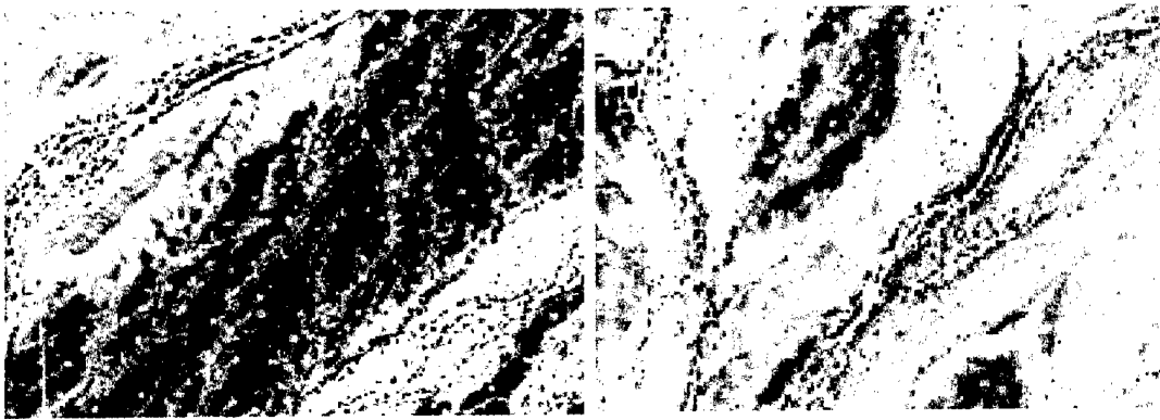
Figure 47. Spotting example (white spots) and vegetation example (black spots).
