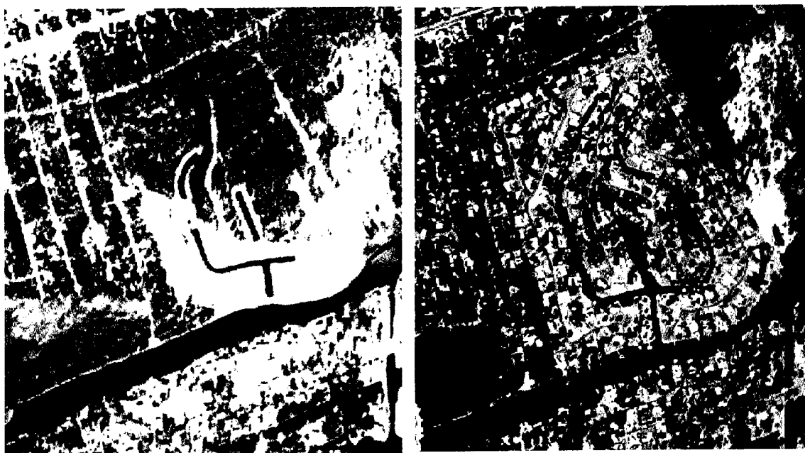
Figure 22. Development areas outside military lands.
