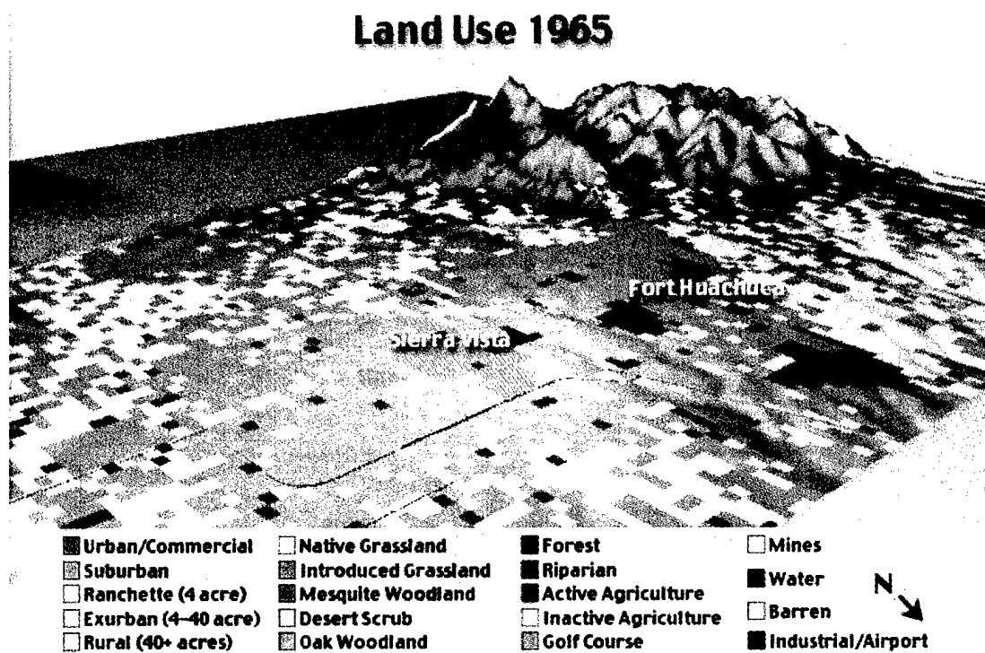
Figure 10. Sierra Vista land use classification 1965, looking southwest.
