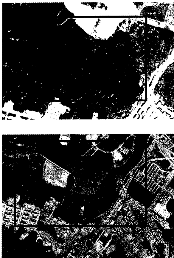
Figure 39. Comparison location, Corona image (top) and DOQQ (bottom).
