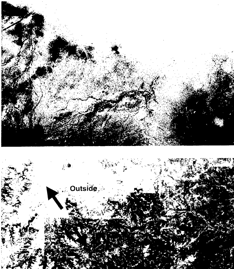
Figure 67. Manmade boundaries: 1964 Corona (top) image and 1989 SPOT (bottom) image.
