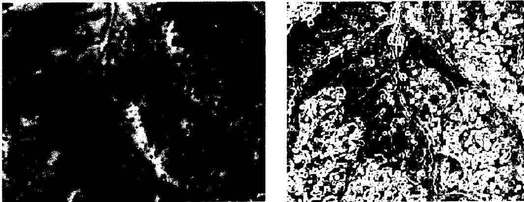
Figure 66. Plateau and slope identification.
