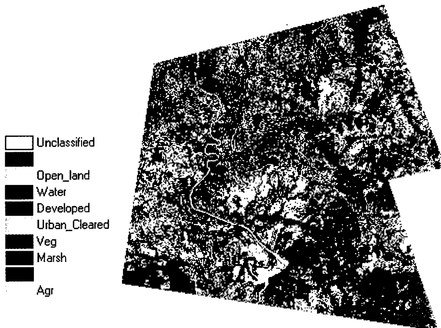
Figure 58. Supervised classification of Landsat TM image (10 classes).
