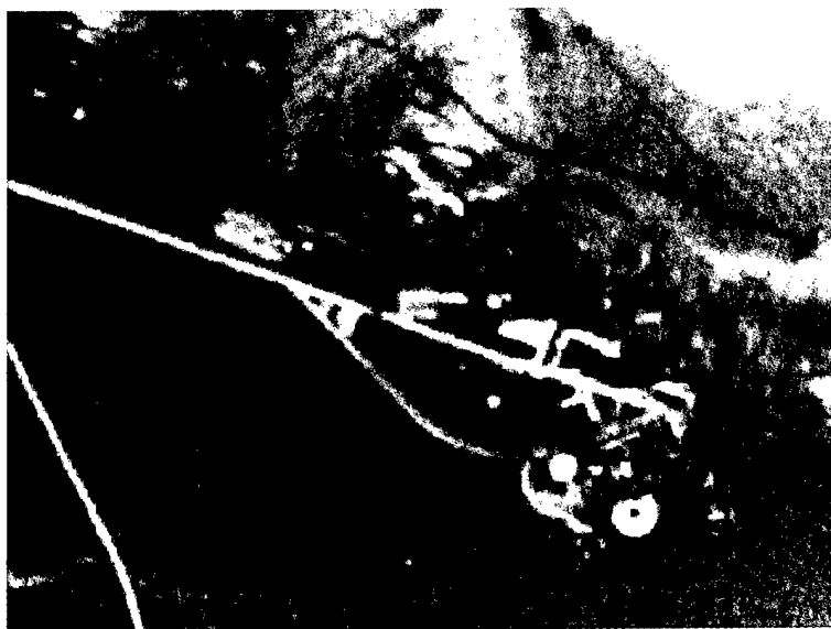
Figure 87. Corona images can be used to find old storage locations (lower right) or old range firing locations (upper right) at installations.
