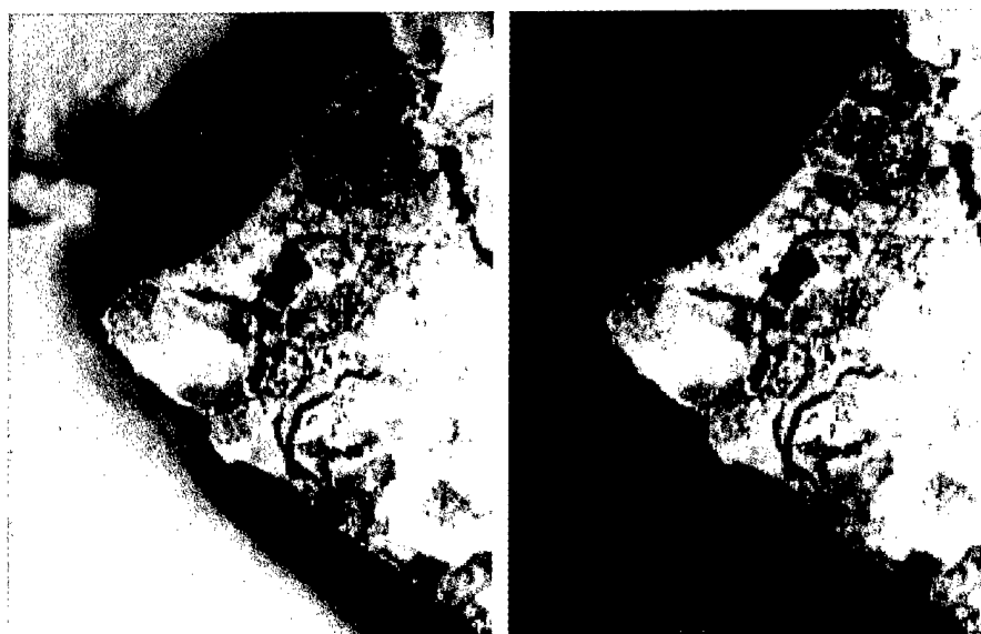
Figure 78. Stereo pair (forward image at left, aft image at right) showing 3-D effects at cliff face and on individual trees near arrow on Ko Yao Yai Island.
