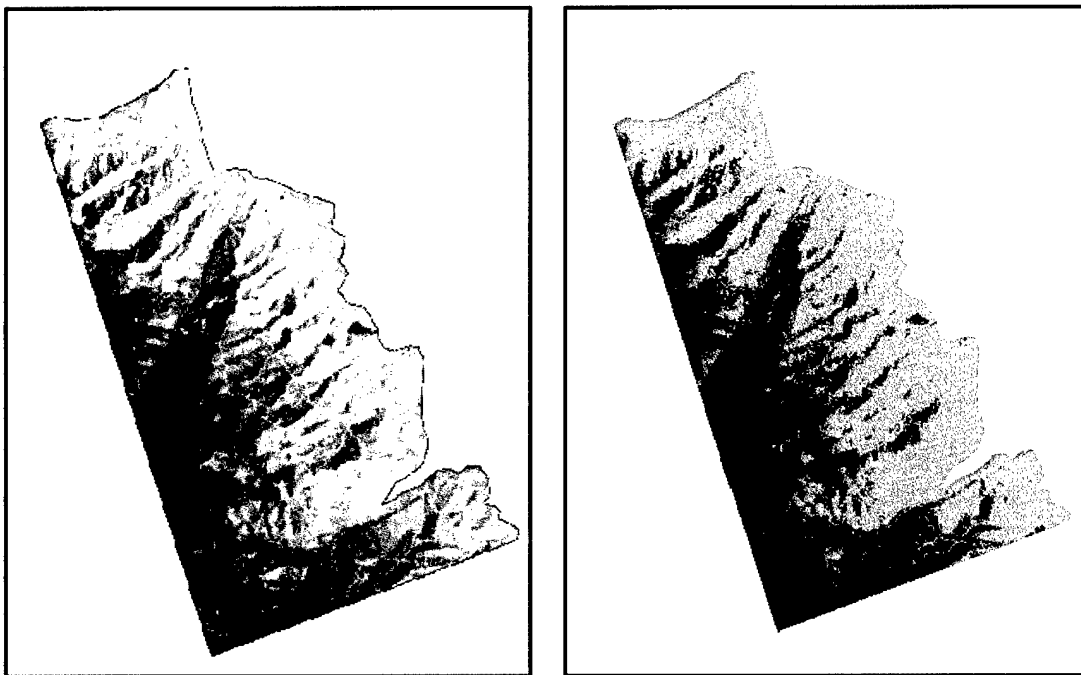
Figure 73. Landsat TM image classified by supervised classification (left) depicting forested area (highlighted, right).
