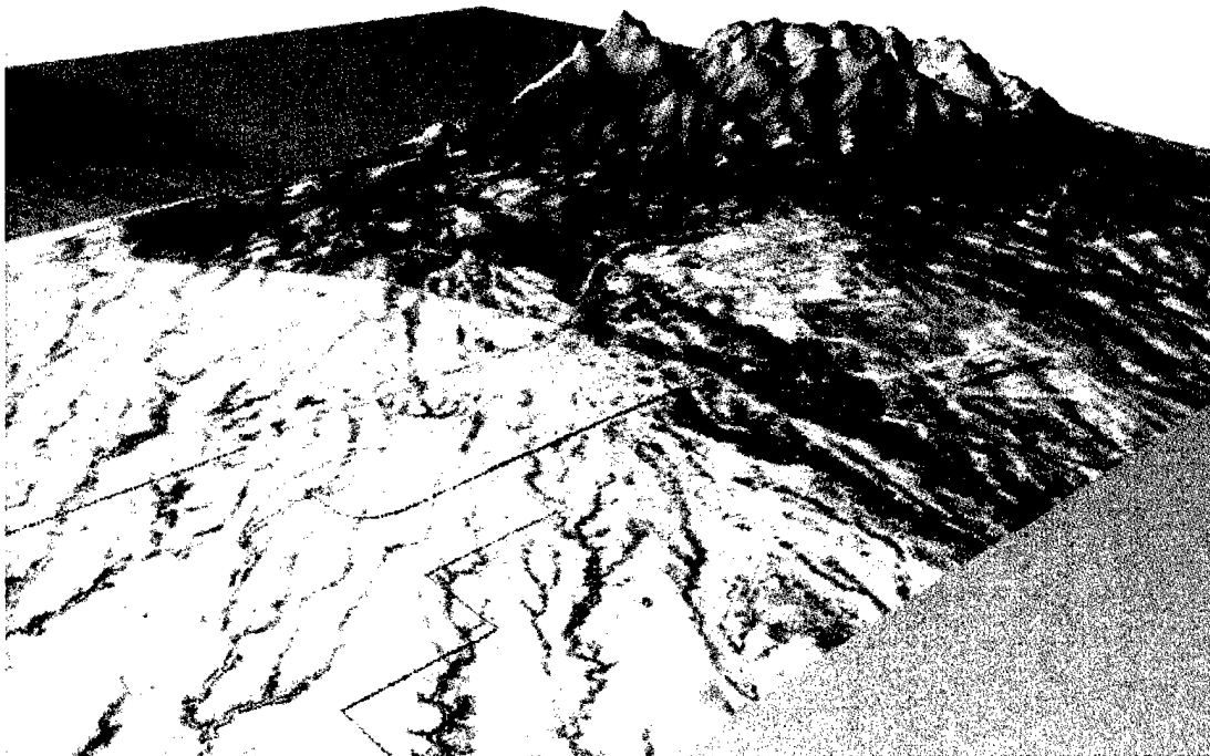
Figure 9. Simulated view of Sierra Vista 1965, looking southwest.
