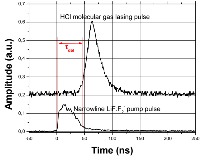
Fig. 4. 9 Oscillograms of narrowline LiF:F 2 - pump and P(5) HCl (3-2) molecular gas oscillating pulses.
