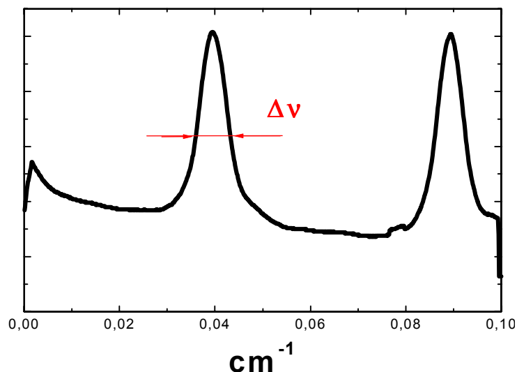
Fig. 4. 3 Oscillation linewidth of the narrowline \text{LiF:F}_2^- laser measured by Fizo interferometer and CCD array.
