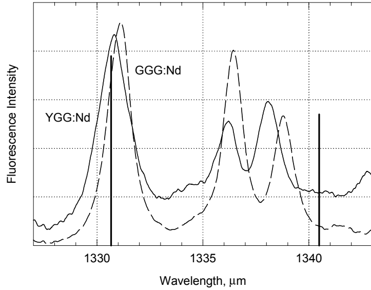
Fig. 2. 10 Fluorescence spectrum of {}^4F_{3/2} \rightarrow {}^4I_{13/2} transition in \text{Nd}^{3+}:\text{GGG} (dashed line) and \text{Nd}^{3+}:\text{YGG} (solid line) crystals at room temperature and P(4) absorption line of \text{HF}(2 \leftarrow 0) transition.
