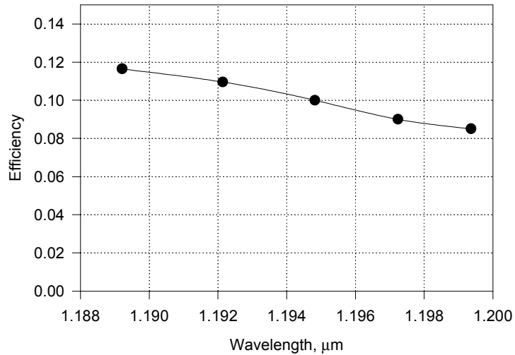
fig. 3. 3 Tuning curve of the \text{LiF:F}_2^- color center laser within 1.19\text{-}1.20\ \mu\text{m} wavelength range.
