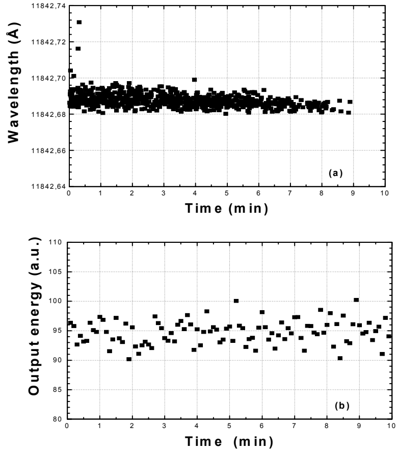
Fig. 4. 2 Spectral (a) and amplitude stability (b) of the narrowline \text{LiF:F}_2^- laser.
