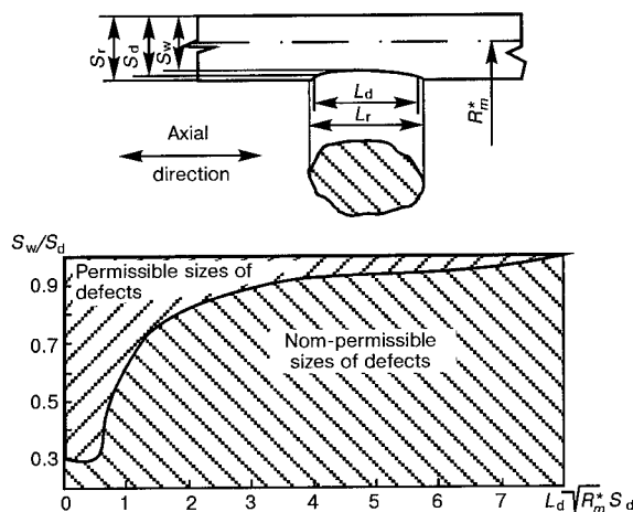
Figure 1. Diagram of maximum permissible sizes of the damaged zone versus erosion-corrosion wear of piping ( S_w , S_d and S_w — rated, design and wear zone thickness of the pipe wall, respectively; L_r and L_d — length of the wear zone corresponding to the rated and design wall thickness, respectively; R_m^* — mean radius of the pipe in the wear zones)
