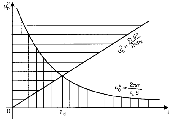
Figure 2. Regions of stability in accordance with inequalities (7)
