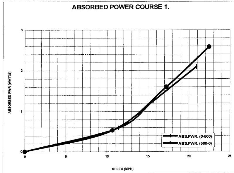
Figure 9. Absorbed power plot for Course 1
