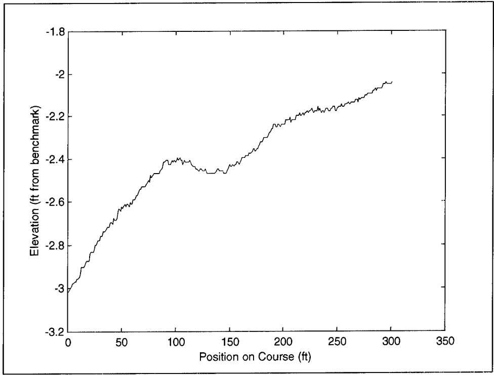
Figure A1. Elevation profile of LeTourneau Ride Course
