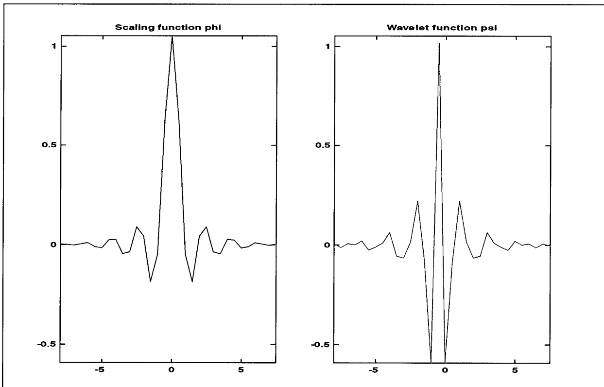
Figure 4. Meyer wavelets
