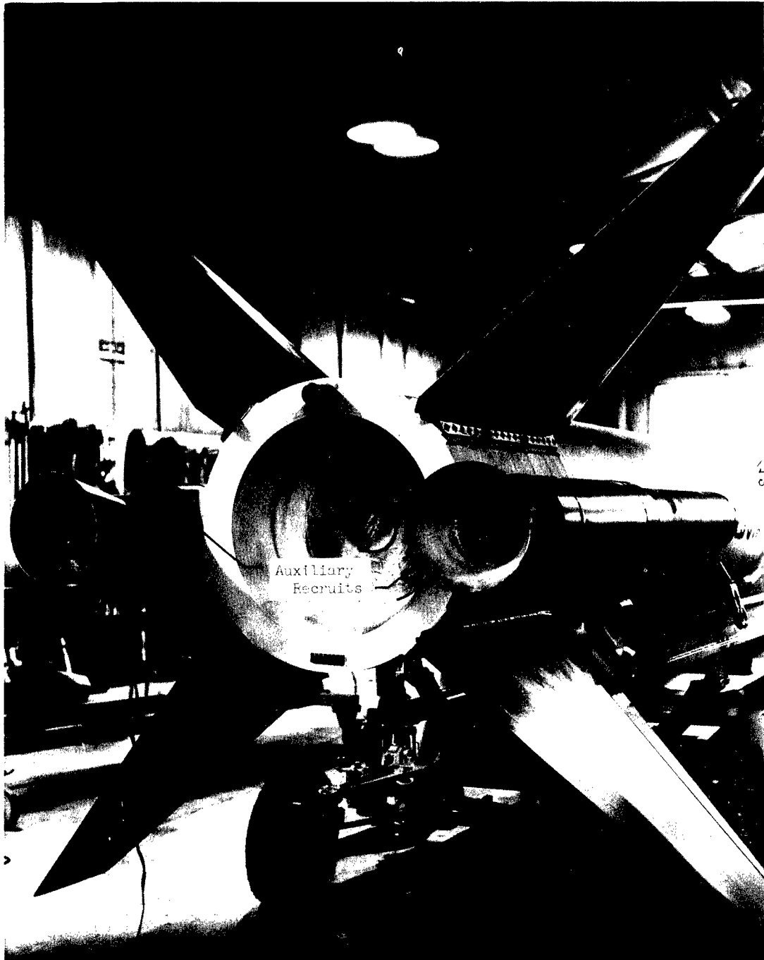
Figure 4.- End view of first stage showing two auxiliary Recruit motors attached to fin-shroud assembly.
