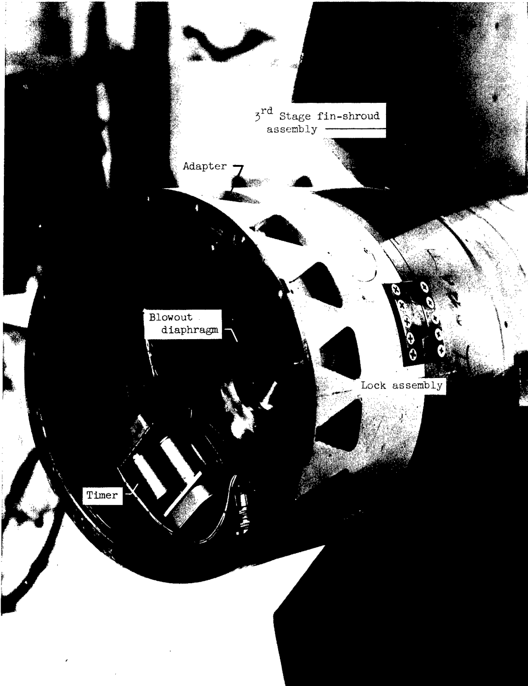
(d) Photograph of second- to third-stage assembly. I-62-1429.1
