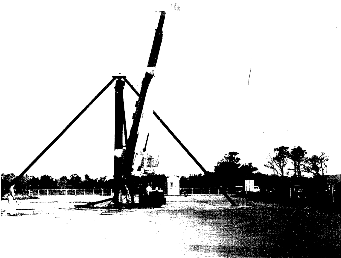
Figure 2.- Photograph of payload stage and booster system in launch position. L-61-6238
