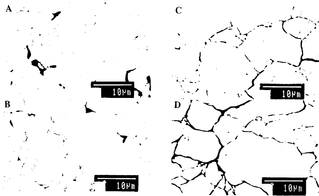
Figure 8. BSE-COMP micrographs of the core regions of W-Ti alloys fabricated from Ti-coated W powder: (a) 0.19 Ti atomic-percent, (b) 0.50 Ti atomic-percent, (c) 1.14 Ti atomic-percent, and (d) 2.67 atomic-percent Ti.
