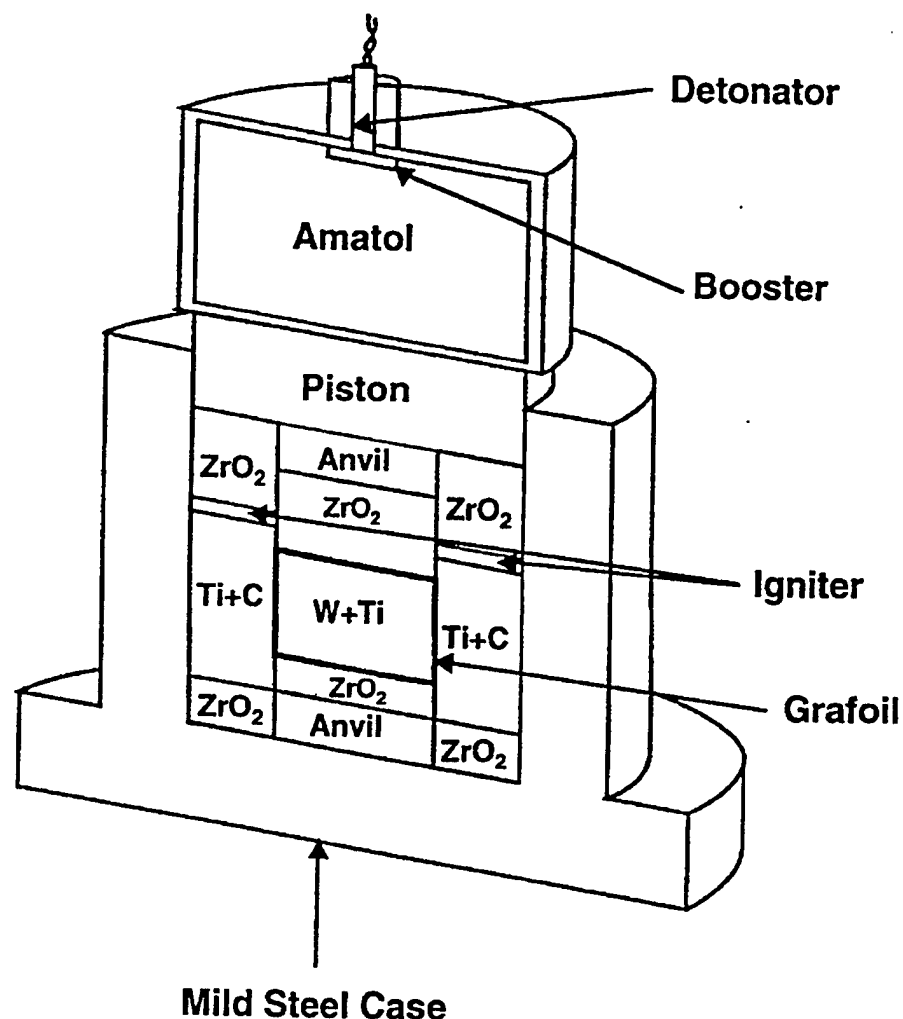
Figure 1(a). CSA-HEC method: (a) schematic diagram of the apparatus.
