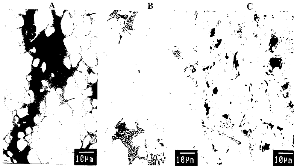
Figure A-2. BSE-COMP micrographs of polished surfaces of a typical 83W-17Ti billet. Core region is shown in (a), transition region is shown in (b), and edge region is shown in (c).
