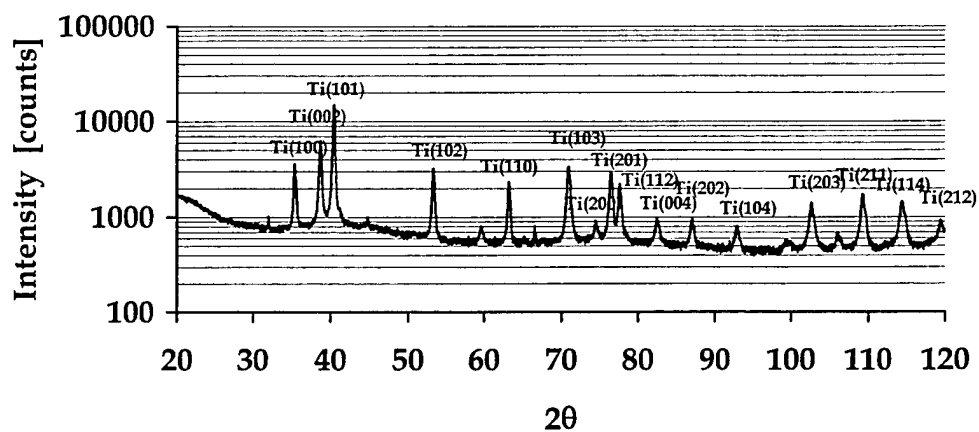
(f) Unalloyed Ti
