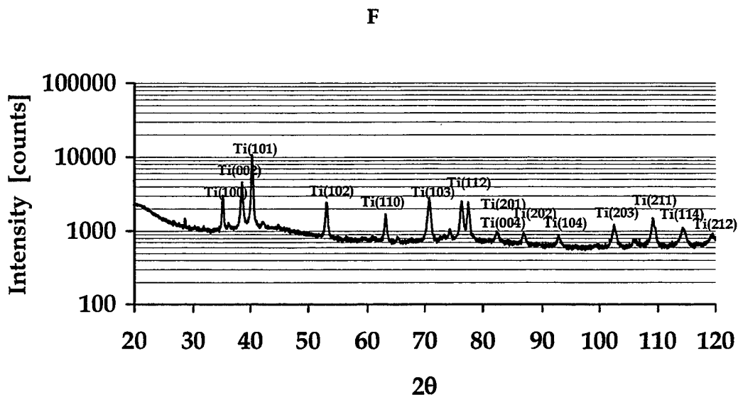
(f) unalloyed Ti
