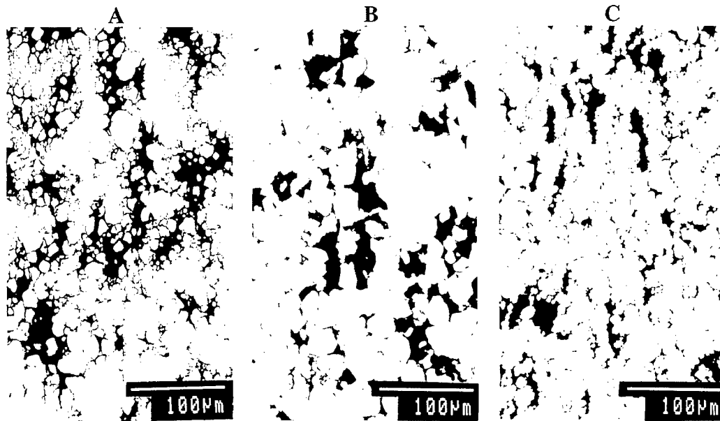
Figure 3. BSE-COMP micrographs of core regions of the 83W-17Ti alloys: (a) standard, (b) coarse, and (c) fine.
