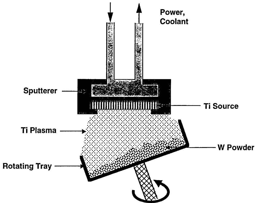
Figure 2. Schematic diagram of the PVD/DC sputtering system that was used to fabricate the Ti-coated W powder.
