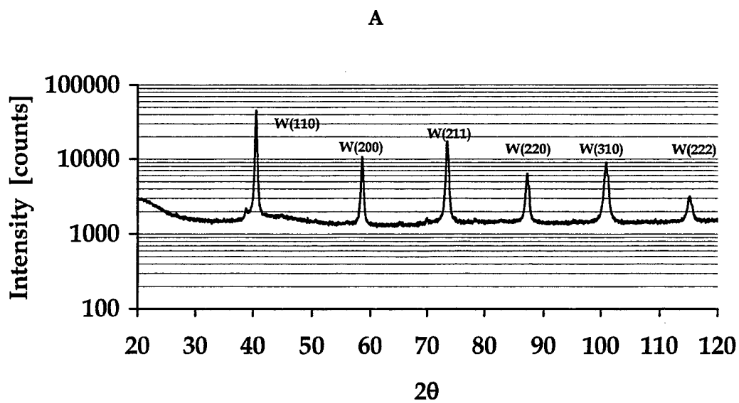
(a) unalloyed W
