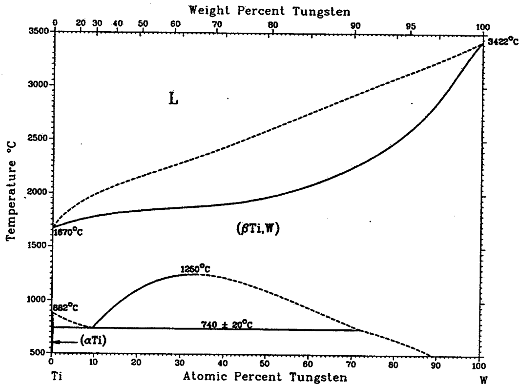
Figure 7. W-Ti equilibrium phase diagram.
