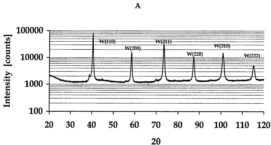
(a) Unalloyed W
