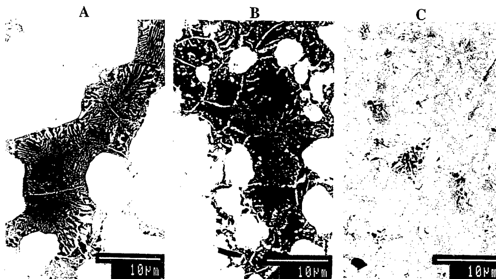
Figure 9. BSE-COMP micrographs of substructures forming during annealing: (a) 700 °C, (b) 1,000 °C, and (c) 1,400 °C.
