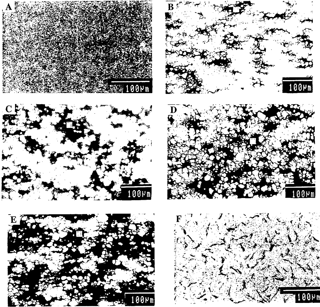
Figure 4. BSE-COMP micrographs of the alloys: (a) unalloyed W, (b) 83W-17Ti, (c) 70W-30Ti, (d) 60W-40Ti, (e) 51W-49Ti, and (f) unalloyed Ti.
