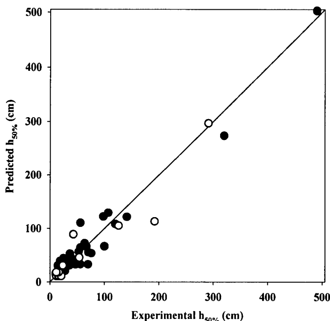
Figure 24. Predicted Versus Experimental h_{50\%} Values for Explosives (solid circles denote 34 explosives whose values were measured by Wilson et al. [42], and hollow circles denote 11 molecules used to assess the predictive quality of the model; solid line denotes exact agreement) .
