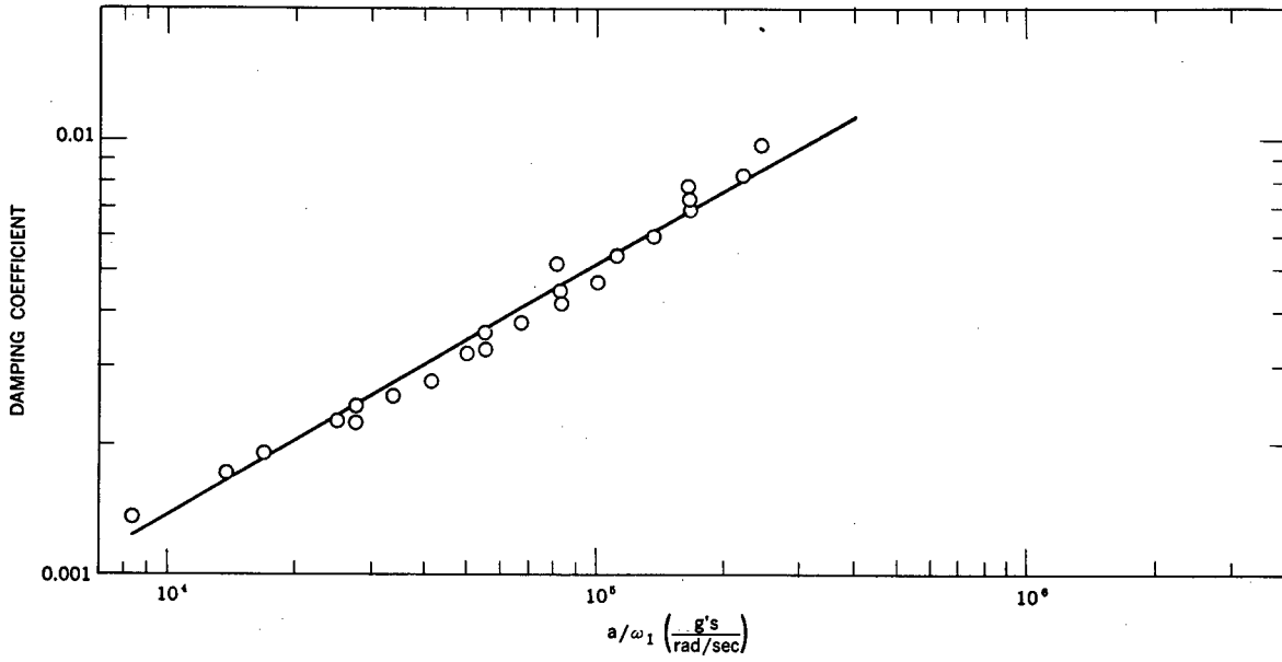
Figure 7—Attempt to correlate damping data for cold-rolled C1018 steel according to Equation 47
