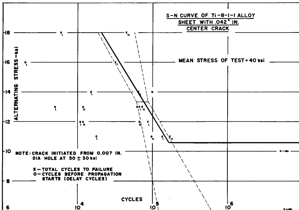
Figure 13. S-N Curve of Ti 8-1-1 alloy sheet with 0.042 in. center crack, 40 ksi mean stress.
