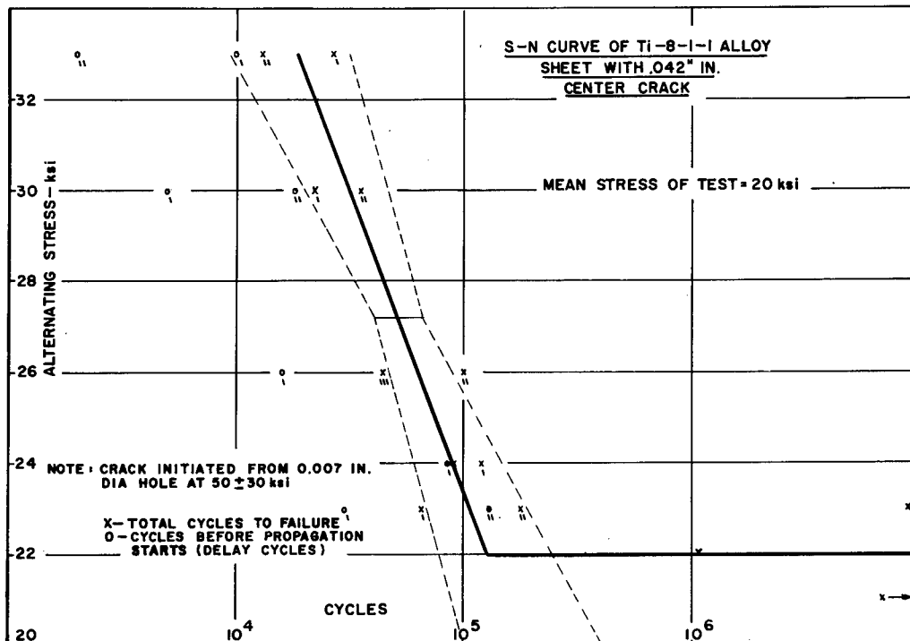
Figure 12. S-N Curve of Ti 8-1-1 alloy sheet with 0.042 in. center crack, 20 ksi mean stress.
