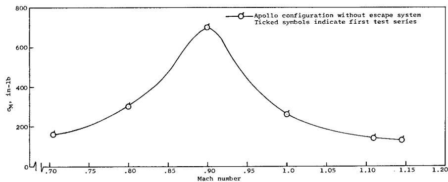
(b) Apollo configuration without escape system.
