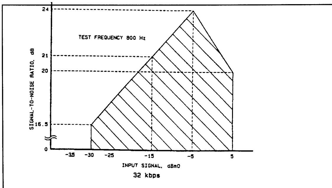
Figure F-6b. Signal to quantizing noise ratio versus input level for CVSD (32 kbps).
