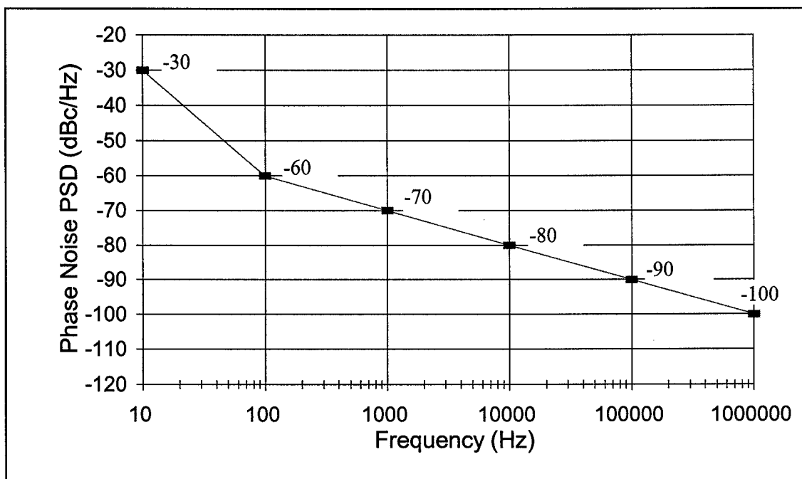
Figure 2-1. Continuous single sideband phase noise power spectral density.
