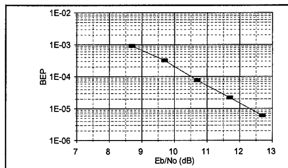
Figure A-17. FQPSK-B BEP vs E_b/N_0 .
