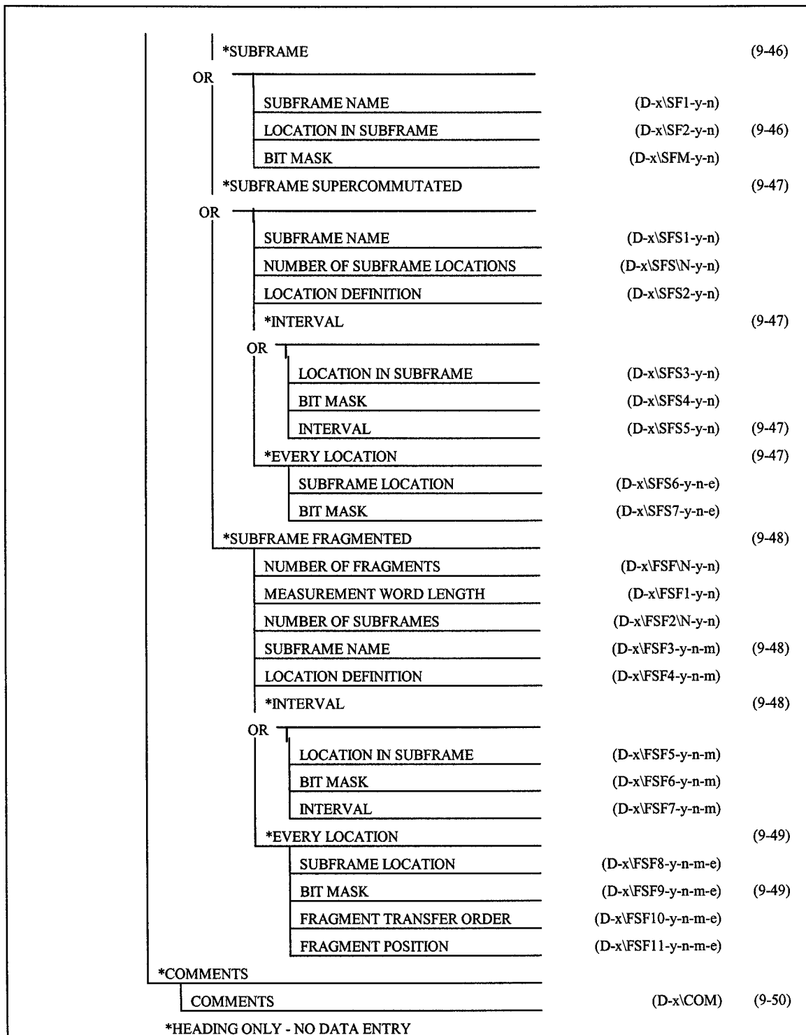
Figure 9-7 (Cont'd). PCM Measurement Description Group (D).
