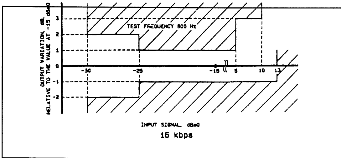
Figure F-5a. Variation of gain with input level for CVSD (16 kbps).
