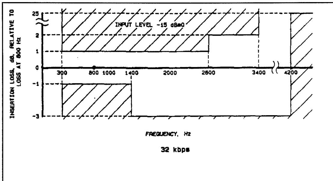
Figure F-4b. Insertion loss versus frequency for CVSD (32 kbps).
