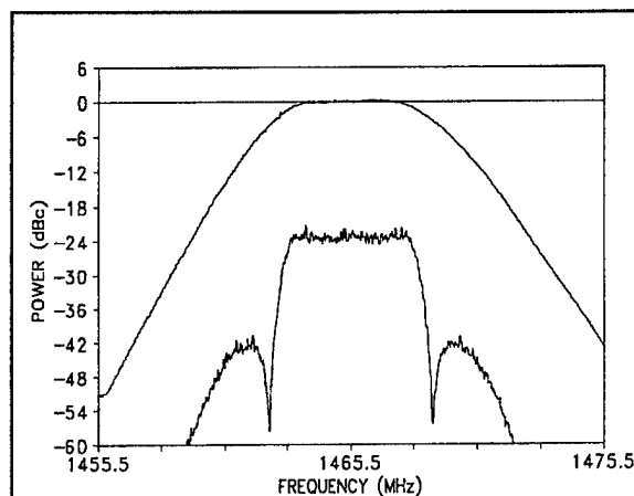
Figure A-3. Spectrum analyzer calibration of 0-dBc level.
