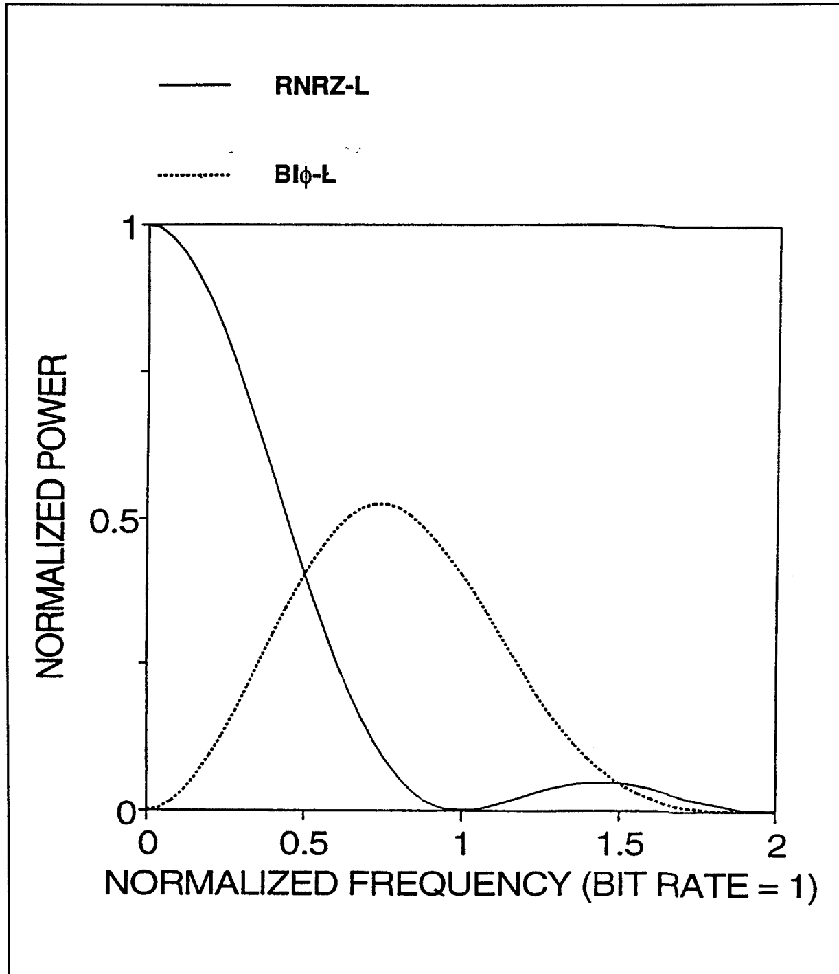
Figure D-4. Random PCM power spectra.
