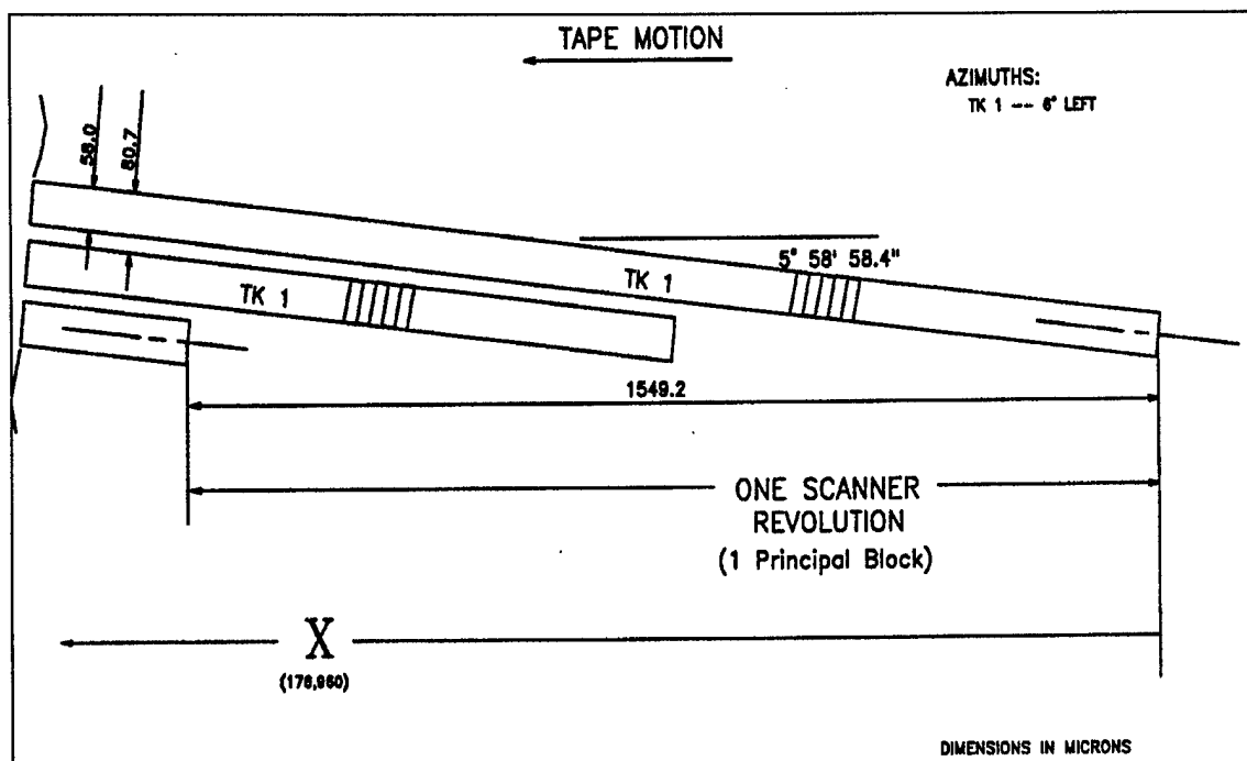
Figure 6-11. Helical track dimensions, E format.
