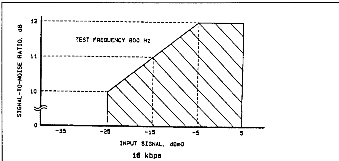
Figure F-6a. Signal to quantizing noise ratio versus input level for CVSD (16 kbps).
