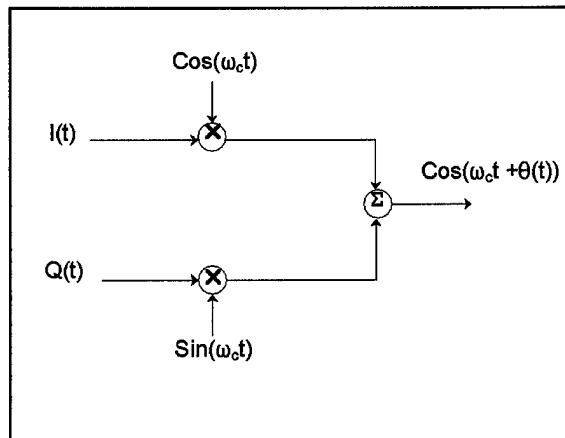
Figure A-10. OQPSK modulator.
