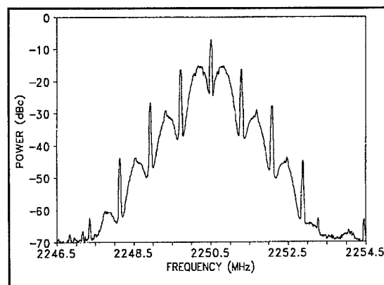
Figure A-4. Biφ PCM/PM signal.
