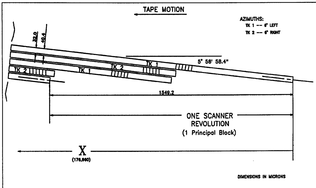
Figure 6-10. Helical track dimensions, B format.
