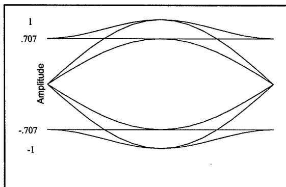
Figure A-12. FQPSK-B wavelets.
