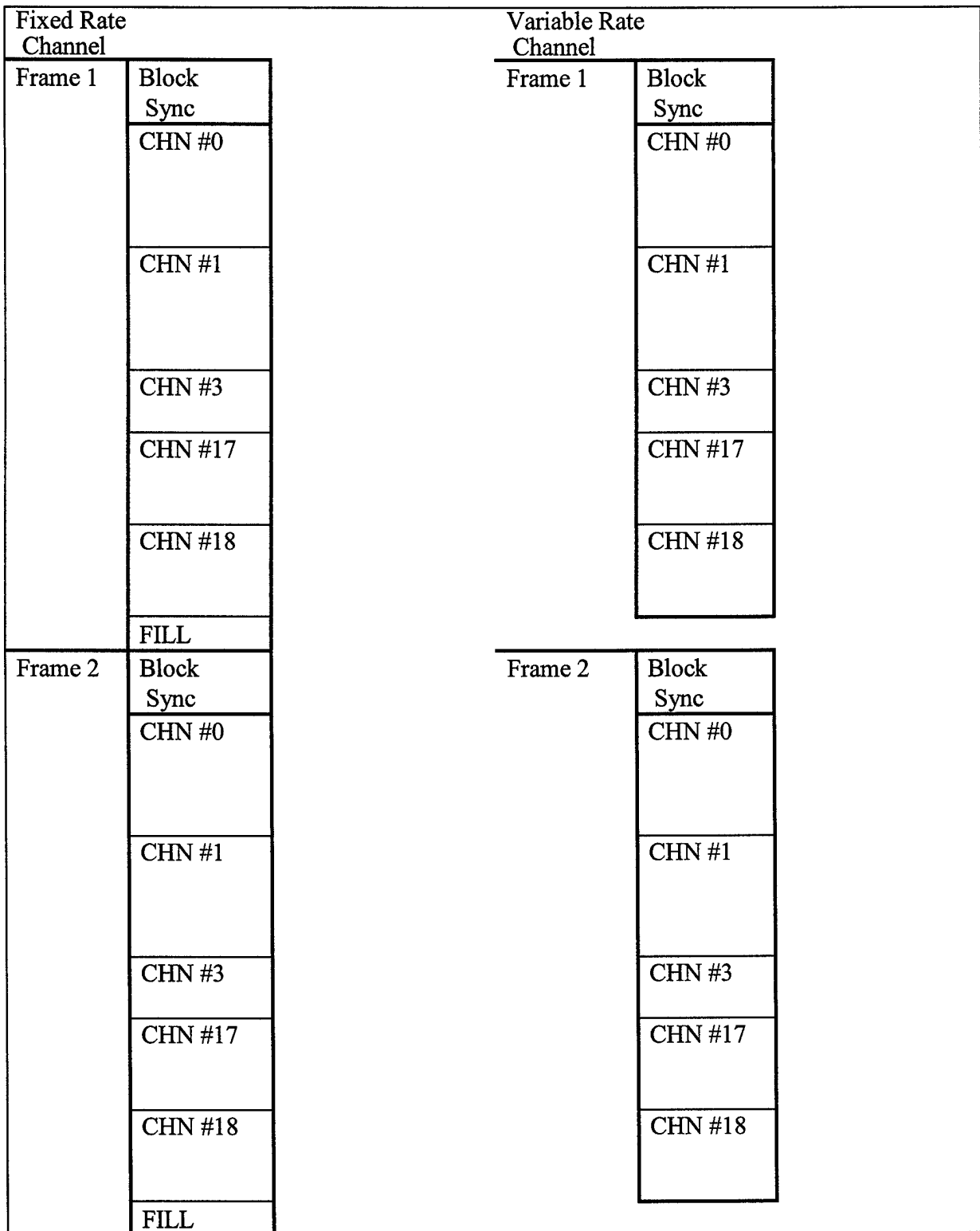
Figure G-5. Submux aggregate format.
