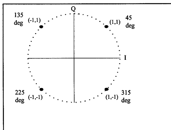
Figure A-11. I & Q constellation.
