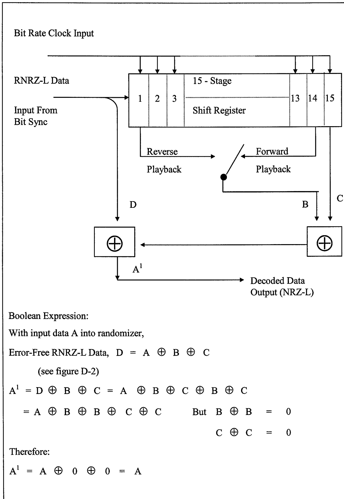
Figure D-3. Randomized NRZ-L decoder block diagram.
