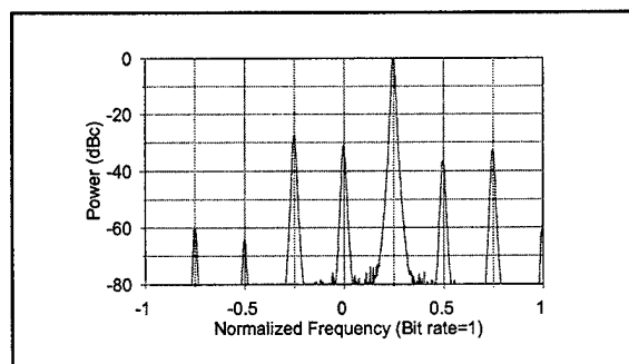
Figure A-16. FQPSK-B spectrum with all 1’s input and large modulator errors.
