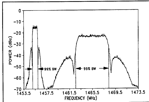
Figure A-1. 800-kb/s and 5-Mb/s RNRZ PCM/FM signals.
