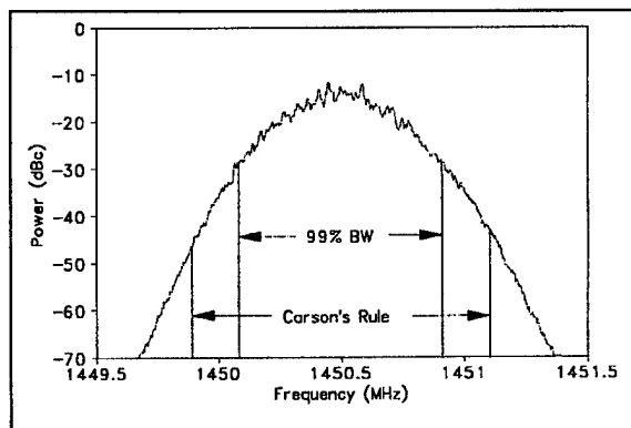
Figure A-5. FM/FM signal and Carson's Rule.
