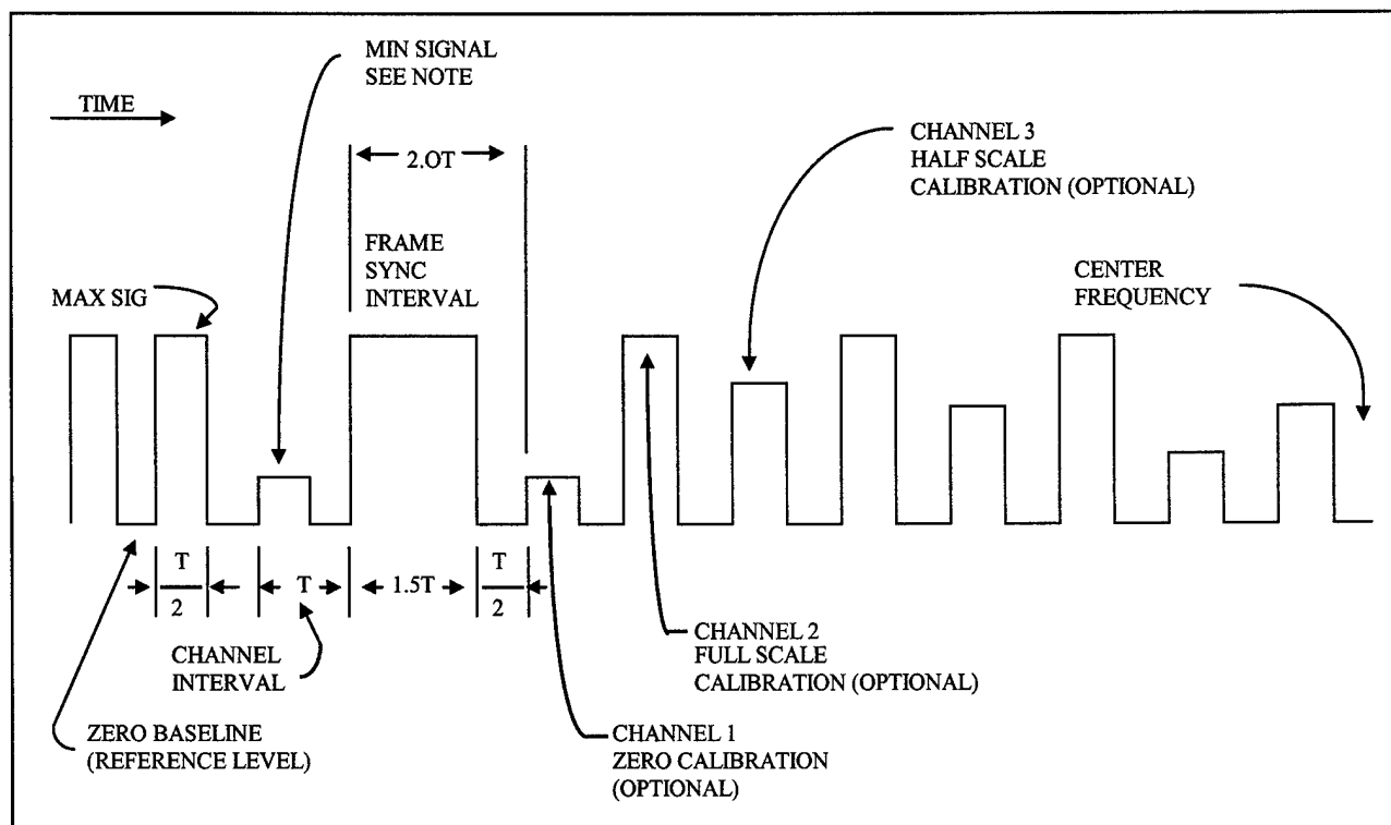
Figure K-1. 50-percent duty cycle PAM with amplitude synchronization.
