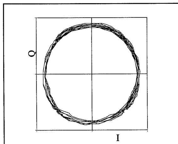
Figure A-14. FQPSK-B vector diagram.
