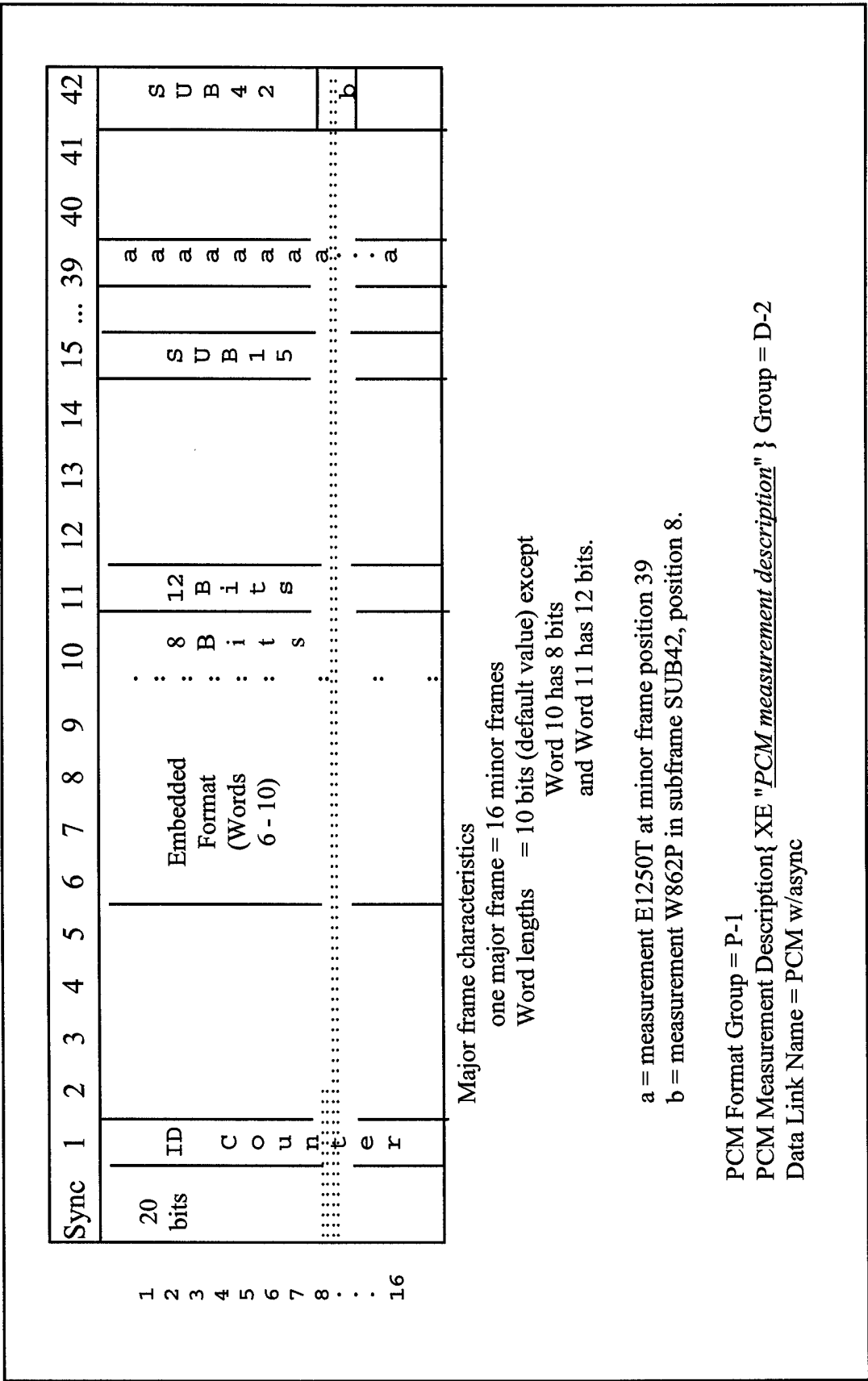
Figure J-2. PCM format for PCM w/async.
