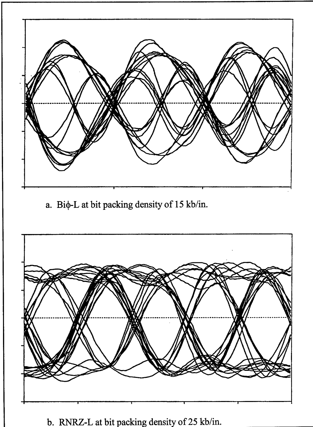
Figure D-5. Sample eye patterns at output of recorder/reproducer.
