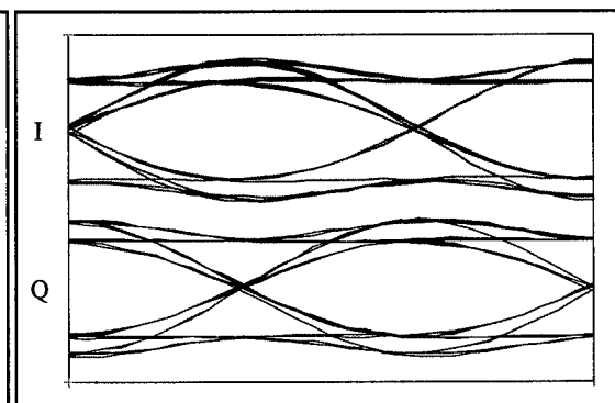
Figure A-13. FQPSK-B I & Q eye diagrams (at input to IQ modulator).
