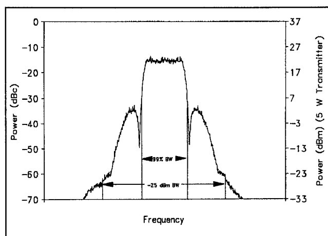
Figure A-2. RNRZ PCM/FM signal.
