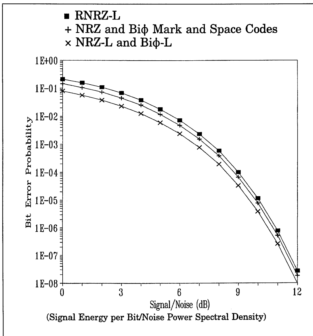
Figure C-3. Theoretical bit error probability performance for various baseband PCM signaling techniques (perfect bit synchronization assumed).
