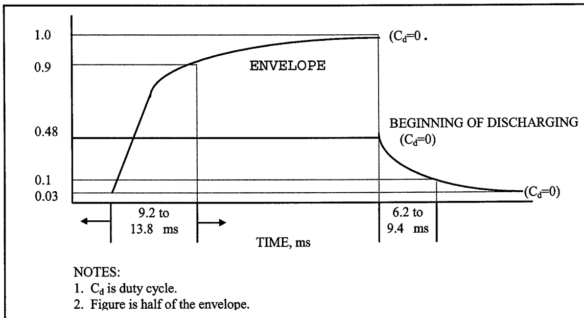
Figure F-2. Typical envelope characteristics of the decoder output signal for CVSD.
