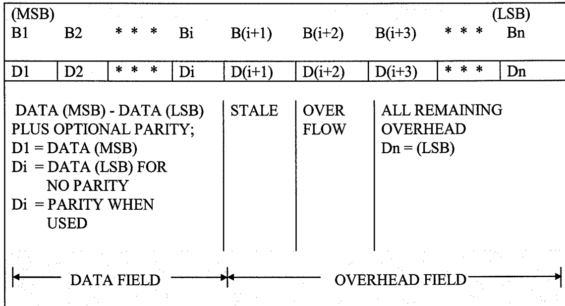
Figure 4-5. Asynchronous word structure
