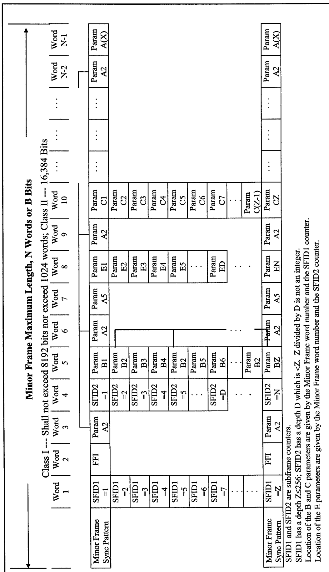
Figure C-6. Major Frame Length = Minor Frame Maximum Length multiplied by Z.
