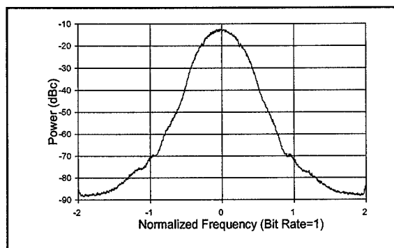
Figure A-15. FQPSK-B spectrum with random input data.
