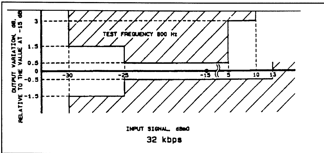
Figure F-5b. Variation of gain with input level for CVSD (32 kbps).
