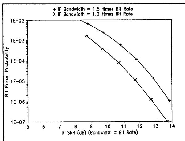
Figure C-1. BEP versus IF SNR in bandwidth = bit rate for NRZ-L PCM/FM.
