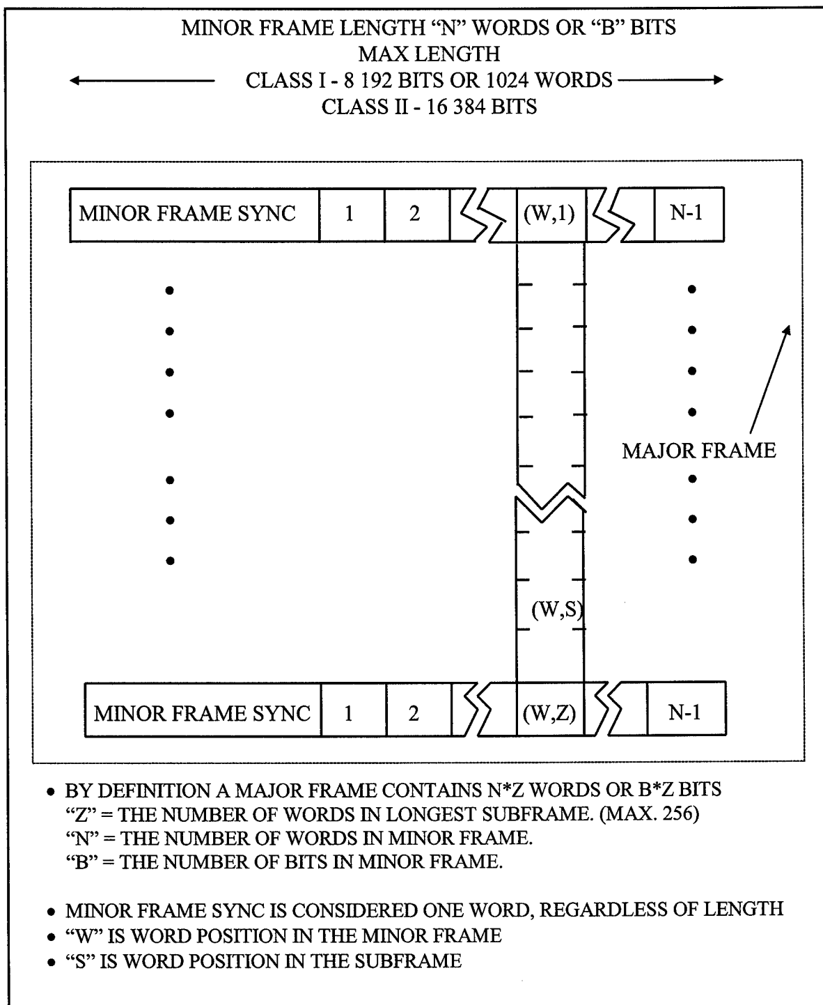
Figure 4-2. PCM frame structure.
