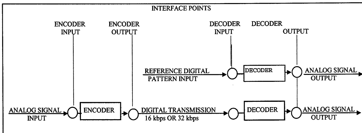
Figure F-3. Interface diagram for CVSD converter.
