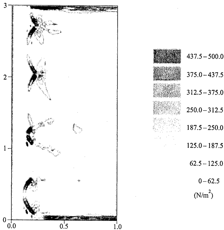
Figure 4 Distribution of shear stress \tau_{yx} (= \tau_{xy}) 565 \mu\text{s} after ignition for Case 1 in Table 2. Dimensions in cm
