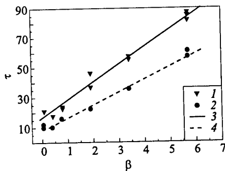
Figure 9 \tau_{TW}^+ and \tau_{tot} vs. \beta when using cylindrical nozzles: 1 — \tau_{tot} , 2 — \tau_{TW}^+ , 3 — fit ( \tau_{tot} ), 4 — fit ( \tau_{TW}^+ )
