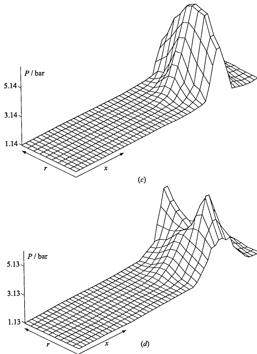
Figure 5 Predicted temporal development of pressure distribution in the combustion chamber: (a) t = t_d + 4 \mu\text{s} ; (b) t = t_d + 10 \mu\text{s} ; (c) t = t_d + 12 \mu\text{s} ; (d) t = t_d + 20 \mu\text{s} ; t_d is the discharge time, r and x are the cylindrical coordinates (Continued)
