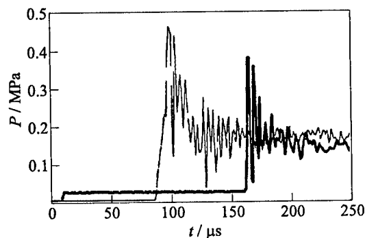
Figure 7 Pressure records for the case presented in Fig. 6 ( M = 2.65 )
