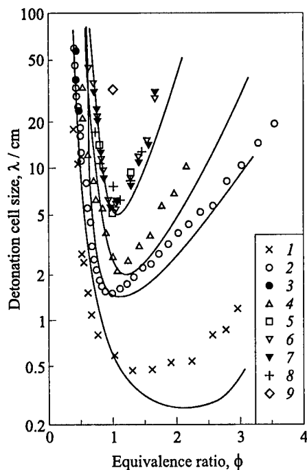
Figure 11 Variation of detonation cell size vs. equivalence ratio for different fuel-air compositions [29]: 1 — C_2H_2 , 2, 3 — H_2 , 4 — C_2H_4 , 5 — C_2H_6 , 6, 7 — C_3H_8 , 8 — C_4H_{10} , 9 — CH_4 (open symbols correspond to smoked foil measurements, filled symbols — to pressure oscillation measurements). Solid curves correspond to the model \lambda = Al ( l is the induction length of the CJ detonation)
