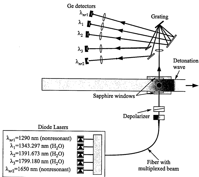
Figure 1 Five-wavelength tunable diode laser absorption diagnostics for measuring gas temperature and \text{H}_2\text{O} mole fraction
