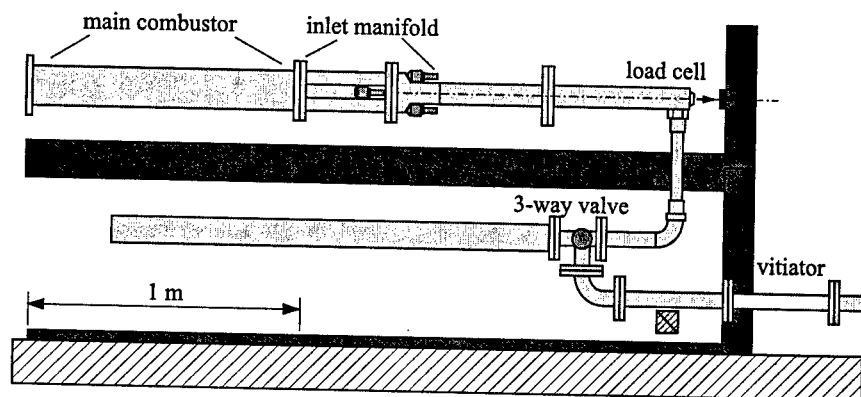
Figure 2 Experimental layout
