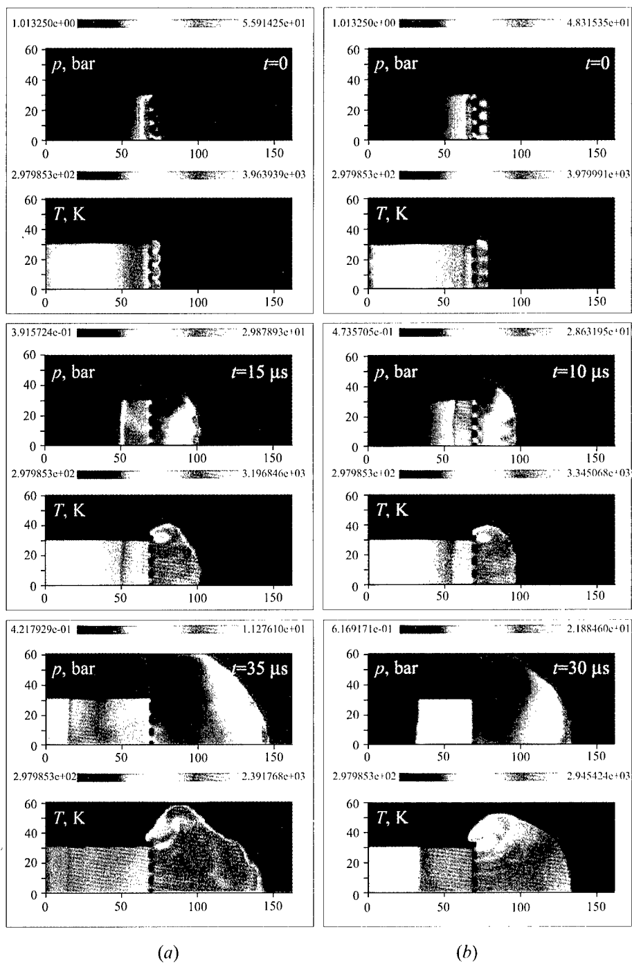
Figure 3 Pressure and temperature profiles from numerical computations showing detonation transmission and failure to transmit through a two-dimensional tube bundle. D_0=6 \text{ cm} , \alpha=0.57 , \gamma=1.4 , M_w = 28.8 \text{ g/mole} , Q=1.445 \text{ MJ/kg} , E = 4.30 \text{ MJ/kg} , computational cell = 1 \times 1 \text{ mm} . (a) k = 6 \times 10^8 \text{ s}^{-1} (failure). (b) k = 3 \times 10^9 \text{ s}^{-1} (successful transmission). (Refer p. 147)
