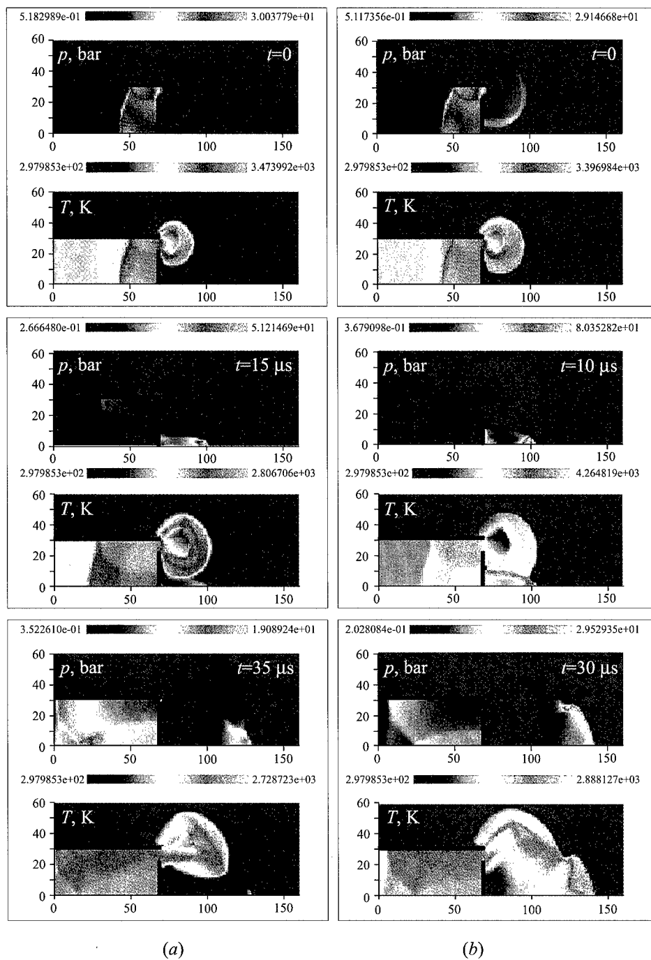
Figure 2 Pressure and temperature profiles from numerical computations showing detonation transmission and failure to transmit through an annular orifice. D_0=6 cm, \alpha=0.44 , \gamma=1.4 , M_w = 28.8 g/mole, Q=1.445 MJ/kg, E = 4.30 MJ/kg, computational cell = 1 \times 1 mm. (a) k=6 \times 10^8 \text{ s}^{-1} (failure). (b) k=3 \times 10^9 \text{ s}^{-1} (successful transmission). (Refer p. 145)
