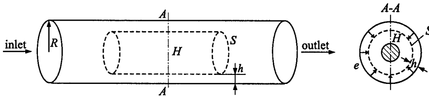
Figure 7 Schematic of the implosion process in the combustion chamber. S is the electrode surface. A-A is the chamber sectional view; e is the electrode, h is the height of electrodes ( h \approx 0.1R ); H is the high-pressure zone due to implosion
