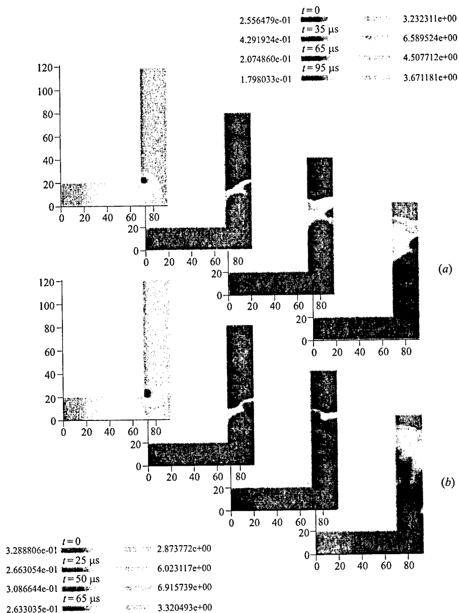
Figure 4 Density profiles from numerical computations showing detonation transmission and failure to transmit to a cylindrical gap. D_0 = 4 \text{ cm} , w/D_0 = 0.6 , \gamma = 1.4 , M_w = 28.8 \text{ g/mole} , Q = 1.445 \text{ MJ/kg} , E = 4.30 \text{ MJ/kg} , computational cell = 1 \times 1 \text{ mm} . (a) k = 8 \times 10^8 \text{ s}^{-1} (failure); (b) k = 5 \times 10^9 \text{ s}^{-1} (successful transmission). (Refer color plate.)
