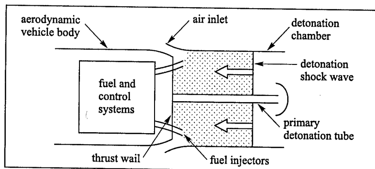
Figure 3 PDE device [13]
