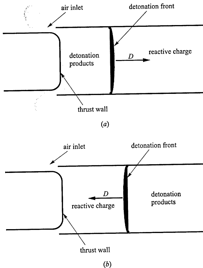
Figure 4 Schematic of the PDE basic setup: (a) detonation initiation at the thrust wall; (b) detonation initiation at the open end
