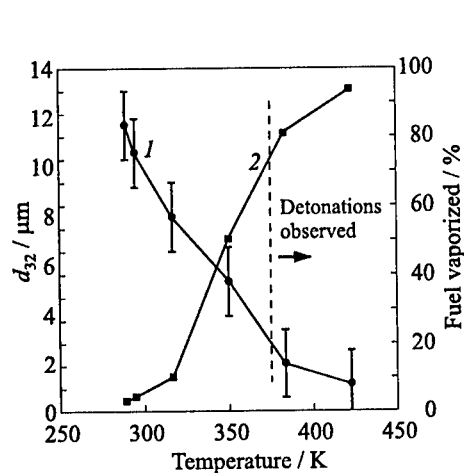
Figure 5 Sauter mean diameter 1 and percent of fuel vaporized 2 as functions of PDE inlet temperature. JP-10-air mixture, air flow rate 0.20 kg/s, fuel pressure 45 psig, air pressure 75 psig
