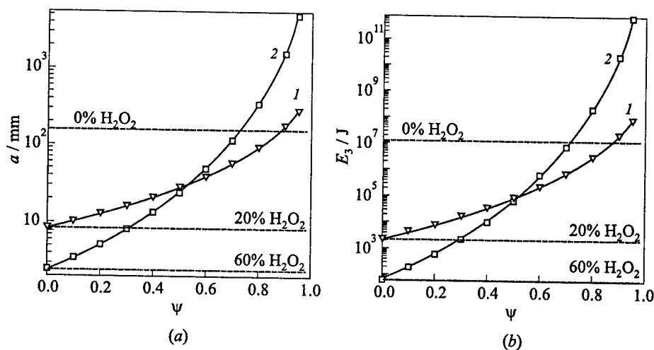
Figure 6 Detonation cell size ( a ) and critical initiation energy for spherical detonations ( b ) as a function of molar fraction of water \psi in the aqueous solution of HP for dual-fuel systems iso -octane – 20% HP (curves 1) and iso -octane – 60% HP (curves 2). Horizontal dashed lines '0% H_2O_2 ,' '20% H_2O_2 ,' and '60% H_2O_2 ' correspond to the cell sizes ( a ) and to E_3 ( b ) in the corresponding systems with \psi = 0
