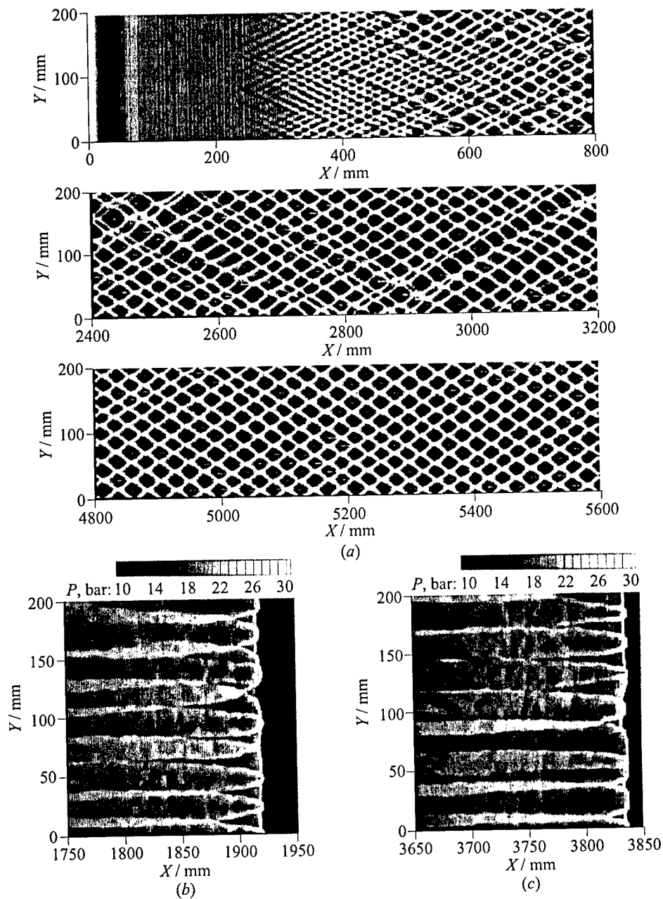
Figure 4 Tracks of maximum pressure (same pressure scales as in Fig. 1) (a) and pressure distribution in pure gaseous mixture at t = 1\text{ ms} (b) and t = 2\text{ ms} (c)
