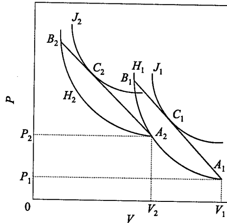
Figure 3 Hugoniot for different initial states of a combustible gas
