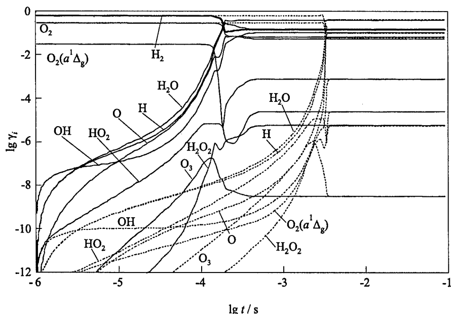
Figure 3 Predicted histories of species concentrations during combustion of the oxygen-hydrogen mixture with H_2/O_2 = 2/1 at P_0 = 10 kPa and T_0 = 800 K with preexcitation of O_2 molecules ( \gamma_{O_2(a^1\Delta_g)}/\gamma_{O_2} = 0.1 ), (solid curves), and without preexcitation (dashed curves)
