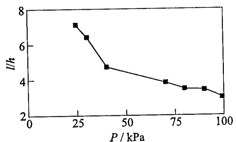
Figure 16 DDT distance vs. initial pressure at \xi_{N_2} = 22\%
