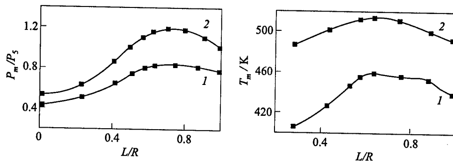
Figure 9 Maximum pressure (a) and temperature (b) vs. the hemicylindrical cavity depth: 1 — d = 2 mm and 2 — 4 mm. Dimensions of R and L are shown in Fig. 8a
