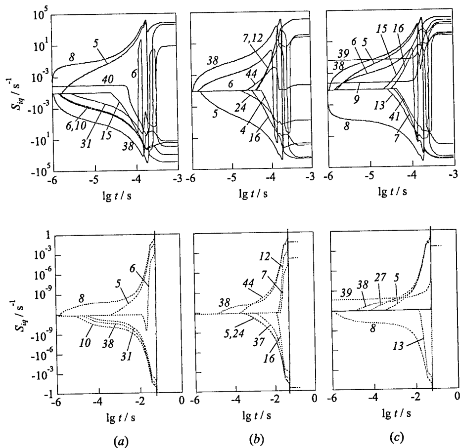
Figure 2 Histories of production (+) and destruction (-) rates S_{iq} for H (a), O (b), and OH (c) species during combustion of the oxygen-hydrogen mixture with H_2/O_2 = 2/1 at P_0 = 10 kPa with preexcitation of O_2 molecules ( \gamma_{O_2(a^1\Delta_g)}/\gamma_{O_2} = 0.1 ) at T_0 = 800 K (solid curves) and 400 K (dashed curves). Numbers denote the reaction numbers in Table 1
