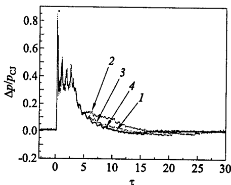
Figure 10 Thrust wall dimensionless overpressure-time records obtained with straight conical nozzles for \beta = 1 : 1 — \alpha = 180^\circ (reference signal); 2 — 0^\circ ; 3 — 5^\circ ; and 4 — 18^\circ
