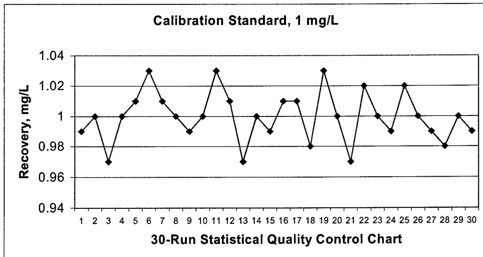
Figure E.6: Copper Instrumental Calibration Standard (ICS)
